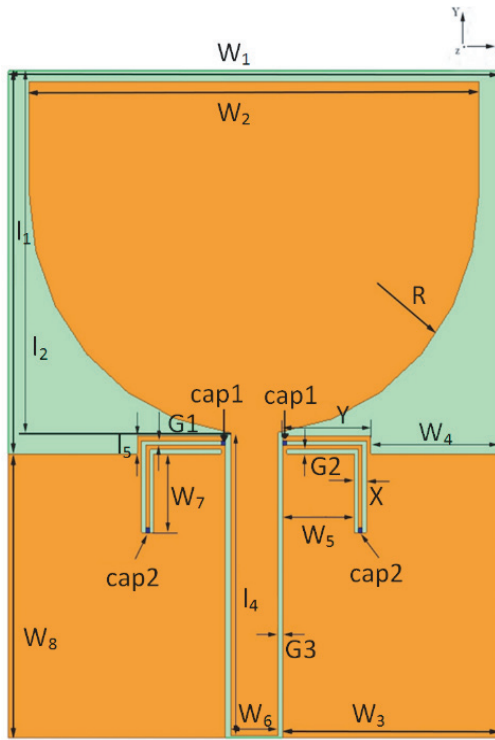
Figure 1. Geometrical parameters of the proposed antenna.
