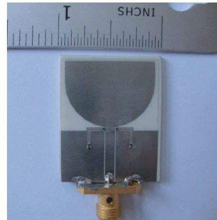
Figure 2. Fabricated monograph of the proposed antenna.
