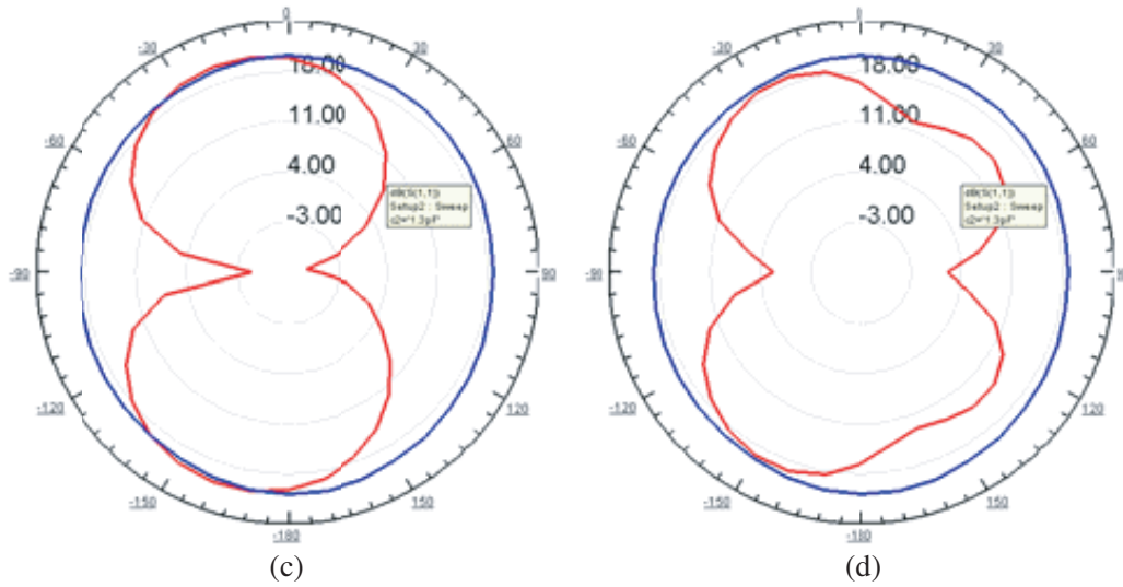
Figure 6. E -plane and H -plane of the proposed antenna. (a) 3.2 GHz, (b) 4.1 GHz, (c) 7.2 GHz, (d) 9.5 GHz. (Red-Line) E -plane and (Blue-line) H -plane.
