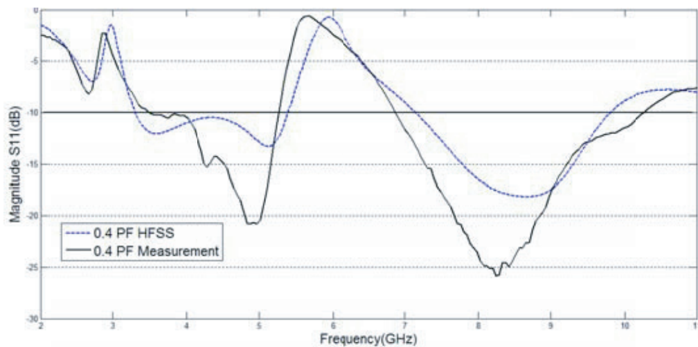
Figure 10. Simulation and measurement magnitude of S_{11} in dB. (Continuous line) measurement and (dash-line) simulation.
