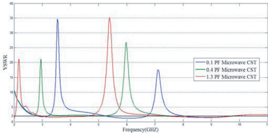
Figure 3. VSWR plot of the proposed antenna at different notched frequencies.
