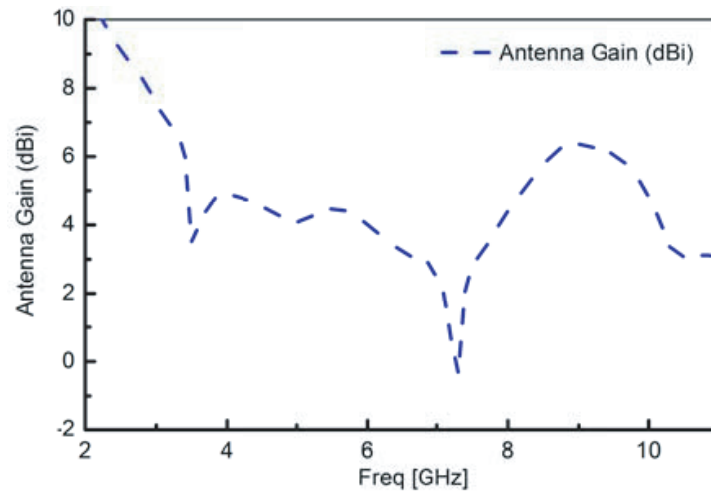
Figure 7. Gain of the proposed antenna at 0.1 pf capacitor.
