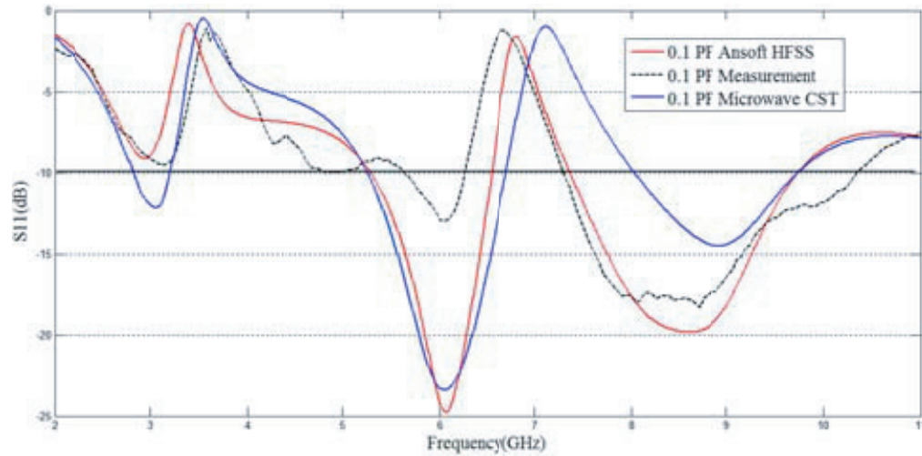
Figure 13. HFSS, CST and measurement results correlation at 0.1 pf.
