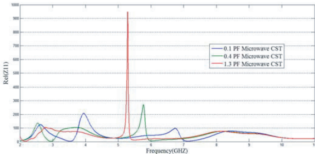
Figure 4. \text{Re}[Z_{11}] plot of the proposed antenna at different notched frequencies.
