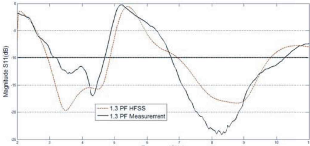
Figure 11. Simulation and measurement magnitude of S_{11} in dB. (Continuous line) measurement and (dash-line) simulation.
