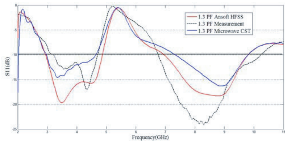
Figure 15. HFSS, CST and measurement results correlation at 1.3 pf.
