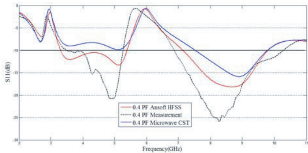
Figure 14. HFSS, CST and measurement results correlation at 0.4 pf.
