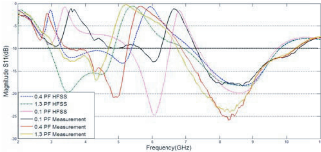
Figure 12. Simulation and measurement magnitude of S_{11} in dB. (Continuous line) measurement and (dash-line) simulation.
