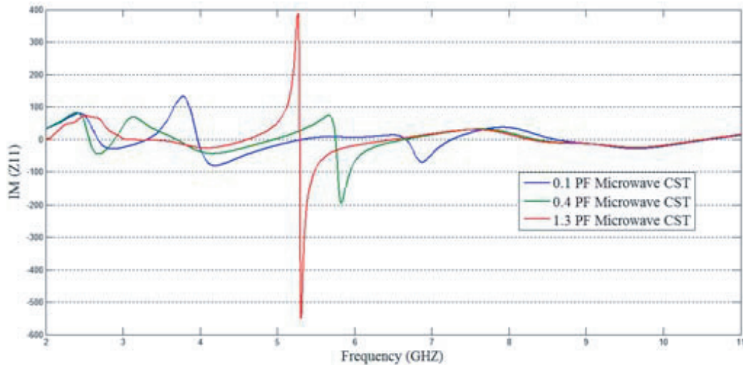
Figure 5. \text{Im}[Z_{11}] plot of the proposed antenna at different notched frequencies.
