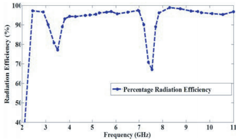
Figure 8. Rad. Efficiency (%) of the proposed antenna at 0.1 pf capacitor.
