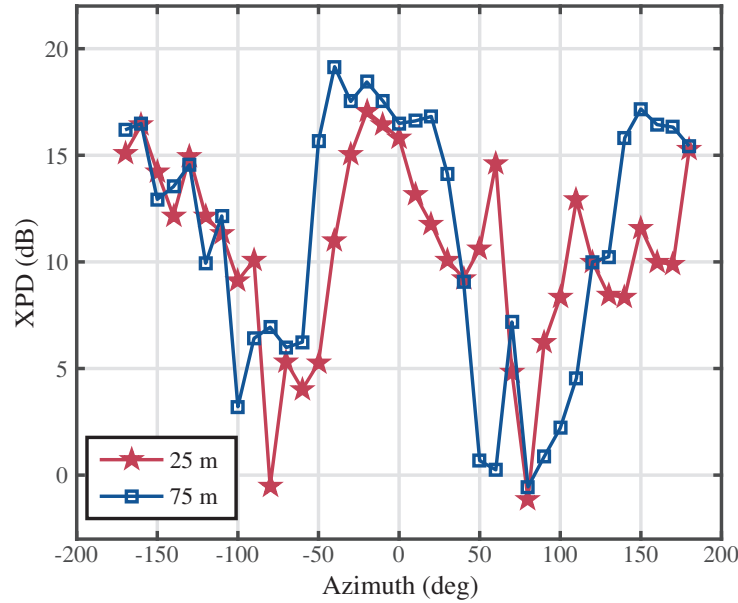
Figure 3. Cross-polarization discrimination.
