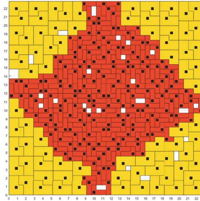
Figure 4. C_{o6} array layout, black squares represent the phase centers of the polyominoes, tetrominoes are in orange, deciminoes in yellow.
