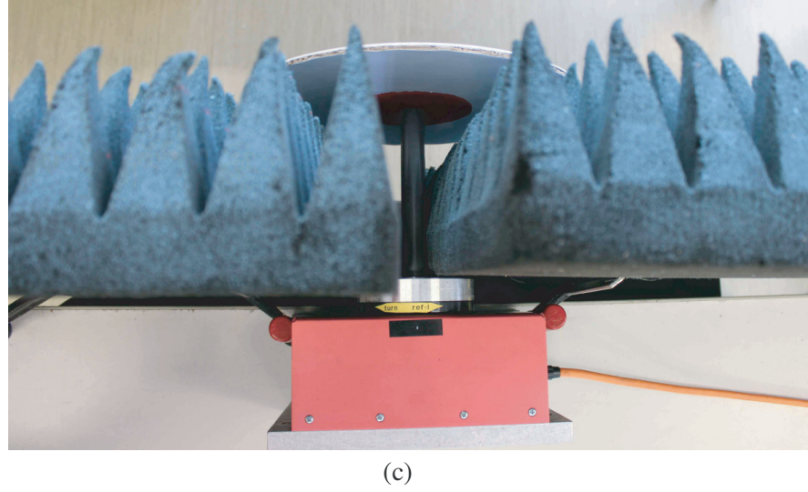
Figure 2. Schematic and photograph of the measurement setup. (a) Schematic: The transmitter is built with an arbitrary waveform generator as baseband signal generator and an external up-converter module. A spectrum analyzer is used as receiver. All units are synchronized. (b) Photograph: The transmit horn antenna is aligned to the turning MUT disc, which reflects the wave back to an aligned receive horn. The MUT disc is backed by absorbers. (c) Close-up of polymeric disc fixture and rotation table (top view).
