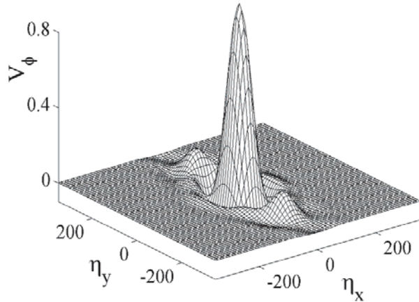
Figure 1. Normalized 3D correlation function of the phase fluctuations at \alpha = 60^\circ .
