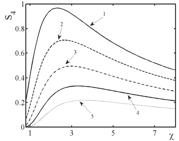
Figure 6. Scintillation index versus anisotropy factor \chi for different characteristic spatial scale of plasma irregularities.
