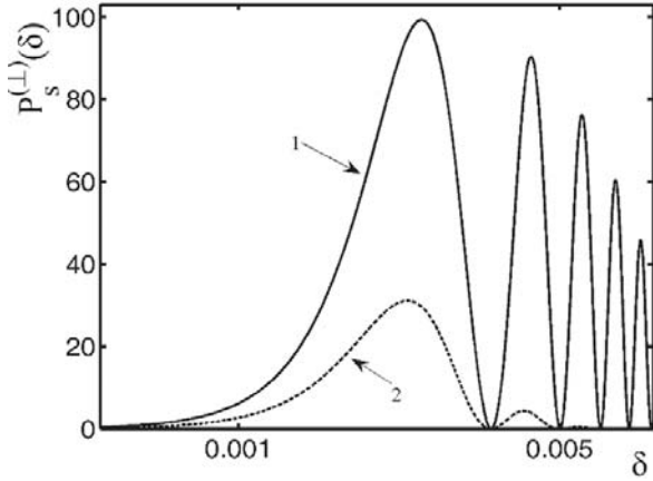
Figure 9. The power spectrum of the phase fluctuations versus parameter \delta for the ordinary and extraordinary waves.
