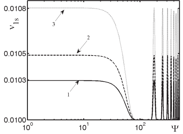
Figure 10. The spectral width (1st moment) of the power spectrum for different orientation angle of elongated plasma irregularities.
