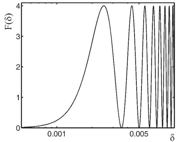
Figure 8. Fresnel filtering factor.
