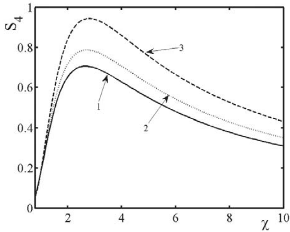
Figure 7. Scintillation index versus anisotropy factor \chi for different orientation angle of anisotropic plasma irregularities.
