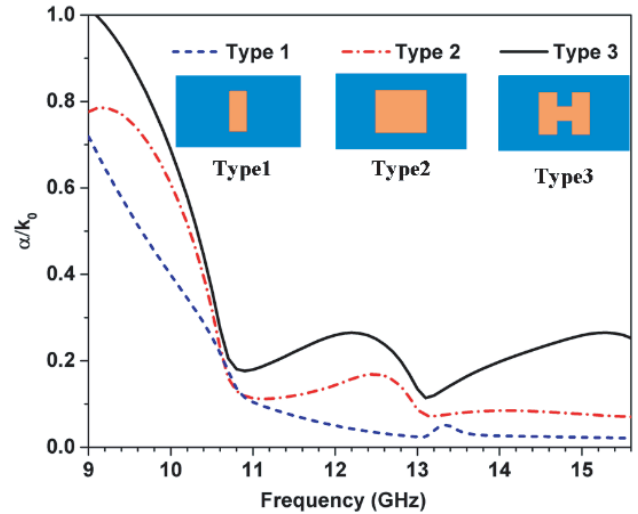
Figure 3. Normalized leakage rate.
