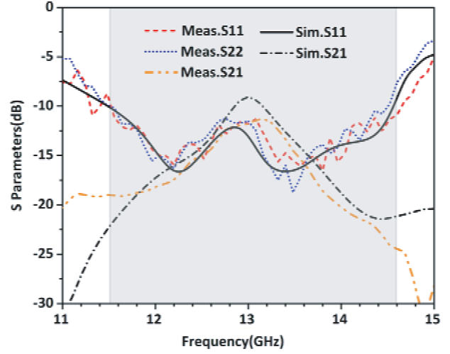
Figure 5. Measured and simulated S parameter.
