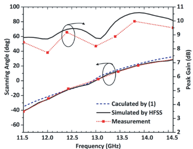
Figure 7. Peak gain and scanning angle with frequency variation.
