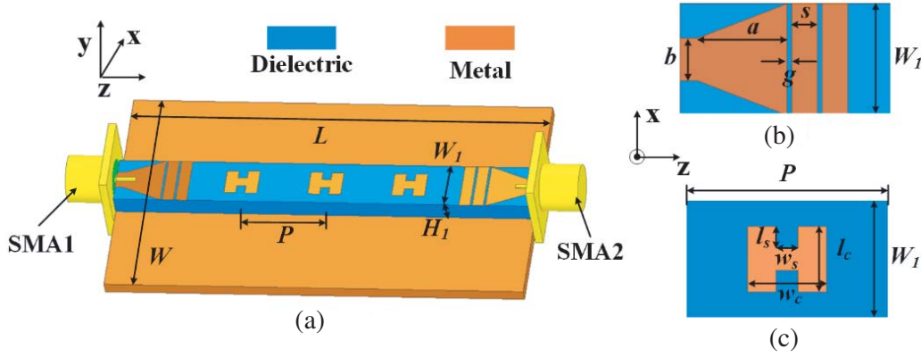
Figure 1. Configuration of the proposed antenna. (a) The overall structure. (b) The feeding network. (c) The H-shaped patch. L = 54.15 mm, W = 40 mm, W_1 = 6.25 mm, H_1 = 2.52 mm, P = 10.75 mm, w_c = 4.2 mm, l_c = 3.5 mm, w_s = 1.2 mm, l_s = 1 mm, a = 5 mm, b = 2.4 mm, g = 0.3 mm, s = 1.5 mm.
