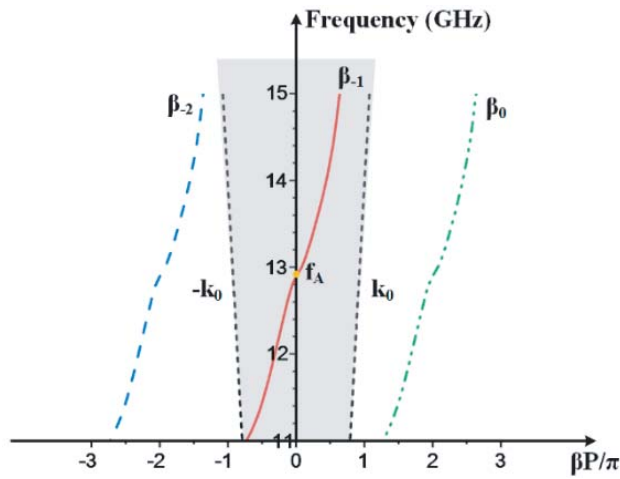
Figure 2. Dispersion diagram of the unit cell.
