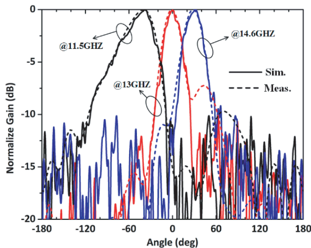
Figure 6. Measured and simulated normalized radiation patterns.
