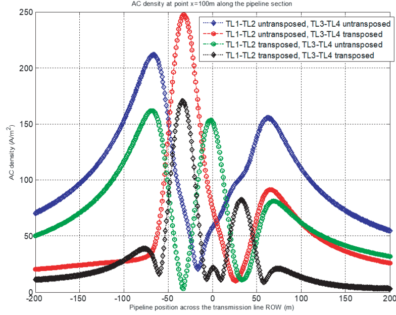
Figure 8. The AC density through a 1 mm defect at 100 m on the pipeline with pipeline variations across the transmission lines due to various phase conductor transpositions.
