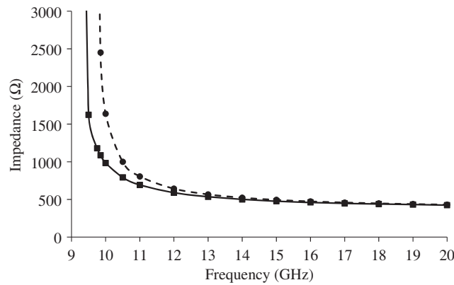
Figure 2. Calculated waveguide impedance across the band for a 45^\circ twist section (solid line with squares) and the rectangular waveguide connected to its ports (dashed line with dots).
