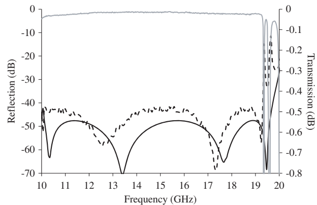
Figure 6. Comparison between measured and simulated performances for the designed 45° twist: Simulated reflection (black solid line), measured reflection (black dashed line) and measured transmission (grey solid line).
