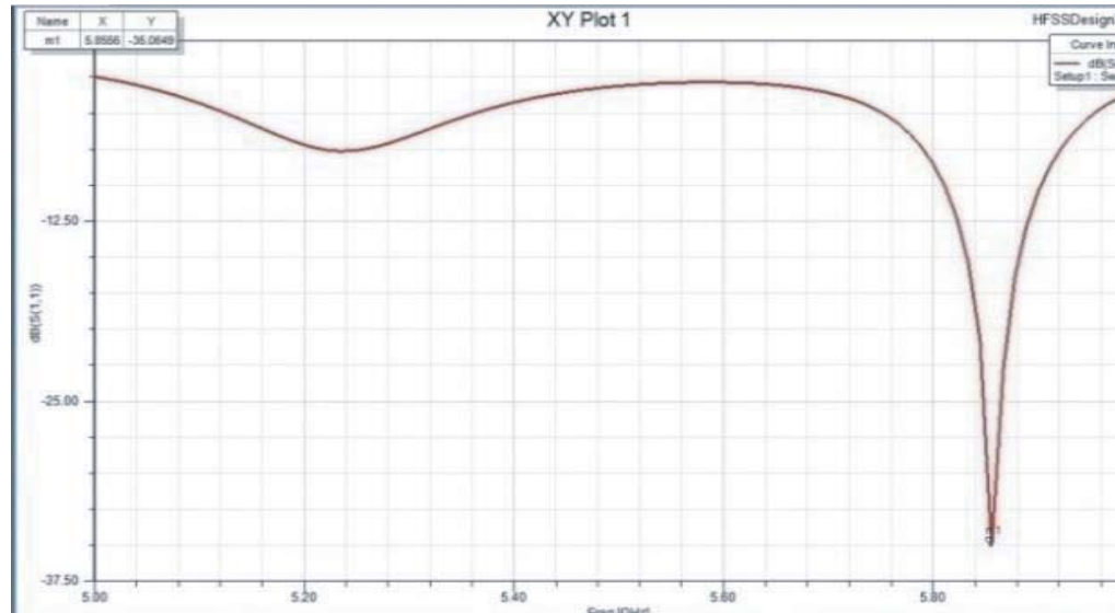
Figure 5. Simulated return loss.
