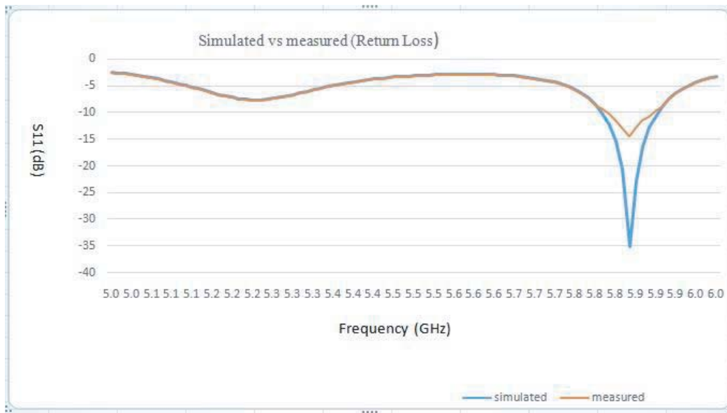
Figure 11. Return loss (simulated vs measured).
