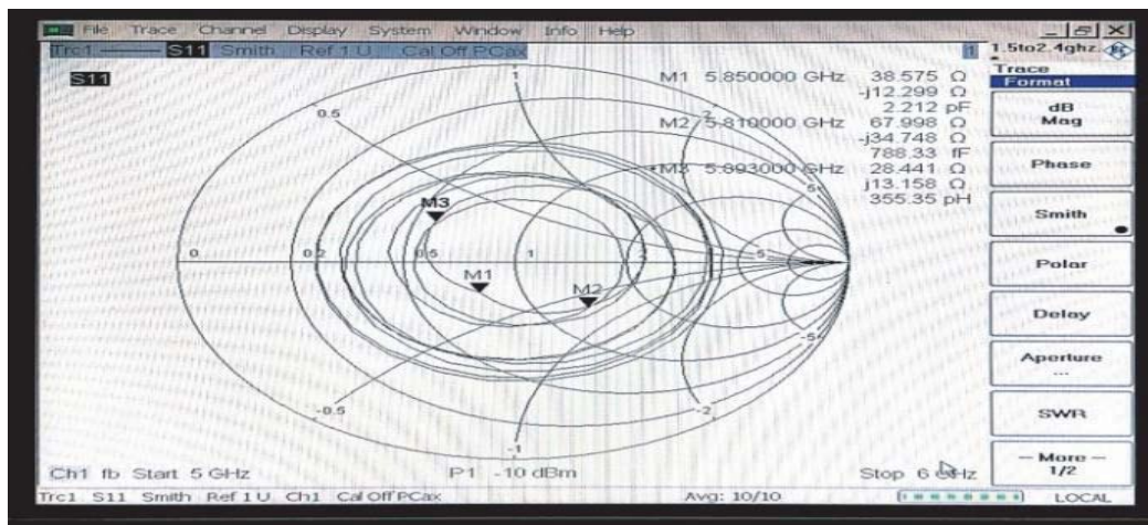
Figure 10. Smith Chart of realized prototype.
