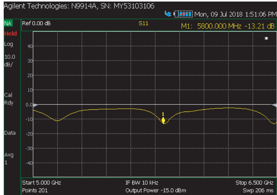
Figure 9. Measured return loss.
