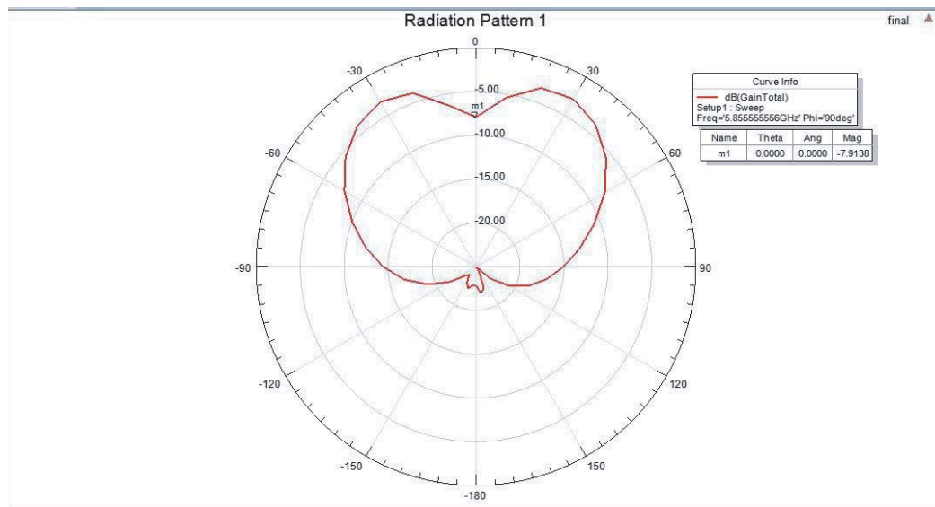
Figure 13. Cross-polarization.
