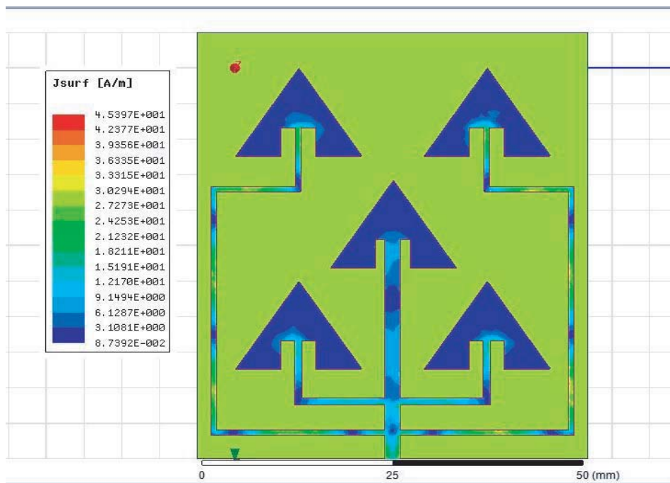
Figure 4. Current distribution.
