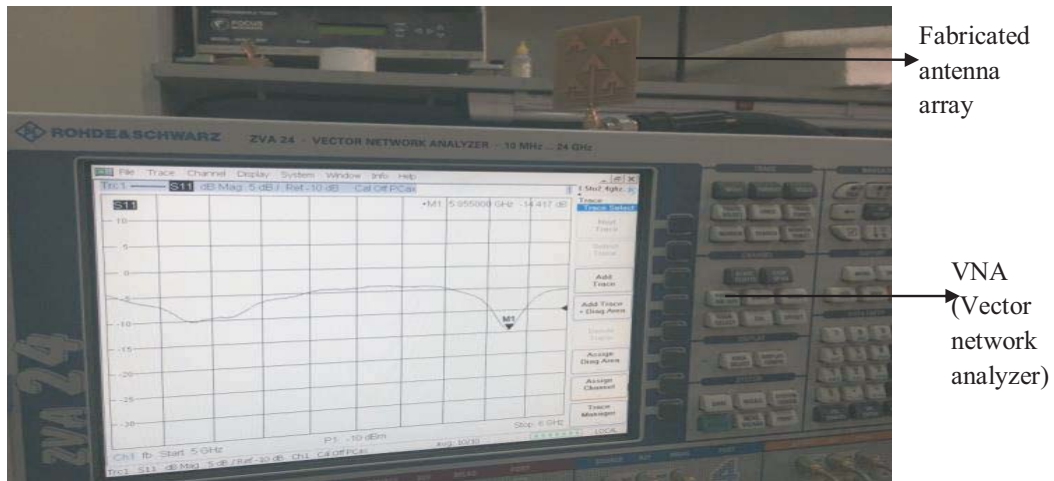
Figure 12. Experimental setup.
