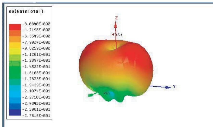
Figure 6. Radiation pattern (3-D).
