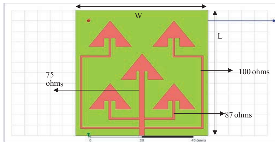
Figure 2. Proposed patch antenna array.
