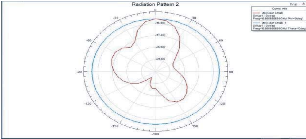
Figure 7. E -plane and H -plane radiation pattern.
