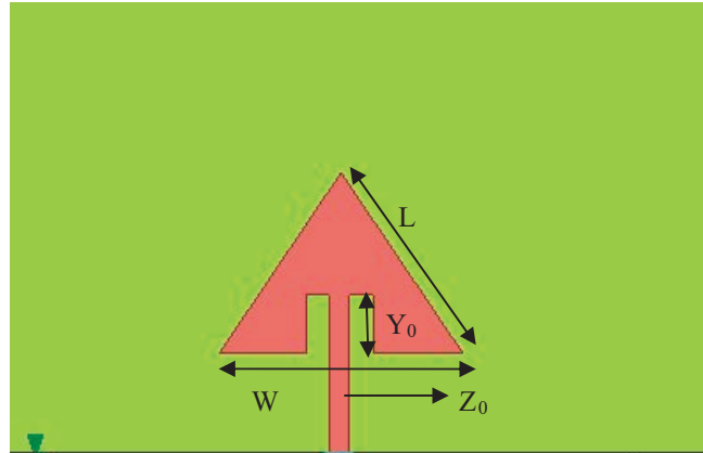
Figure 1. Single C-band microstrip patch.
