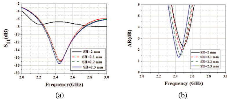
Figure 5. Effect of SH (horizontal length of the stub) on antenna performance: (a) S_{11} . (b) AR.
