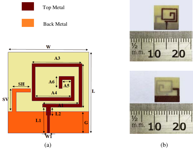
Figure 1. Geometry and photograph of the proposed implantable antenna. (a) Geometry of the designed antenna. (b) Fabricated antenna prototype (Top view and back view).
