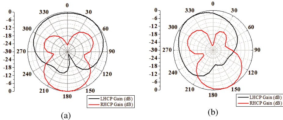
Figure 7. Normalised radiation pattern at 2.45 GHz (a) \Phi = 0^\circ . (b) \Phi = 90^\circ .
