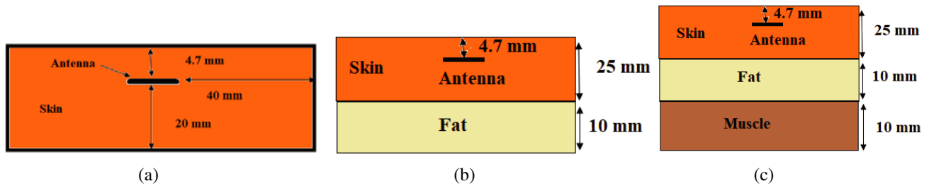
Figure 2. Simulation models: (a) One-layer tissue phantom. (b) Two-layer tissue phantom. (c) Three layer tissue phantom.
