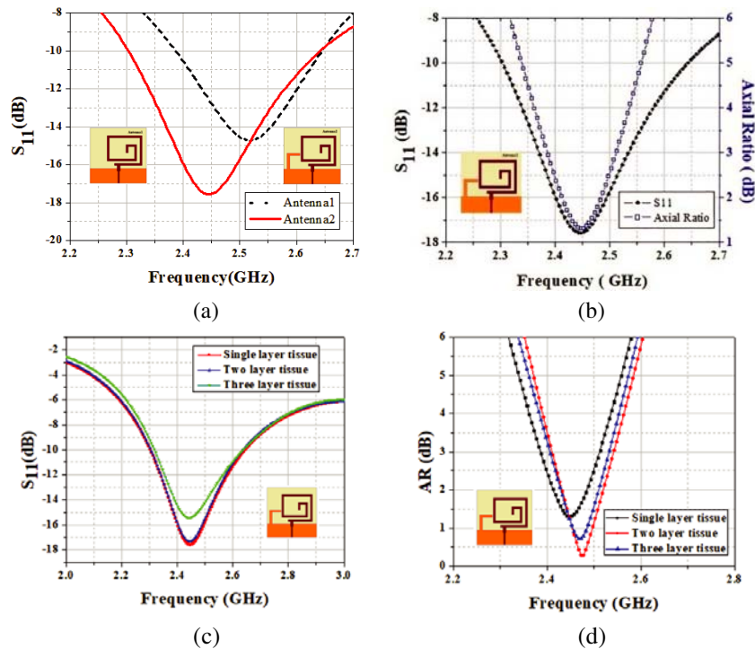
Figure 6. Simulated antenna characteristics. (a) S_{11} of the Antenna1 and Antenna2 in skin phantom. (b) S_{11} and AR of Antenna2 in skin phantom. (c) S_{11} of Antenna2 for different phantoms. (d) AR of Antenna2 for different phantoms.
