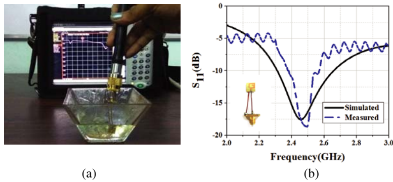
Figure 9. Measurement setup for the proposed antenna. (a) Implantable monopole antenna inside skin mimicking gel. (b) Simulated and measured reflection coefficient.
