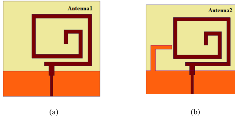
Figure 3. Prototypes of the proposed antenna. (a) Antenna without stub. (b) Antenna with stub.
