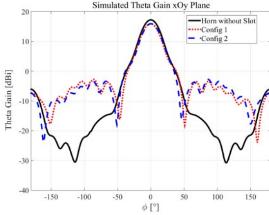
Figure 5. Comparison of simulated theta gains (radar function) in xOy plane at 5 GHz.
