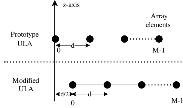
Figure 1. The geometries of prototype ULA and modified ULA.
