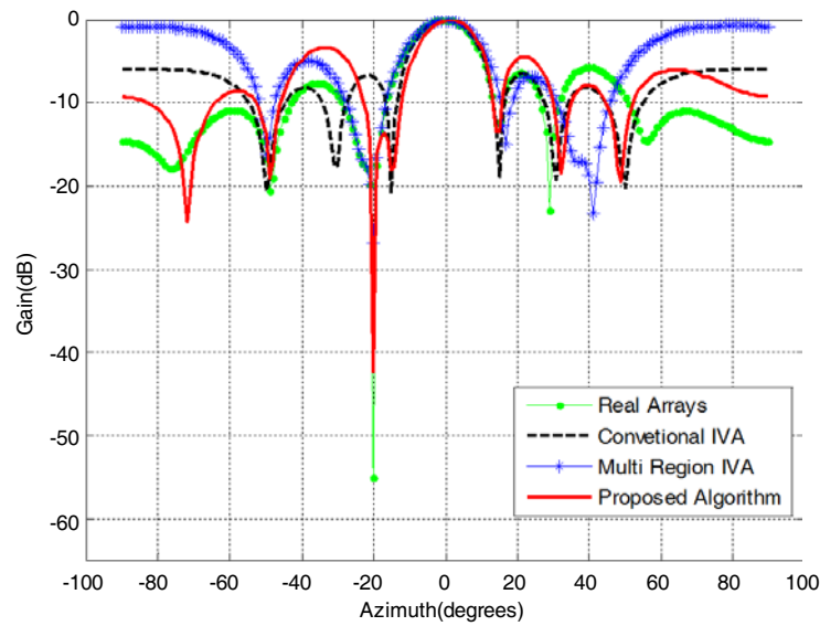
Figure 4. Analysis beamforming under large transformation angle.
