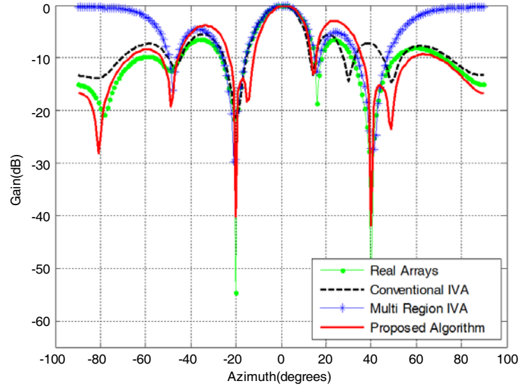
Figure 6. Analysis beamforming under burst interference.
