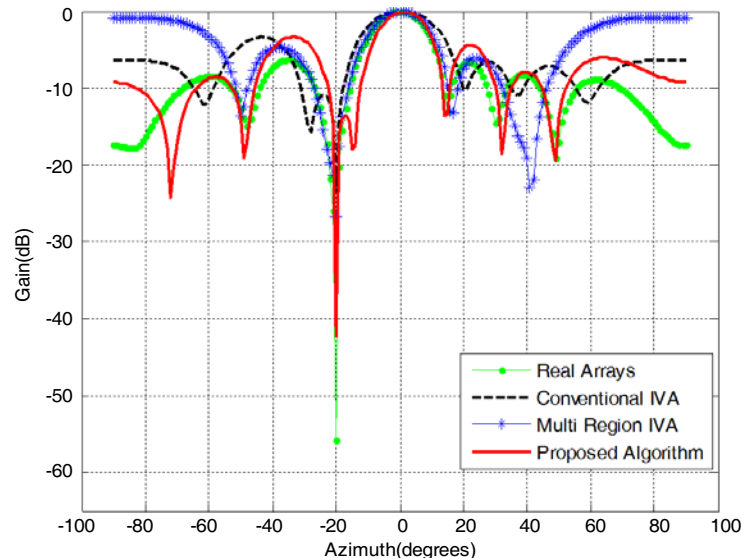
Figure 2. Analysis beamforming under small transformation angle.
