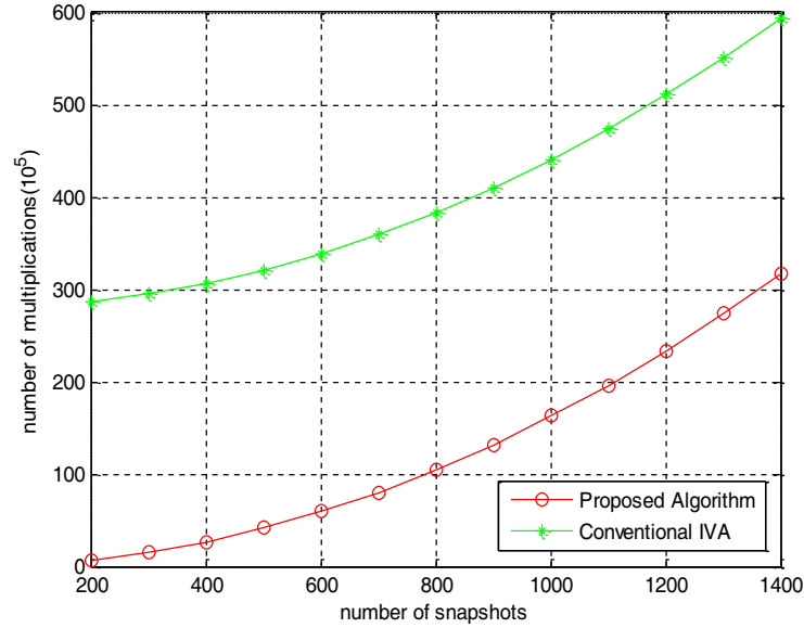
Figure 10. Analysis the number of multiplications with different snapshots.
