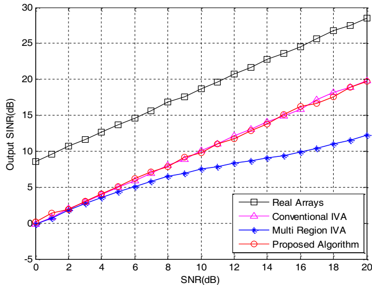
Figure 3. Analysis output SINR under small transformation angle.
