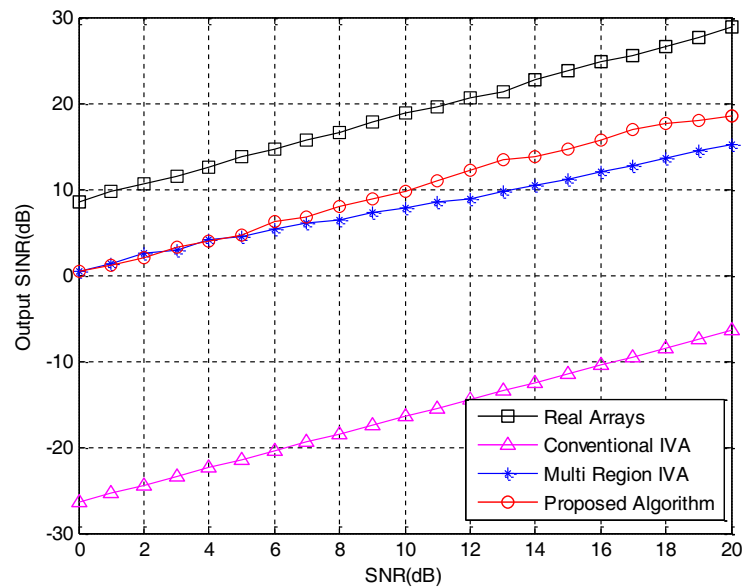
Figure 5. Analysis output SINR under large transformation angle.
