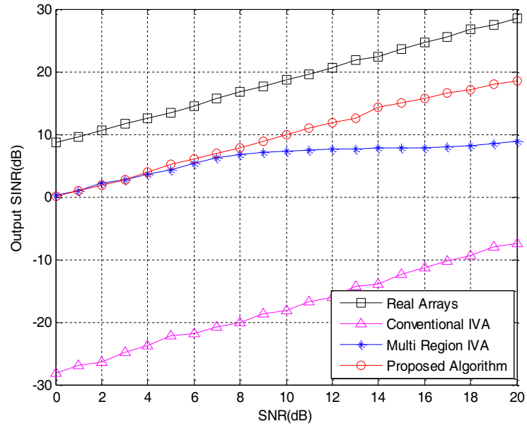
Figure 7. Analysis output SINR under burst interference.
