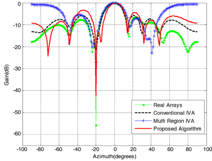
Figure 8. Analysis beamforming with large interpolated step.
