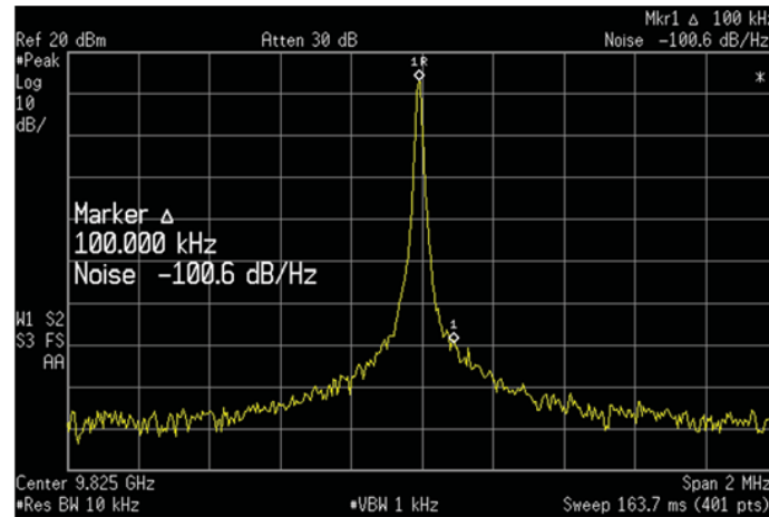
Figure 8. Measured phase noise of the 2nd harmonic for a bias voltage of 4.0 V.
