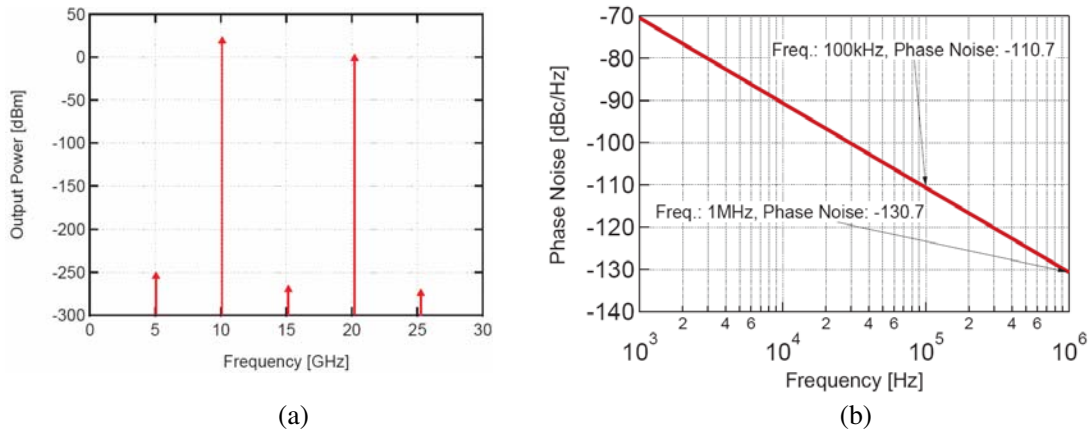
Figure 5. Simulated results for the proposed oscillator. (a) Output spectrum. (b) Phase noise of the 2nd harmonic.
