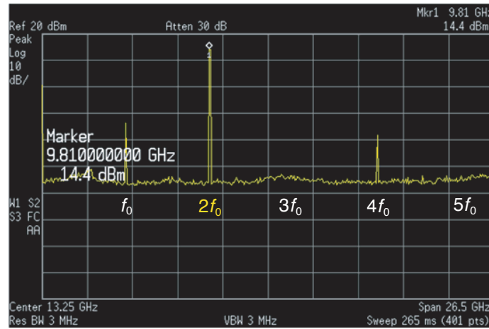
Figure 7. Measured output power spectrum of the oscillator for a bias voltage of 4.0 V.
