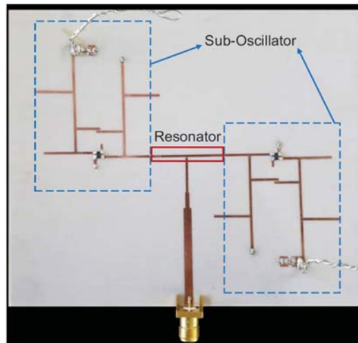
Figure 6. Photograph of the fabricated X-band push-push oscillator using dual-feedback sub-oscillators ( 112 \times 93 \text{ mm}^2 ).
