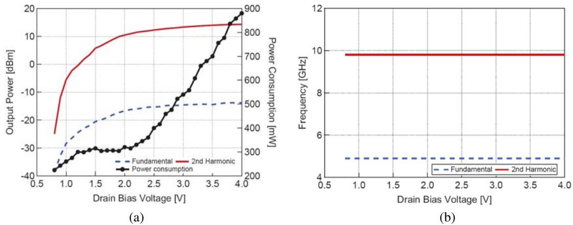
Figure 9. Measured performance with respect to the drain bias voltage. (a) Output power and power consumption. (b) Oscillation frequency.
