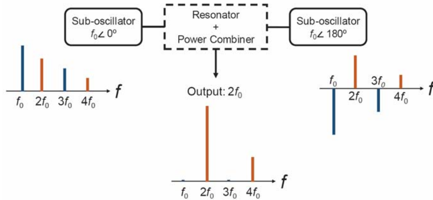
Figure 1. Schematic of a push-push with a resonator that function as power combiner.
