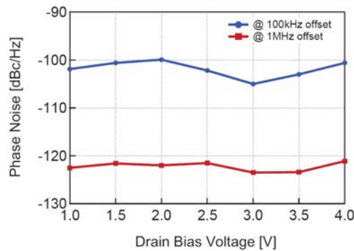
Figure 10. Measured phase noise with respect to the drain bias voltage.
