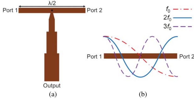
Figure 4. Half-wavelength microstrip line resonator and output network. (a) Circuit diagram. (b) Resonant voltage.
