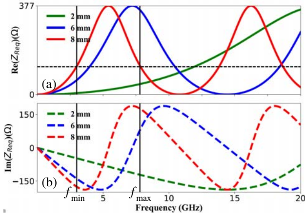
Figure 2. (a) Real part of required impedance. (b) Imaginary part of required impedance. The two solid vertical black lines represent the f_{min} = 3 GHz and f_{max} = 7.8 GHz limits which is our frequency band design goal used in Section 3.
