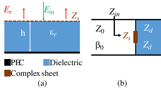
Figure 1. (a) Schematic design of a radar absorber. (b) Transmission line model of the absorber.
