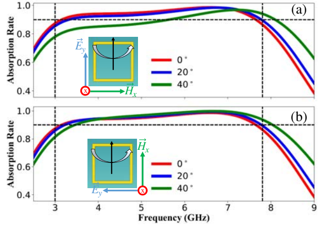
Figure 8. Absorption rate of the proposed structure under oblique incidences of 0–40°. (a) TE polarization. (b) TM polarization.
