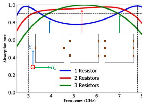
Figure 11. Absorption rate of the PEC with one, two and three resistors in the two vertical arms. The structures were simulated for linearly polarized TE wave.
