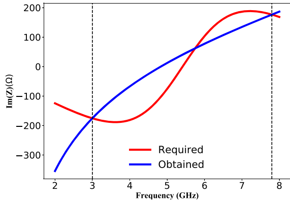
Figure 5. Comparison between \text{Im}(Z) required and calculated \text{Im}(Z) using Equation (8) of the LC model.
