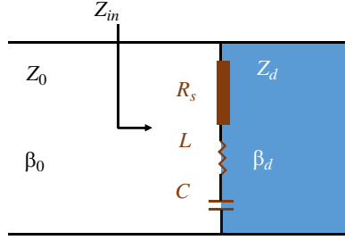
Figure 4. TLM model proposed for broadband absorption.
