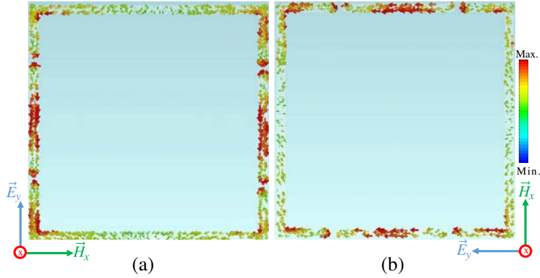
Figure 12. (a) Maximum currents flow on the vertical arms for TE polarization at 5.5 GHz. (b) Maximum currents flow on the horizontal arms for TM polarization at 5.5 GHz.
