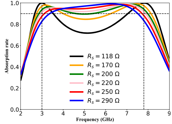
Figure 6. Absorption rate for different values of resistance.
