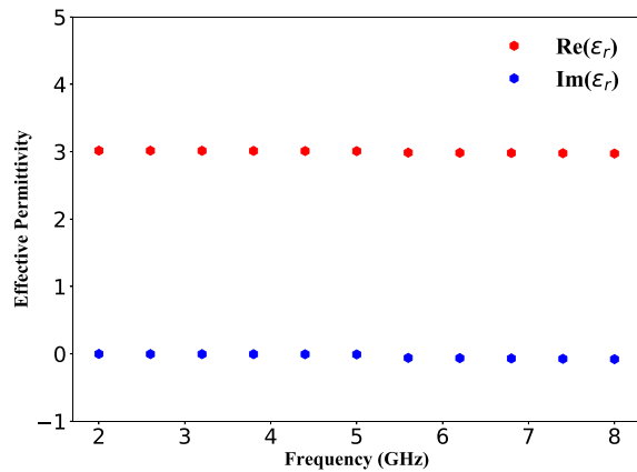
Figure 9. Retrieved real part (red curve) and imaginary part (blue curve) of the effective permittivity of a 0.1 mm thick FR4 substrate placed on top of a 7.9 mm thick rubber substrate.
