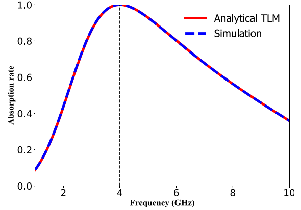
Figure 3. Analytical and simulated absorption rates.
