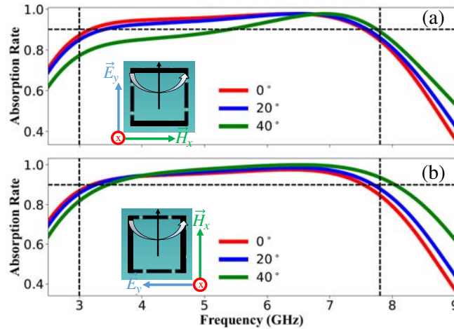
Figure 13. Absorption rate of the proposed structure under oblique incidences of 0–40°. (a) TE polarization. (b) TM polarization.
