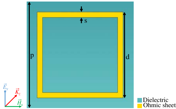
Figure 7. Top view of the unit cell of squared ohmic sheet placed on a 8 mm grounded dielectric.
