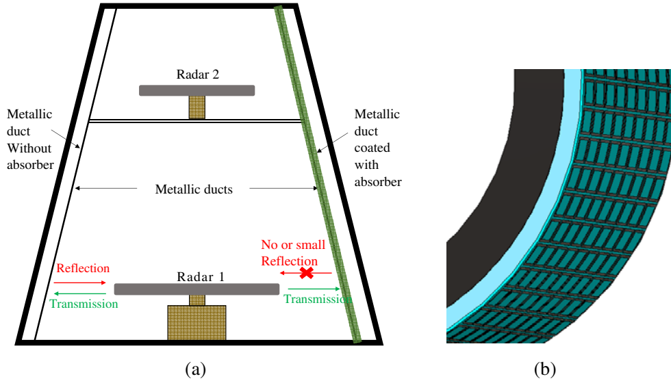
Figure 14. (a) Representation of a metallic duct inside a radome. On the left, the metallic duct is not covered and on the right the metallic duct is covered by a flexible radar absorber. (b) Illustration of the presented absorber conformed on a non planar metallic duct.
