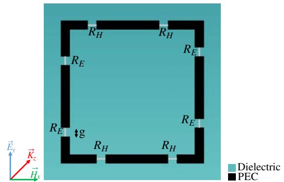
Figure 10. Top view of the unit cell of a PEC square array printed on FR4 substrate placed on top of a 7.9 mm grounded rubber dielectric.
