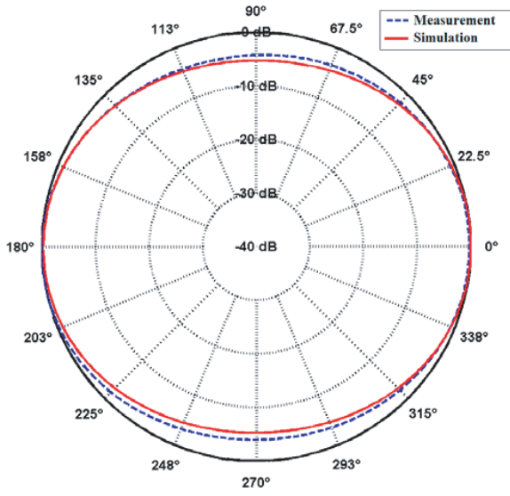
H -plane radiation pattern at 9.0 GHz
