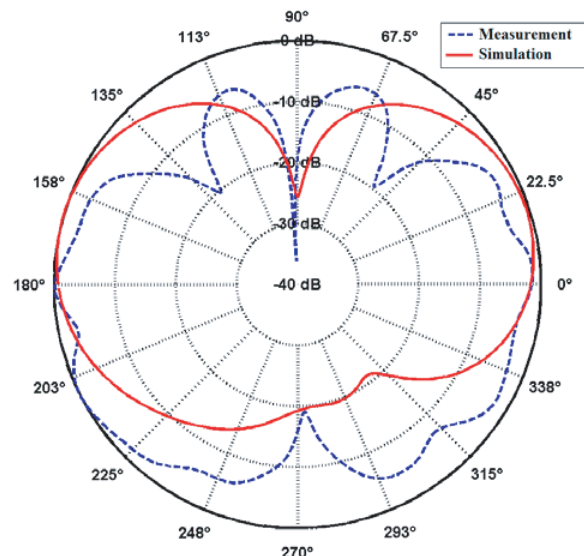
E -plane radiation pattern at 6.5 GHz
