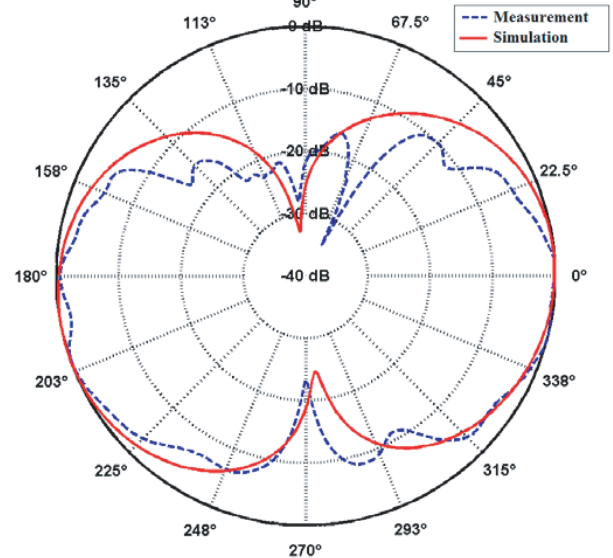
E -plane radiation pattern at 9.0 GHz
