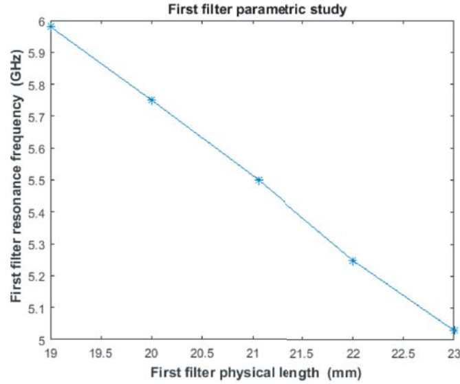
Figure A2. Parametric study of the first filter.
