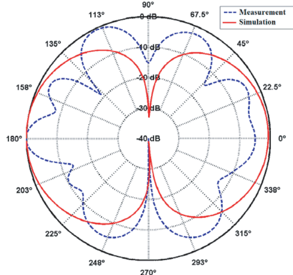
E -plane radiation pattern at 4.0 GHz
