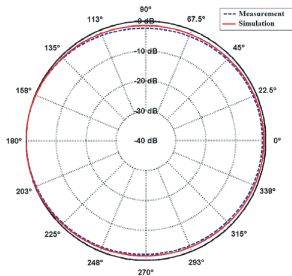
H -plane radiation pattern at 4.0 GHz
