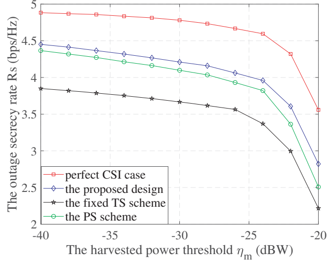
Figure 4. The outage secrecy rate versus the harvested energy threshold.
