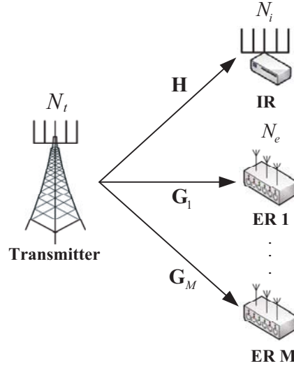
Figure 1. The secrecy MIMO SWIPT system.
