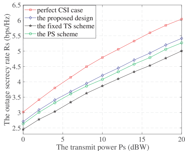
Figure 3. The outage secrecy rate versus the transmit power.
