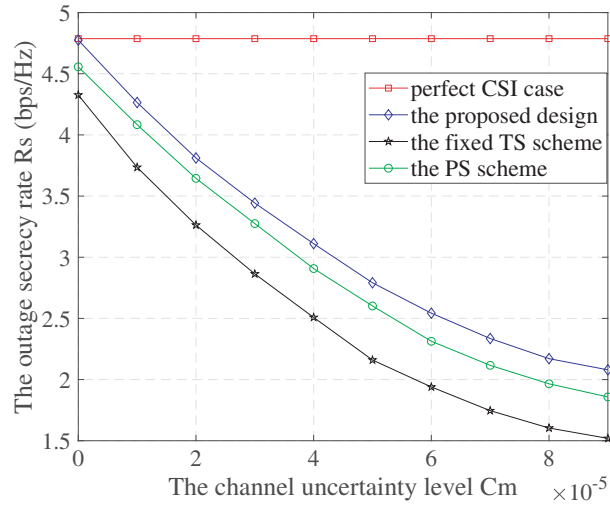
Figure 5. The outage secrecy rate versus the channel uncertainty level.
