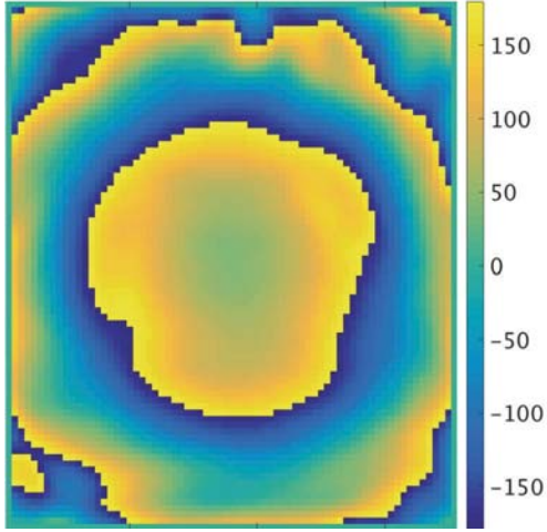
Figure 10. Ideal R_{TE-TE} phase (degrees) requirement at 3.9 GHz.
