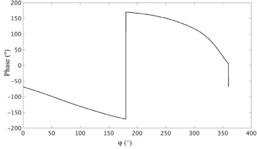
Figure 5. R_{\text{TE-TE}} phase evolution along the equatorial cycle at the central frequency 3.9 GHz.
