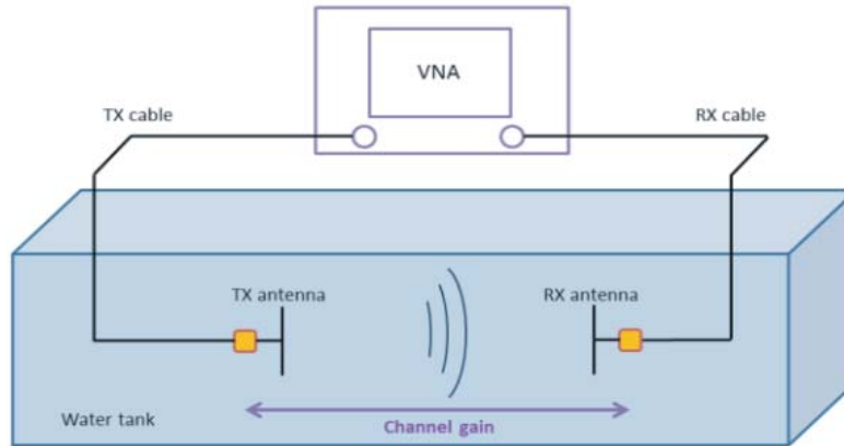
Figure 1. Block diagram of the measurement setup.
