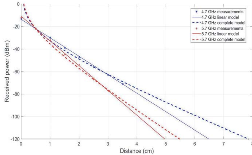
Figure 3. Channel measurements and models fit at 4.7 GHz and 5.7 GHz.
