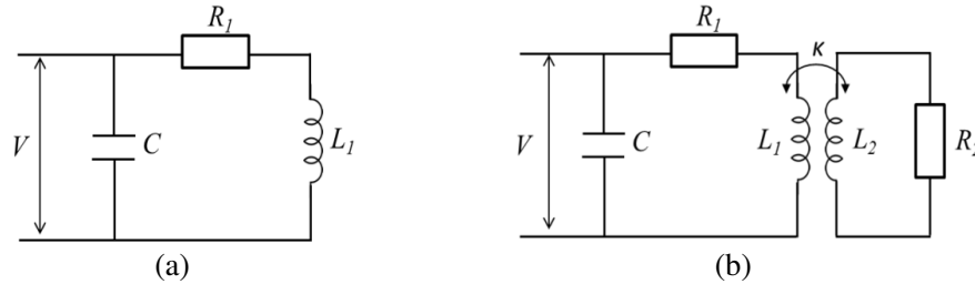
Figure 1. Equivalent circuit model of the sensing system (a) when the probe is on free space, (b) when the probe is on top of a conductive material.
