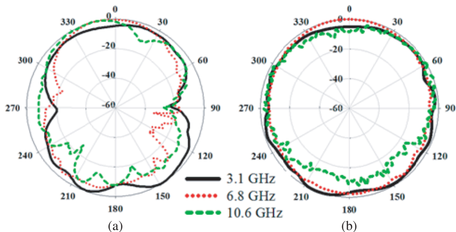
Figure 3. Measured radiation pattern of the proposed antenna (a) E -plane, (b) H -plane at 3.1, 6.8 and 10.6 GHz.
