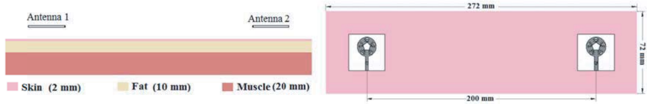
Figure 4. Three layered human tissue model for time domain analysis with identical antenna placed side by side place at a distance of 5 mm from the skin (Front and Top view).
