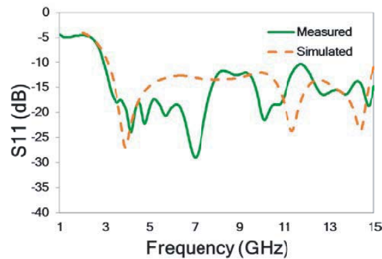
Figure 2. Measured and simulated reflection coefficient of the proposed antenna.
