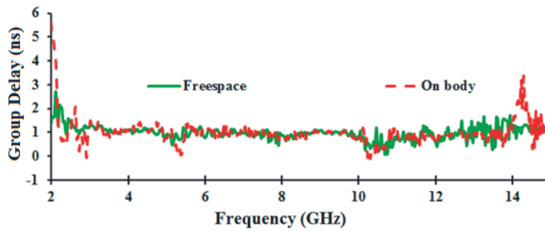
Figure 7. Group delay of the antenna in free space and in close proximity to the body.
