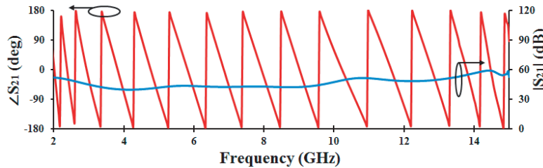
Figure 6. Magnitude and phase of S_{21} for antenna placed side by side on hand.
