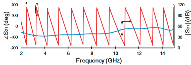
Figure 5. Magnitude and phase of S_{21} for antenna placed side by side in free space.
