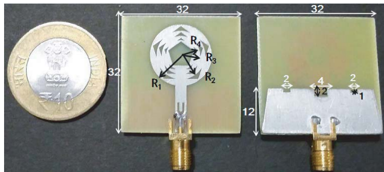
Figure 1. Photograph of the Prototype with dimensional details. (Dimensions are in mm).
