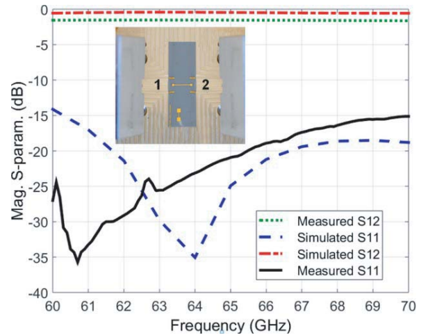
Figure 4. Simulated and measured S -parameters results of the fabricated back-to-back transition prototype over the frequency range of 60 GHz to 70 GHz.
