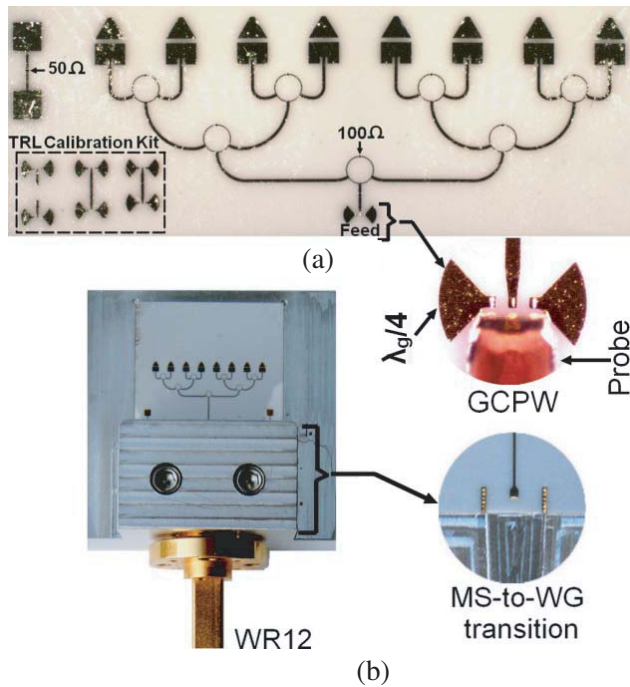
Figure 6. Photograph of the fabricated 8-by-1 gap-coupled antenna array: (a) prototype with grounded coplanar to microstrip line (GCPW-to-MS) transition and, (b) prototype with waveguide (WR12) to microstrip transition.
