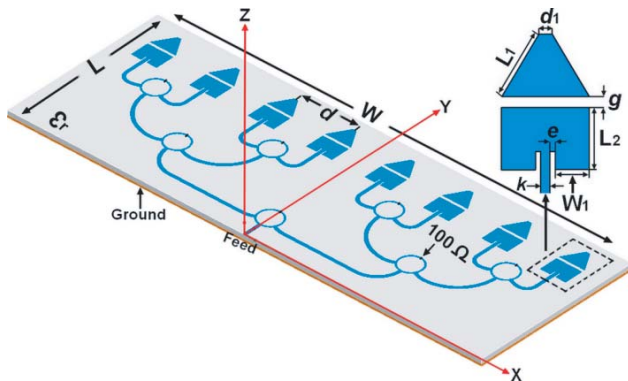
Figure 1. The 8-by-1 gap-coupled antenna array design with the geometrical parameters.
