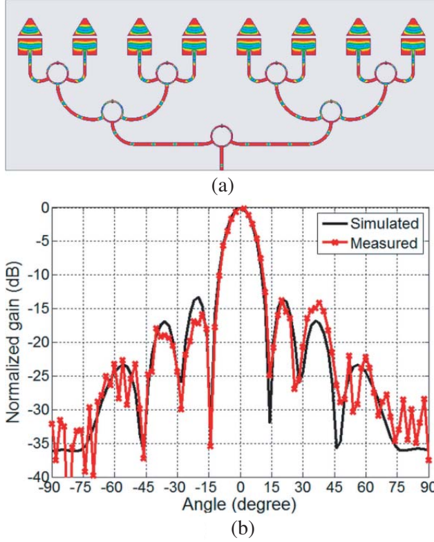
Figure 8. Simulated surface current distributions on the conductor of the 8-by-1 gap-coupled antenna array at 61 GHz in (a), and E -plane measured and simulated radiation pattern in (b).
