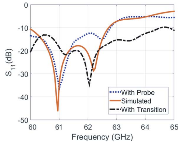
Figure 7. Measured and simulated S -parameters of the fabricated 8-by-1 gap-coupled antenna array.
