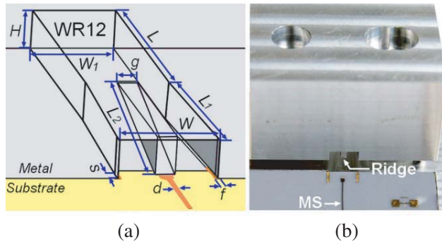
Figure 3. The geometrical parameters of the designed waveguide (WR12) to microstrip transition in (a), and the photograph of the fabricated prototype in (b).
