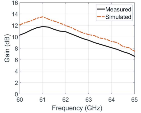
Figure 9. Simulated and measured peak gains of the fabricated 8-by-1 gap-coupled antenna array versus frequency.
