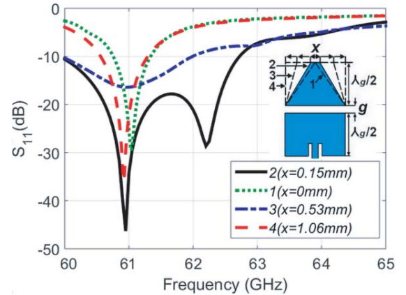
Figure 2. Variation of S -parameters with frequency for different parasitic element base lengths ( x ).
