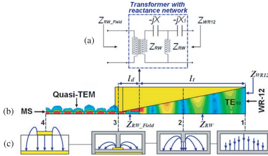
Figure 5. The metal ridge/substrate junction equivalent circuit in (a), simulated electrical field inside transition in (b), and the electric field intensity distributions at the main cross-sections (1–4) in (c).
