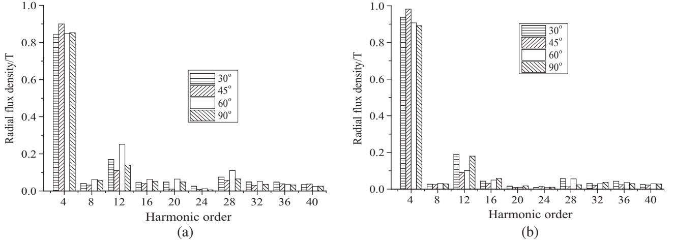
Figure 7. Harmonic spectra of radial flux density. (a) Right angle PM bridge. (b) Arc PM bridge.
