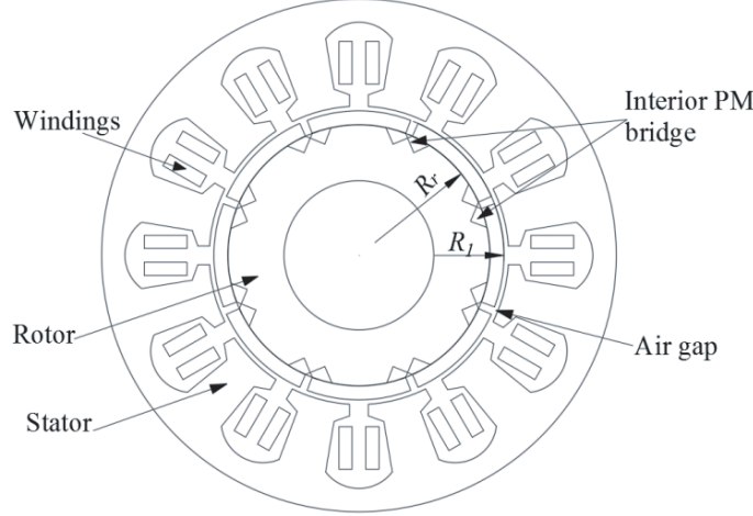
Figure 1. PMSM with interior PM bridge.
