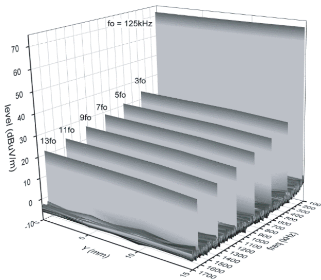
Figure 18. Radiation map of diode rectifier, direction Y, x = 10 mm.
