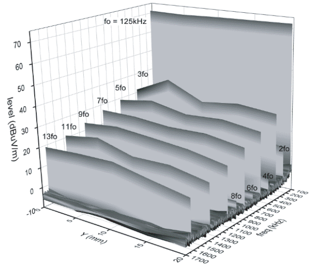
Figure 19. Radiation map of Mosfet rectifier, direction Y, x = 10 mm.
