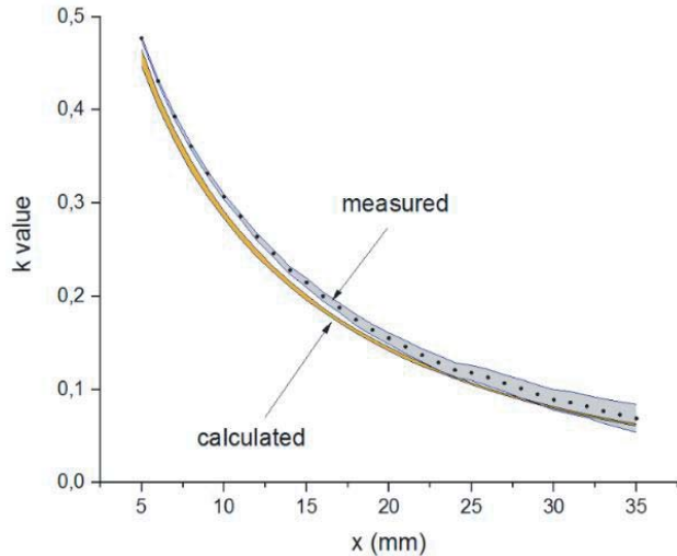
Figure 6. k values, X direction, y = 0 mm.
