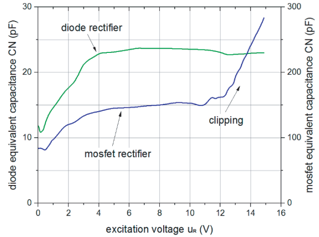
Figure 11. Capacitance equivalent C_N .
