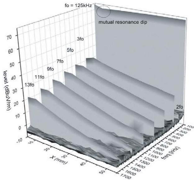
Figure 16. Radiation map of diode rectifier, direction X, y = 0 mm.
