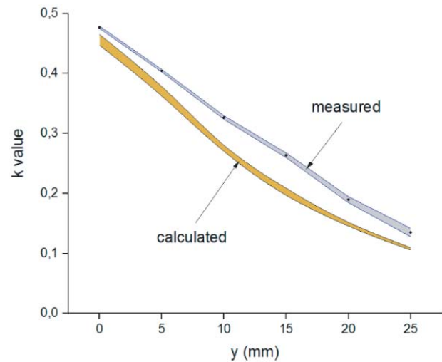
Figure 7. k values, Y direction, x = 5 mm.
