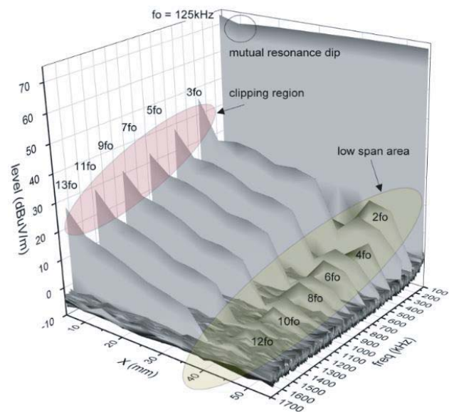
Figure 17. Radiation map of Mosfet rectifier, direction X, y = 0 mm.
