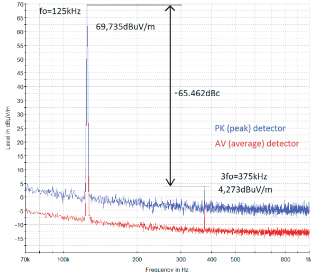
Figure 14. Tx signal quality @1 kΩ load.
