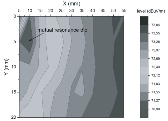
Figure 21. Mutual resonance dip, Mosfet rectifier, f_o = 125 kHz, flat view.
