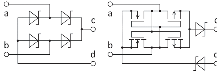
Figure 8. Analyzed AFE structures.
