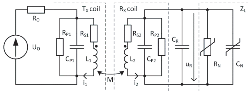
Figure 12. Circuit diagram.
