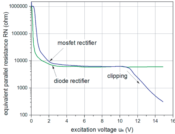
Figure 10. Resistance equivalent R_N .
