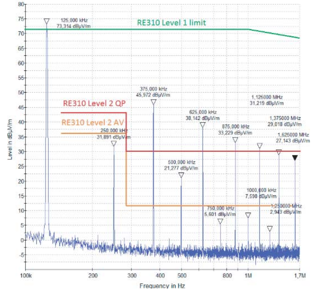
Figure 15. Emission spectrum of Mosfet rectifier, position (5, 0).
