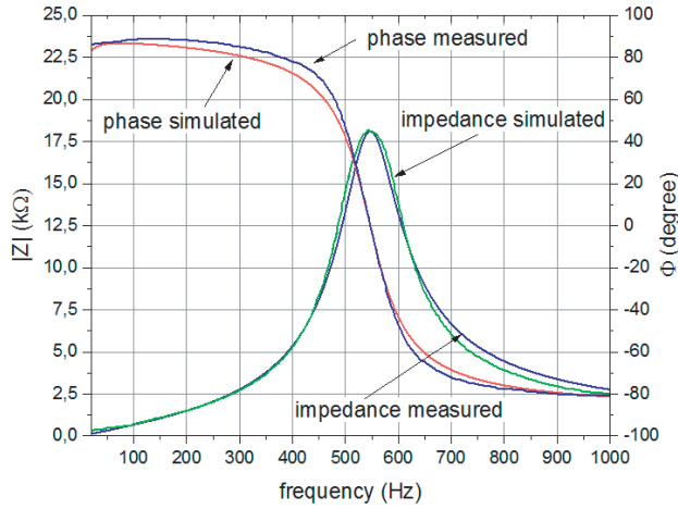
Figure 3. |Z| and phase of Tx coil.
