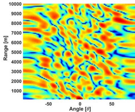
Figure 4. Coding matrix FDM-RDA beamforming with M = 10 at desired receiver location (50^\circ, 6 \text{ km}) .
