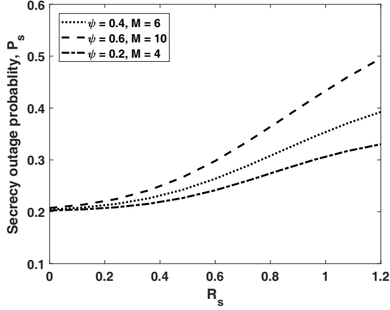
Figure 5. SOP as function of R_s for distinct values of \psi and coding matrix M .
