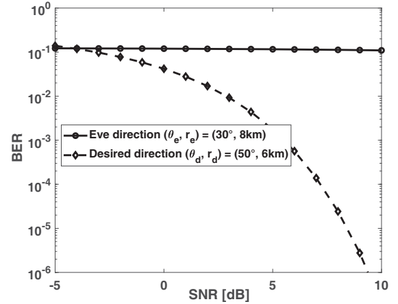
Figure 8. BER comparisons between desired receiver (i.e., at t_1 = 0.02 ms) and Eve receiver (i.e., at t_2 = 0.0277 ms).
