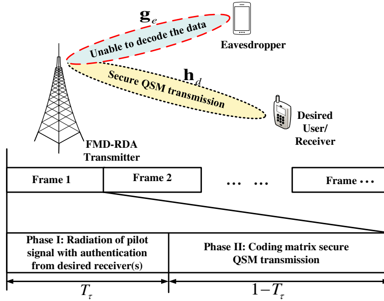
Figure 2. Time frame block is decomposed into two phases: The desired receiver emit pilot signal with authentication during T_r in phase I. After the pilot signal, the FMD-RDA transmitter re-transmit the confidential data during 1 - T_r in phase II.
