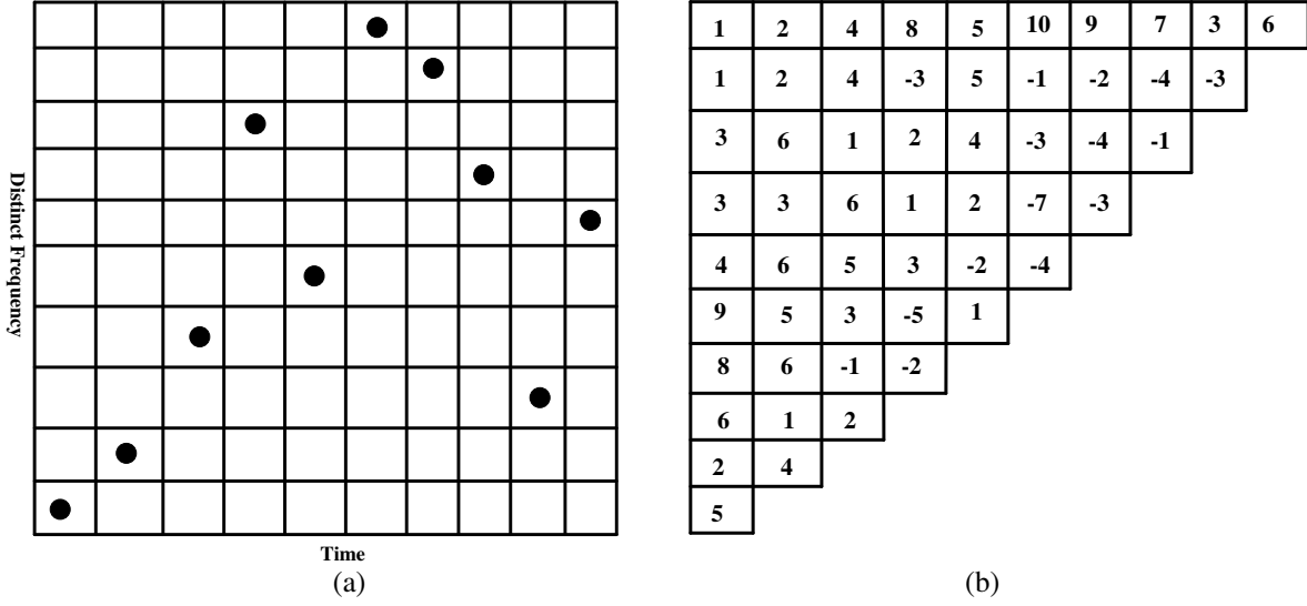
Figure 3. Illustration of (a) Coding matrix c_s , M = 10 : \{1, 2, 4, 8, 5, 10, 9, 7, 3, 6\} and (b) Difference matrix design.
