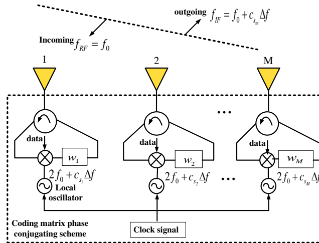
Figure 1. Proposed coding matrix frequency modulated diverse retrodirective array secure transmitter for QSM transmission in mmWave communications: Note c_{sm} = \{c_{s1}, c_{s2}, \dots, c_{sM}\} denotes the coding matrix for frequency increments \Delta f , namely \{1, 2, 4, 8, 5, 10, 9, 7, 3, 6\} .
