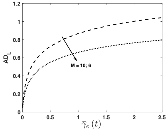
Figure 7. Illustration of AD_L against \bar{\gamma}_e(t) for distinct values of coding matrix M .
