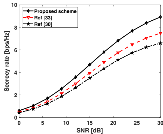
Figure 9. Secrecy rate vs SNR comparisons.
