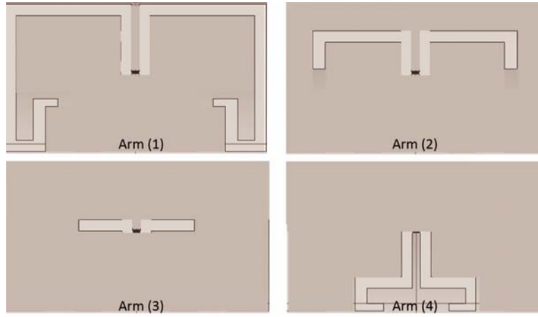
Figure 3. Design conception steps.
