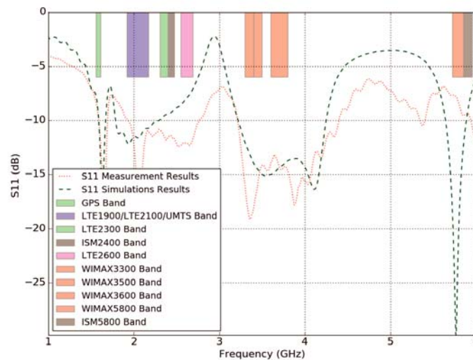
Figure 8. S_{11} simulation vs measurements results.
