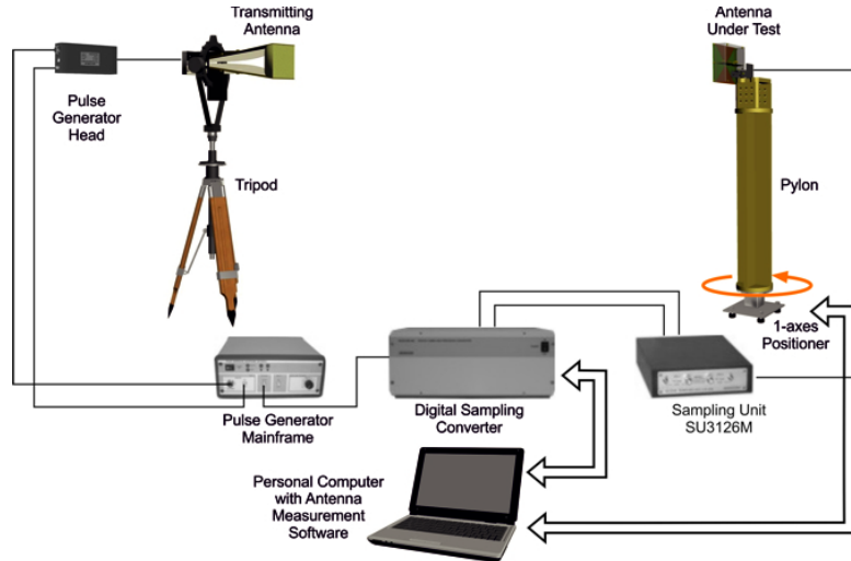
Figure 7. Measurement setup for the radiation pattern.
