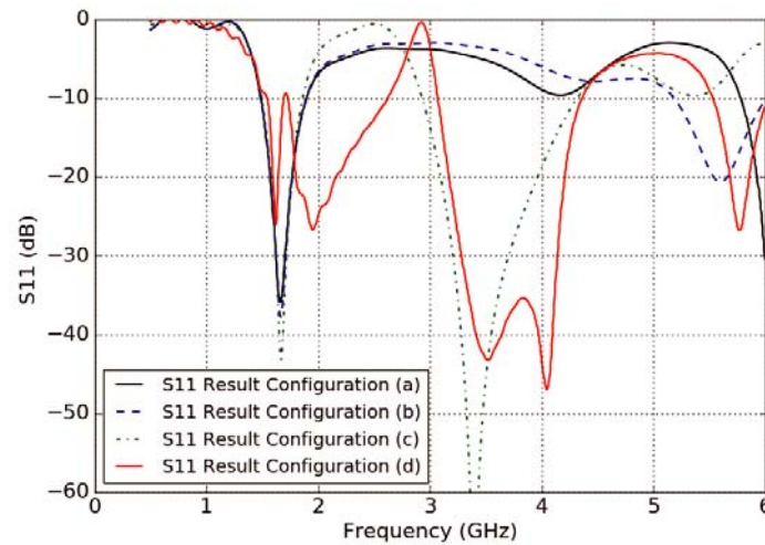
Figure 4. S_{11} simulation result for each configuration.
