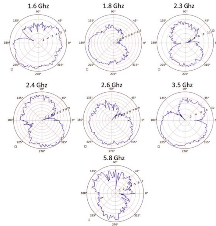
Figure 10. Azimuth of the radiation pattern measurements results in each frequency.
