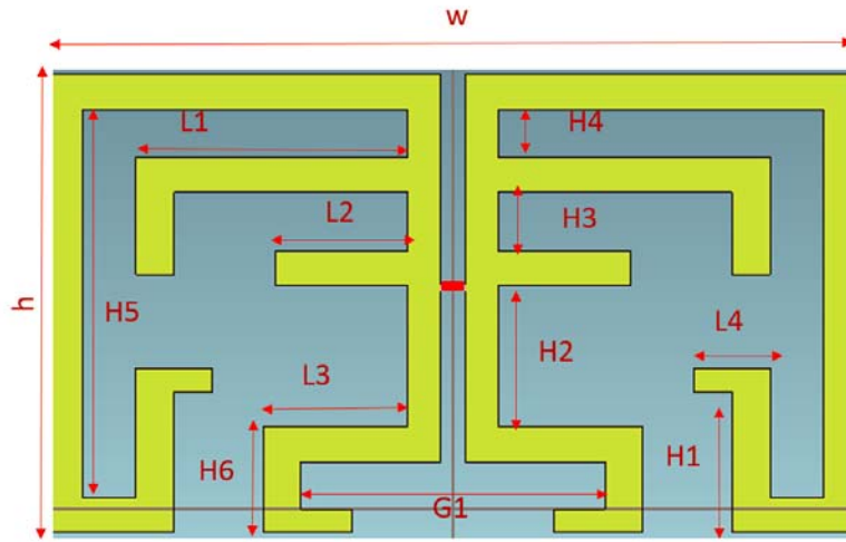
Figure 5. Antenna conception parameters. Each length is a parameter for the antenna conception.
