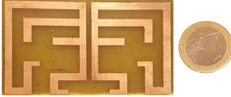
Figure 6. Manufactured antenna design.
