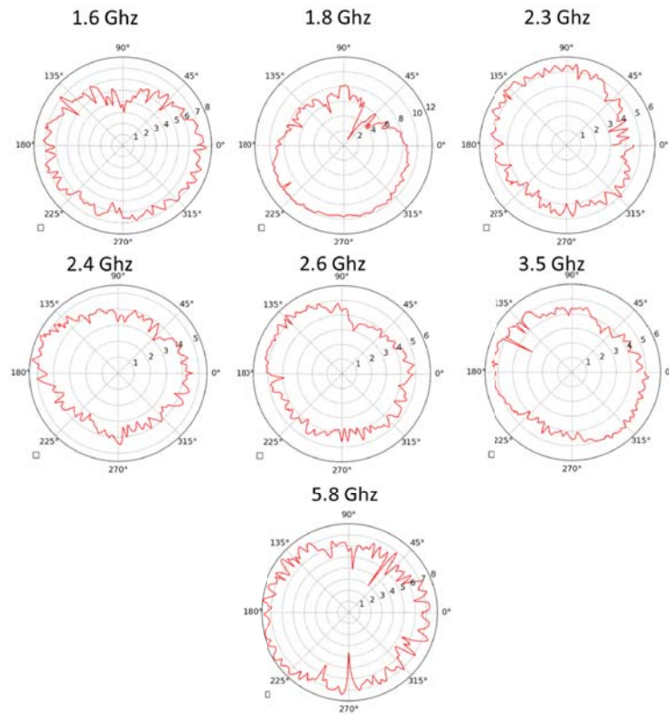
Figure 9. Elevation of the radiation pattern measurements results in each frequency.
