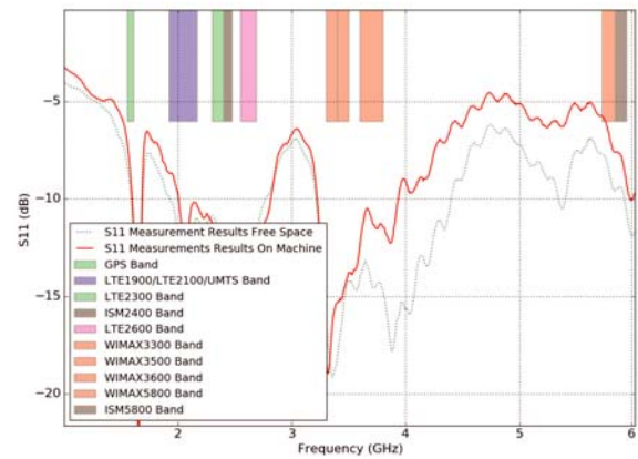
Figure 12. Influence of the machine automaton on the antenna in term of S_{11} .
