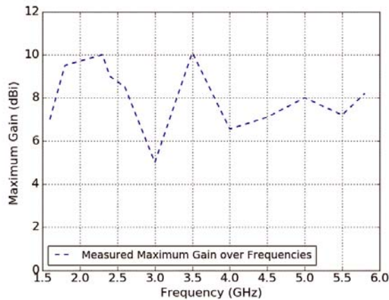
Figure 11. The maximum gain measurements over frequency.
