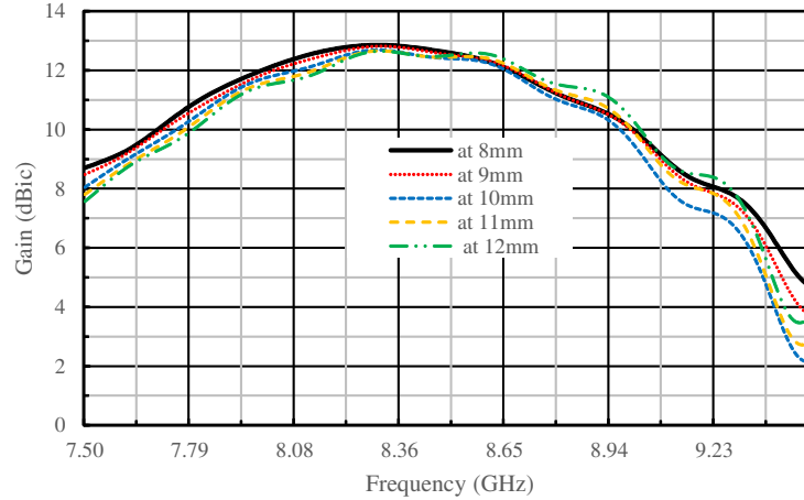
Figure 8. Effect of the feeding line length to the gain.
