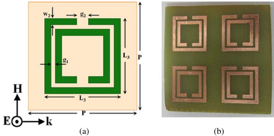
Figure 1. Split ring resonator structure. (a) Schematic topology of the unit cell. (b) Fabricated prototype of 2 \times 2 arrays of the unit cell.
