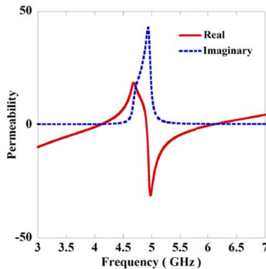
Figure 2. Retrieved effective permeability of the unit cell of SRR.
