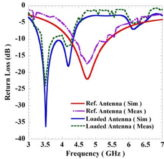
Figure 4. Simulated and measured return loss characteristics for the metamaterial loaded and the reference dipole planar antenna.
