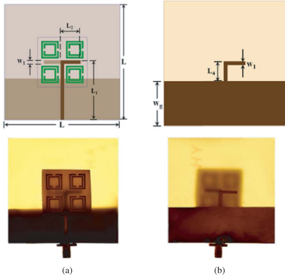
Figure 3. Schematic topology and fabricated prototype of the loaded antenna. (a) Front view. (b) Back view.
