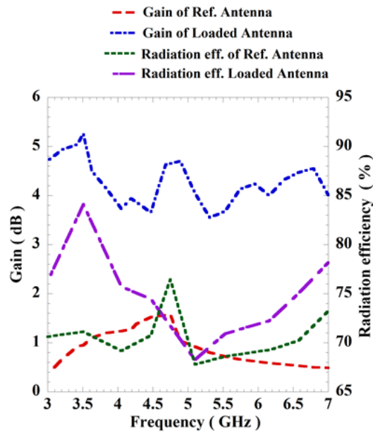
Figure 5. Measured gain and efficiency vs. frequency plot of MTM loaded dipole w.r.t reference dipole.
