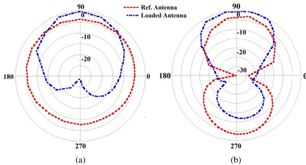
Figure 6. Normalized measured radiation pattern of MTM loaded dipole w.r.t reference dipole (a) E -plane and (b) H -plane.
