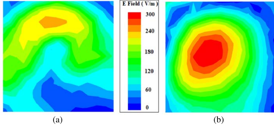
Figure 7. Simulated electric field distribution at the respective resonance frequency. (a) Reference antenna. (b) Metamaterial loaded antenna.
