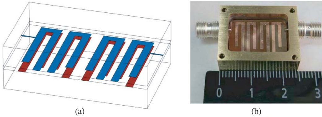
Figure 6. (a) Structure of the proposed 4-pole filter based on the resonator of the type C. (b) Photo of the fabricated filter.
