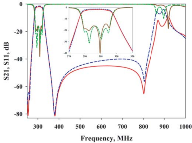
Figure 7. Simulated (blue and green dashed curve) and measured (red and brown solid curve) frequency responses of the filter.
