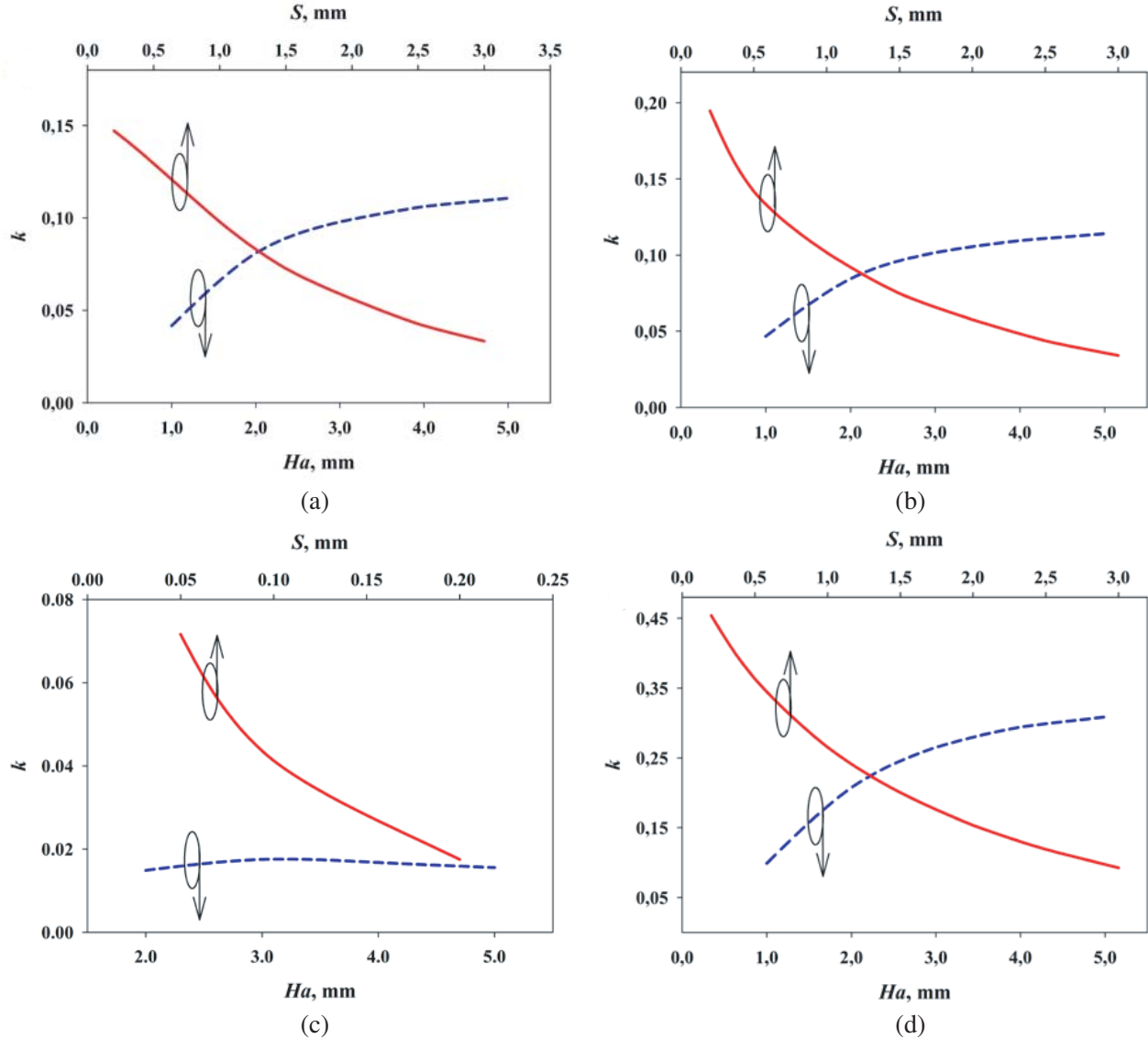
Figure 5. Dependencies of the coupling coefficient vs space S between resonators (red solid curve) and a distance from substrate's faces to shielding covers (blue dashed curve). (a) and (b) for the sections consisting of resonators C ; (c) and (d) for the sections consisting of resonators D .
