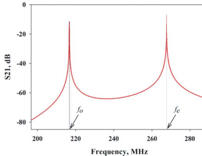
Figure 3. Typical response of a two-resonator section having large external Q -factor.
