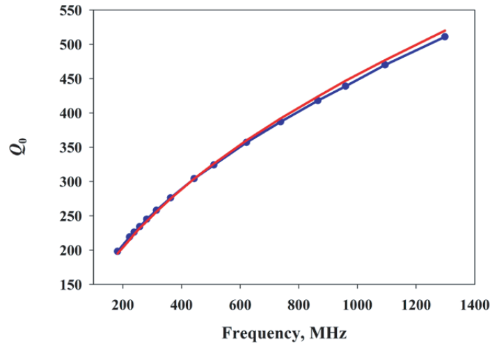
Figure 2. Q -factor of the two-conductor resonator on a suspended substrate vs resonant frequency. Blue line is a result obtained with a help of simulation, red curve is an approximation by the formula (4).
