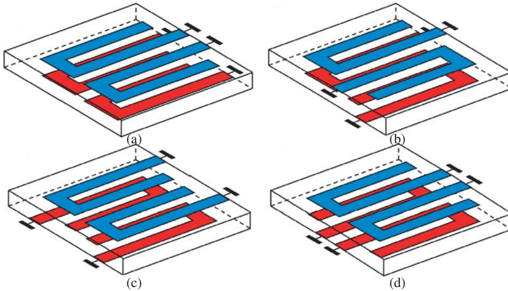
Figure 4. Two-resonator sections: (a) and (b) are two arrangements of the resonators C ; (c) and (d) are two variants of the section consisting of the resonators D .
