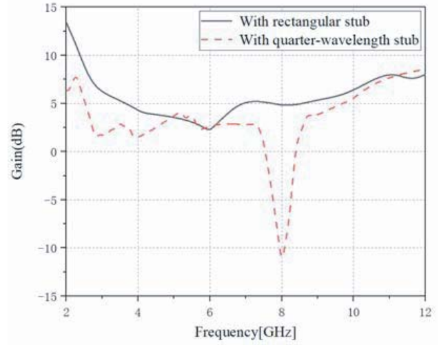
Figure 5. Gain of the proposed antennas.
