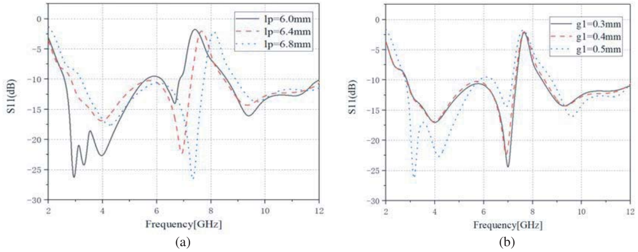
Figure 3. The influence of each parameter on the notch frequency.
