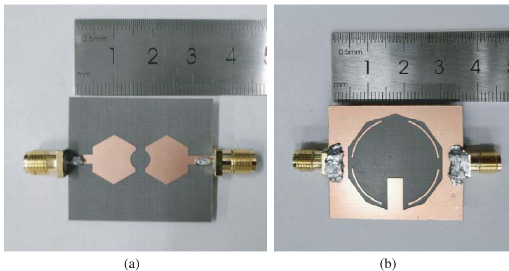
Figure 7. Fabricated sample of the proposed antenna. (a) Radiation patch. (b) Grounding plate of the proposed antenna.
