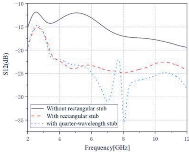
Figure 4. Isolation of the proposed antennas.
