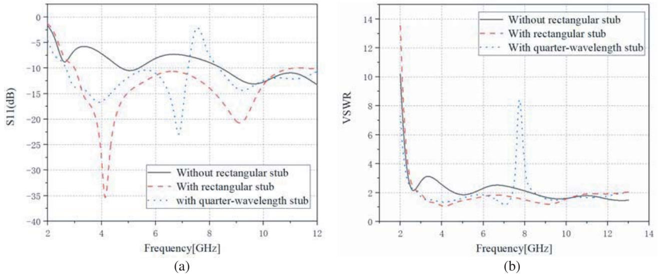
Figure 2. The simulated reflection coefficient and VSWR characteristic of the proposed antenna. (a) S_{11} . (b) VSWR.
