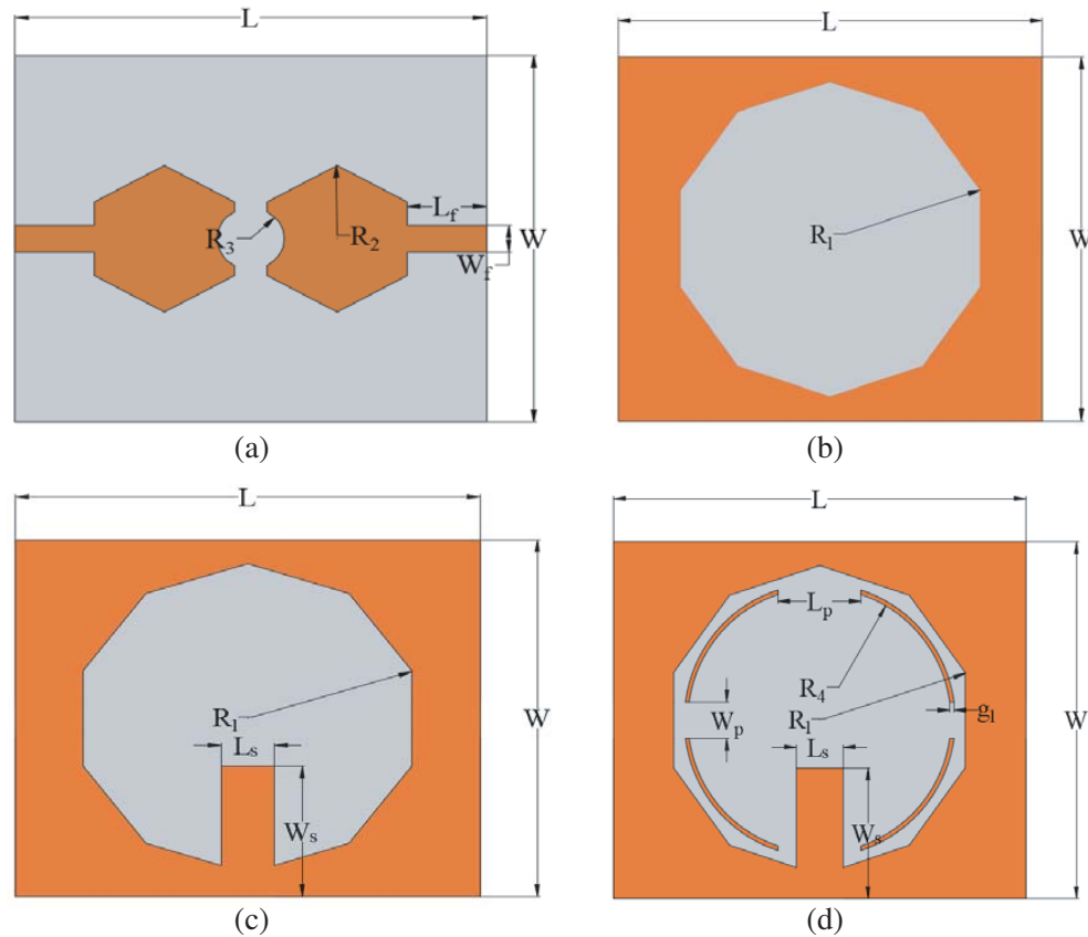
Figure 1. Design evolution and geometry of the proposed antenna. (a) Radiation patch. (b) Grounding plate of antenna 1. (c) Grounding plate of antenna 2. (d) Grounding plate of the proposed antenna.
