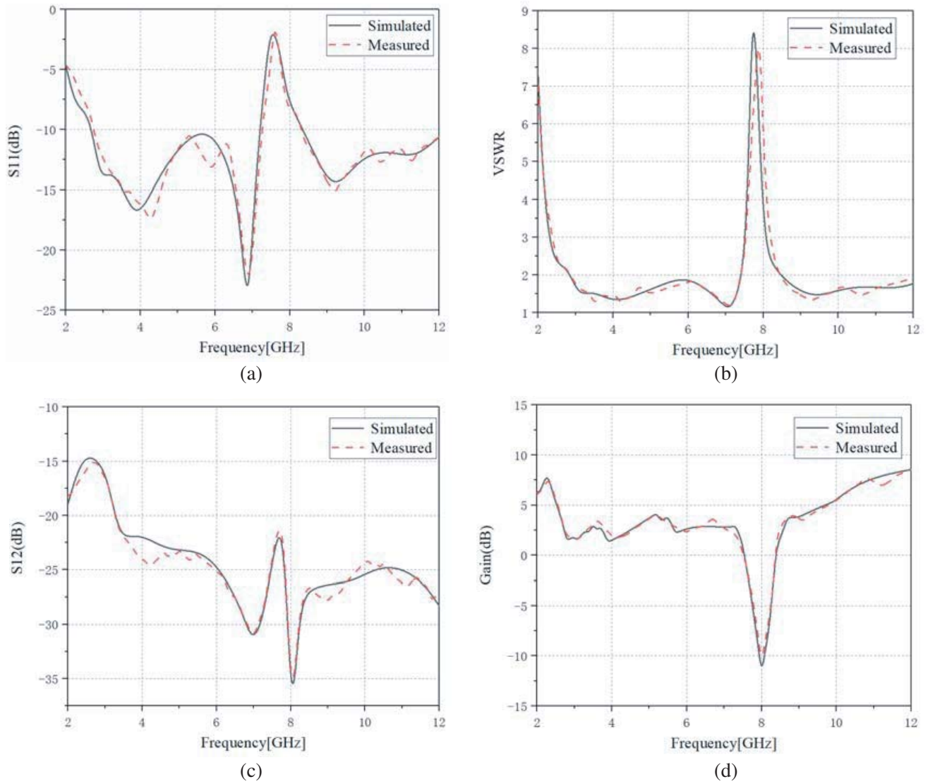
Figure 8. Simulated and measured of the proposed antenna, (a) S_{11} . (b) VSWR. (c) S_{12} . (d) Gain.
