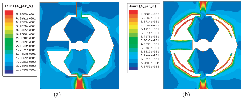
Figure 6. Surface current distribution of the proposed antennas.
