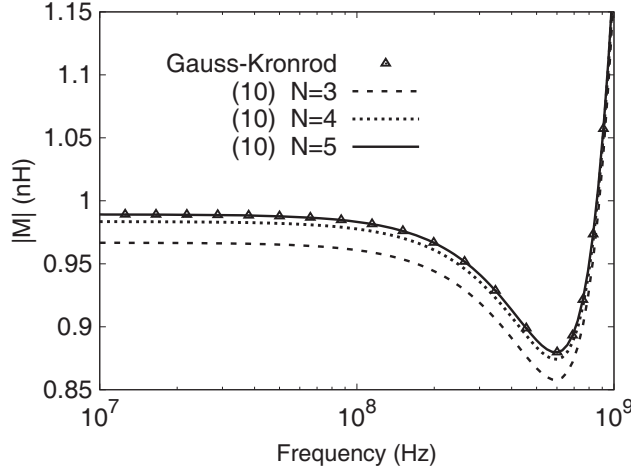
Figure 2. Mutual inductance between two loops with radius a=2 cm, computed against frequency.
