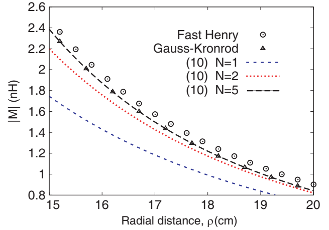
Figure 3. Mutual inductance between two loops with radius a=5 cm, computed against the radial distance \rho .
