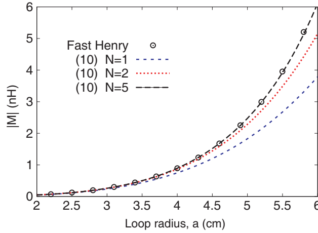
Figure 4. Mutual inductance between two loops separated by the distance \rho=15 cm, computed against the loop radius a .
