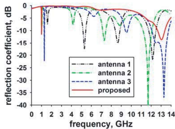
Figure 3. Harmonic suppression characteristics comparison for the four antenna structures in Figure 2.
