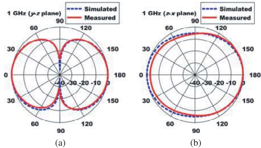
Figure 5. Measured radiation pattern at 1 GHz: (a) y - z plane, and (b) z - x plane.
