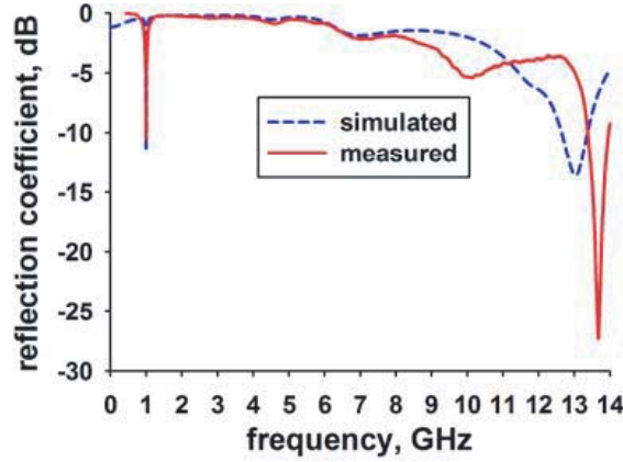
Figure 4. Comparison of simulated and measured reflection coefficient characteristics of the proposed antenna.
