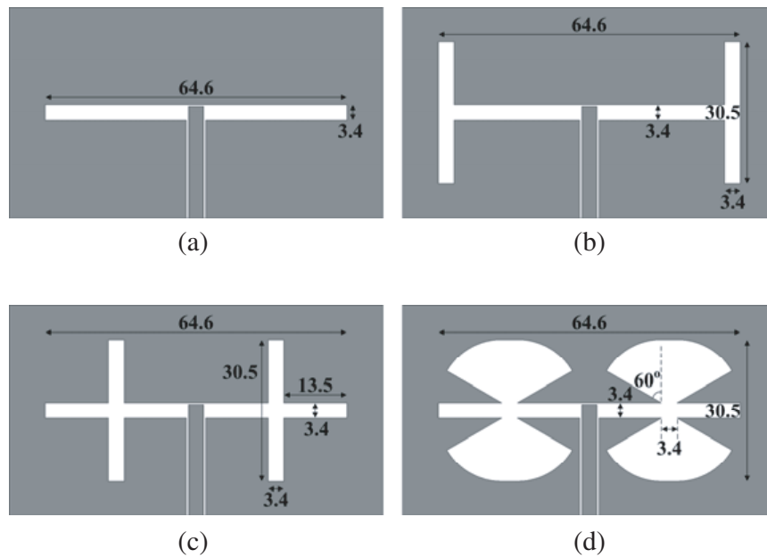
Figure 2. Geometries of four antennas considered in design procedure: (a) antenna 1, (b) antenna 2, (c) antenna 3, and (d) antenna 4.
