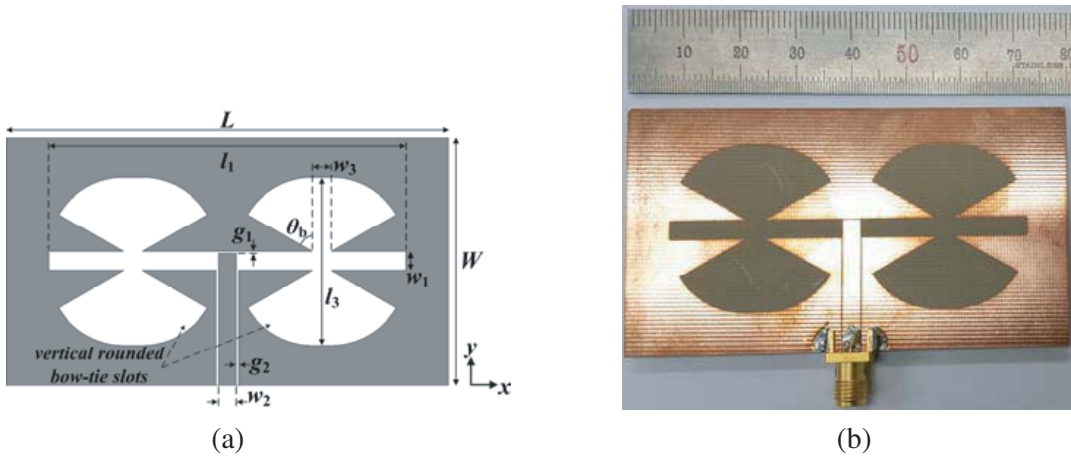
Figure 1. Configuration and fabricated prototype of proposed antenna: (a) configuration and (b) fabricated prototype.
