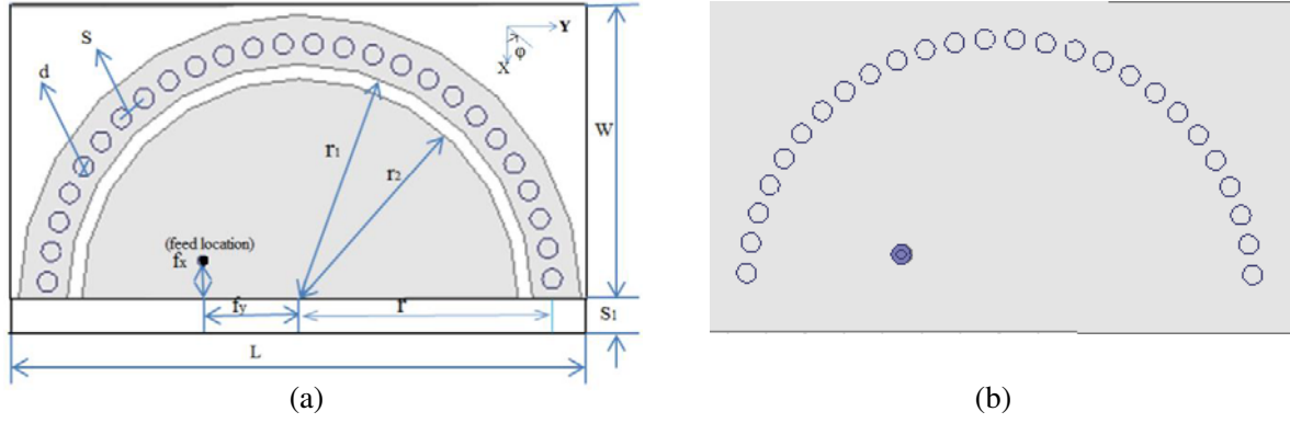
Figure 1. (a) Proposed antenna structure (top view). (b) Proposed antenna structure (bottom view).
