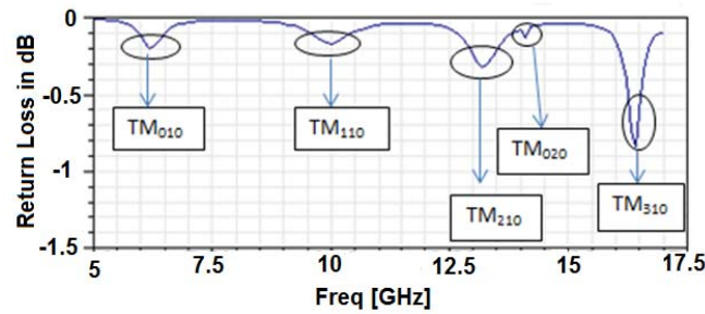
Figure 2. The simulated return loss of FMSIW cavity.
