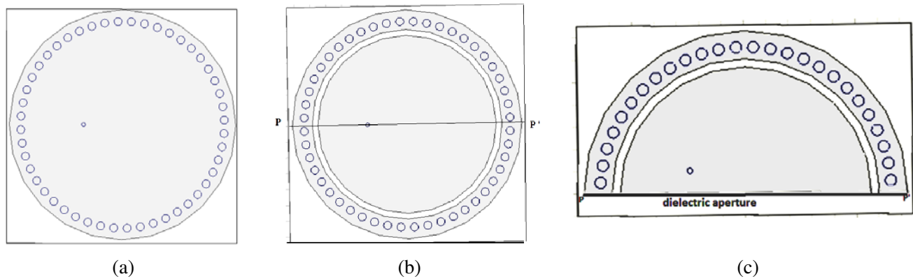
Figure 4. Design evolution: (a) FMSIW circular cavity. (b) FMSIW circular cavity with ring slot. (c) HMSIW cavity with slot (proposed design).
