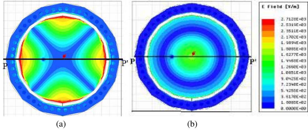
Figure 5. E -field distributions of FMSIW cavity with ring slot at (a) 8.5 GHz: TM_{210} . (b) 10.6 GHz: TM_{020} .
