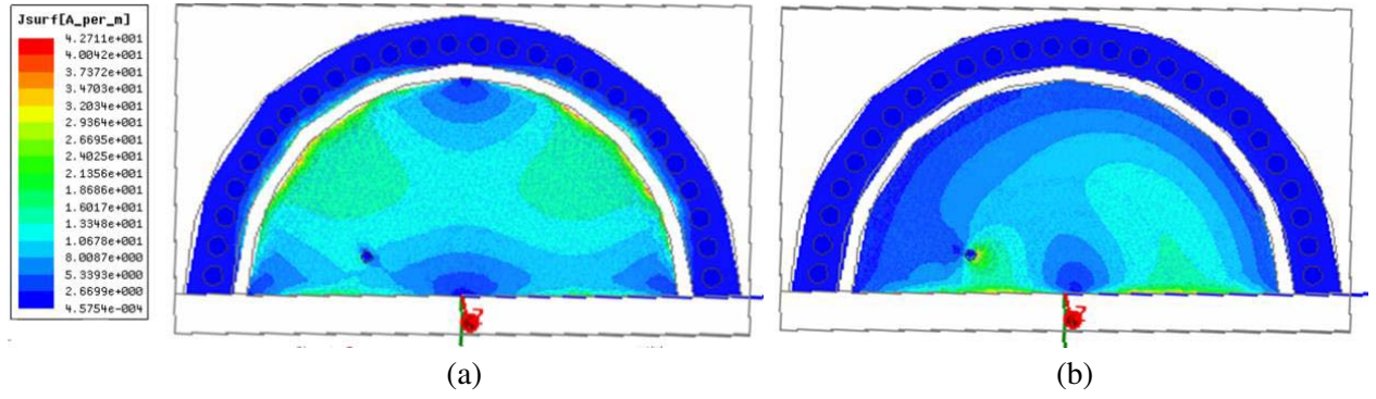
Figure 10. Surface current distribution at (a) 8.5 GHz and (b) 10.6 GHz.
