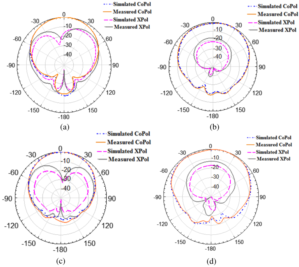
Figure 11. Simulated and measured (a) E -Plane ( \phi = 90^\circ ) pattern at 8.5 GHz (b) H -Plane ( \phi = 0^\circ ) pattern at 8.5 GHz (c) E -Plane ( \phi = 90^\circ ) Pattern at 10.6 GHz (d) H -Plane ( \phi = 0^\circ ) pattern at 10.6 GHz.
