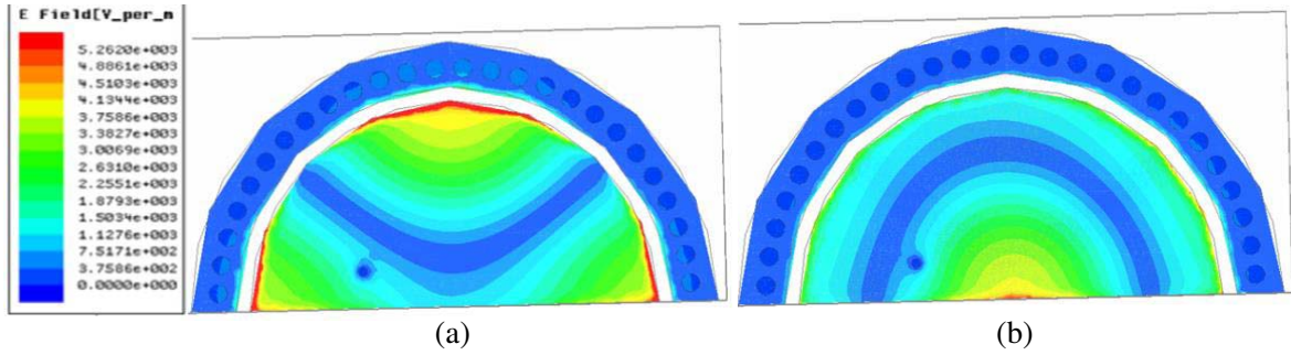
Figure 6. E -field distribution of proposed design at (a) 8.5 GHz: TM_{210} . (b) 10.6 GHz: TM_{020} .
