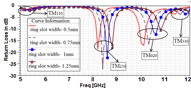
Figure 7. Simulated return loss for different slot width in HMSIW.
