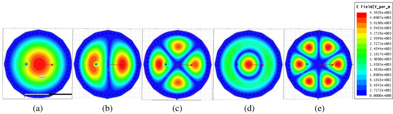
Figure 3. E -field distribution of FMSIW cavity at (a) TM_{010} Mode: 6.2 GHz. (b) TM_{110} Mode: 10 GHz. (c) TM_{210} Mode: 13.2 GHz. (d) TM_{020} Mode: 14.1 GHz. (e) TM_{310} Mode: 16.4 GHz.
