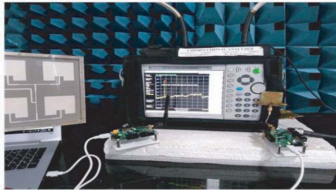
Figure 21. Transmitting data from fabricated antenna to CDAC Cmote.
