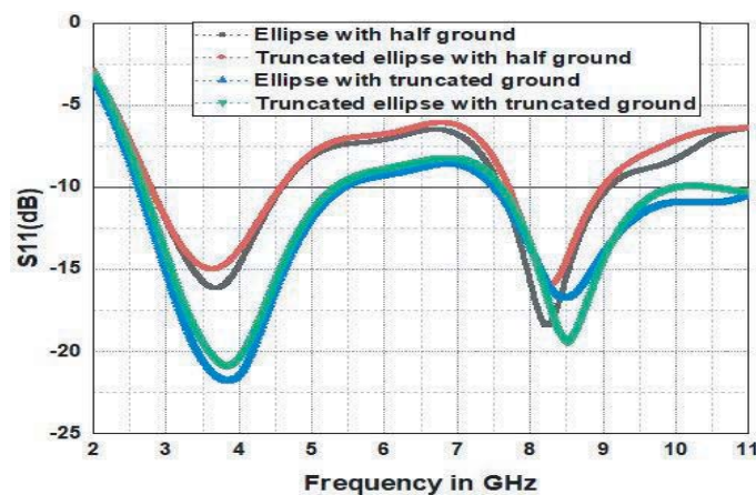
Figure 3. Reflection coefficients of the proposed monopole antennas.
