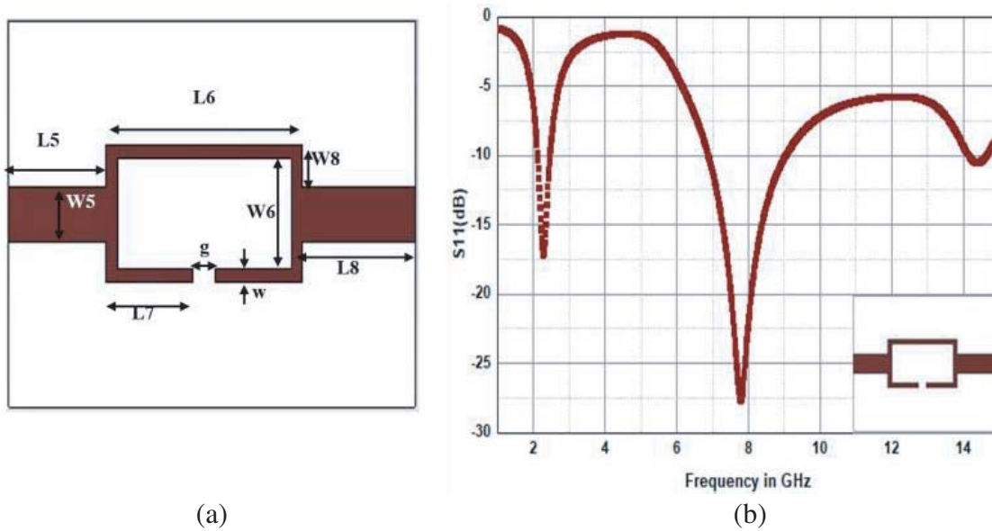
Figure 5. (a) Layout of the open loop filter. (b) Simulated S -parameters of open loop filter.
