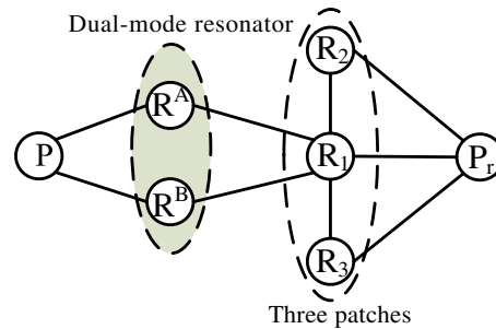
Figure 2. Coupling topologies of the proposed filtering antennas.
