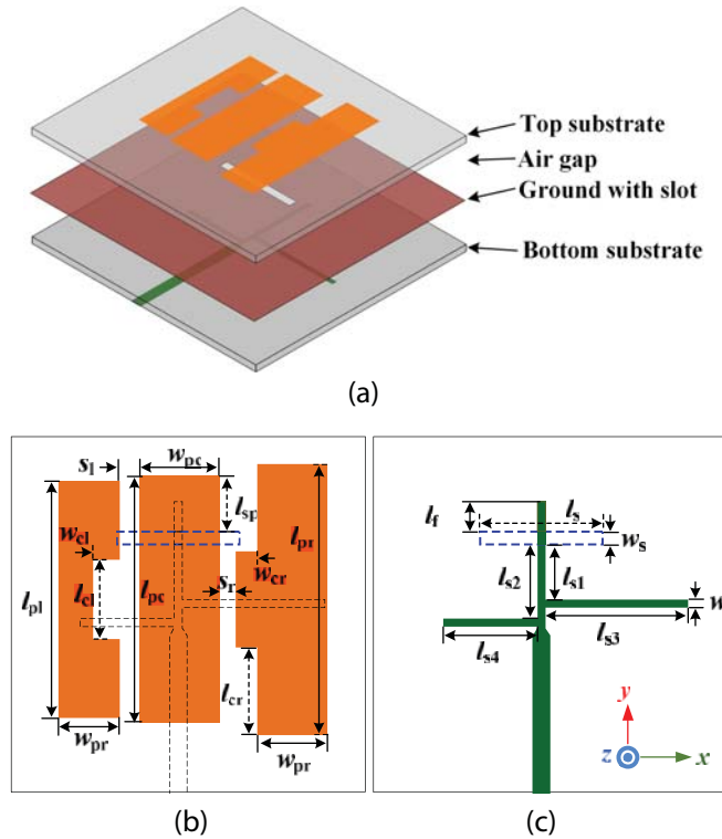
Figure 1. Structure of the proposed broadband filtering antenna. (a) Exploded view. (b) Top view. (c) Bottom view.
