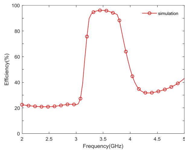
Figure 6. Simulated radiation efficiency of the proposed filtering antenna.
