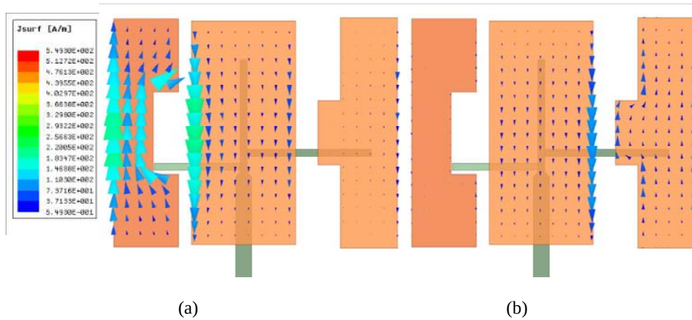
Figure 4. Current distributions at the frequencies of the first pair of gain zeros. (a) 3.2 GHz. (b) 3.8 GHz.
