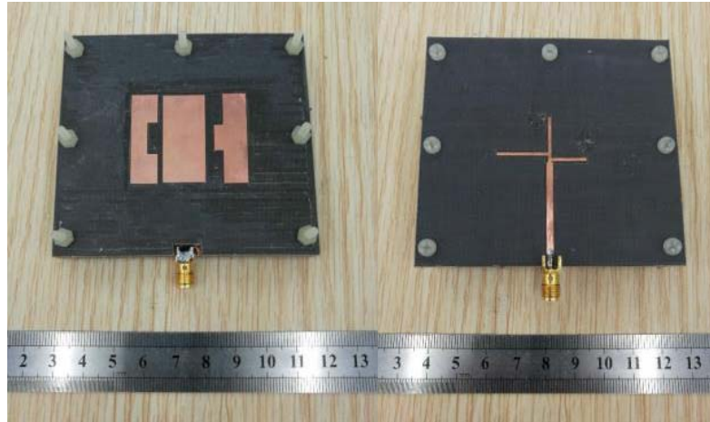
Figure 7. Photography of the proposed broadband filtering antenna.
