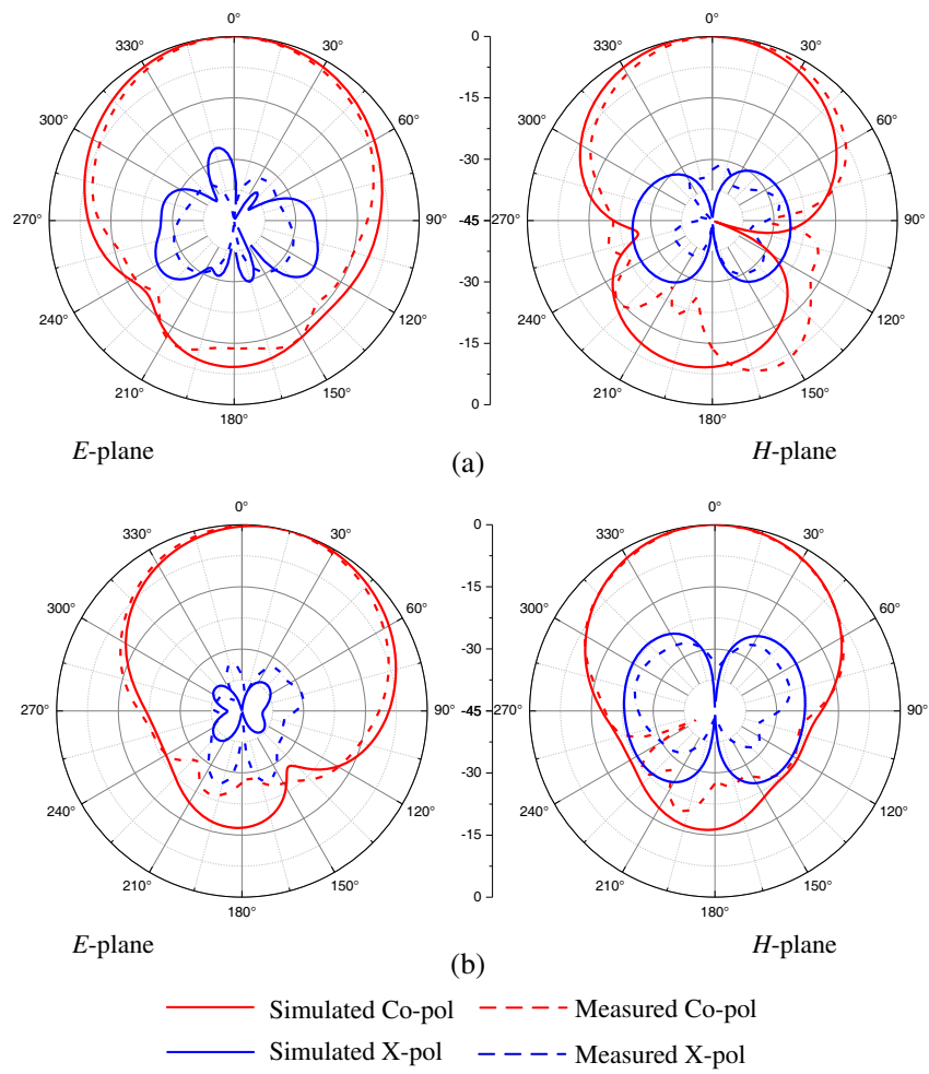
Figure 5. Normalized simulated and measured radiation patterns of the proposed filtering antenna at (a) 3.4 GHz. (b) 3.6 GHz.
