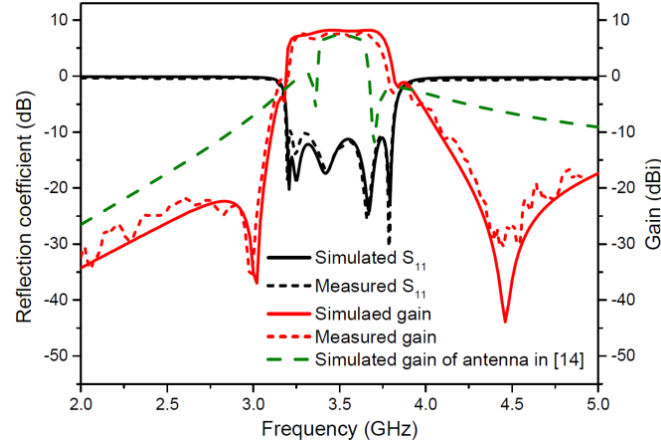
Figure 3. Simulated and measured reflection coefficients and gains of the proposed filtering antenna.
