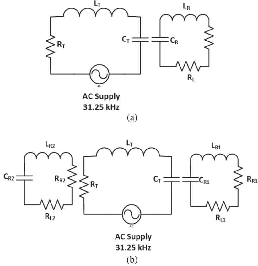
Figure 3. (a), (b) Equivalent circuit models of RIC-WPT system for single and multiple loads.
