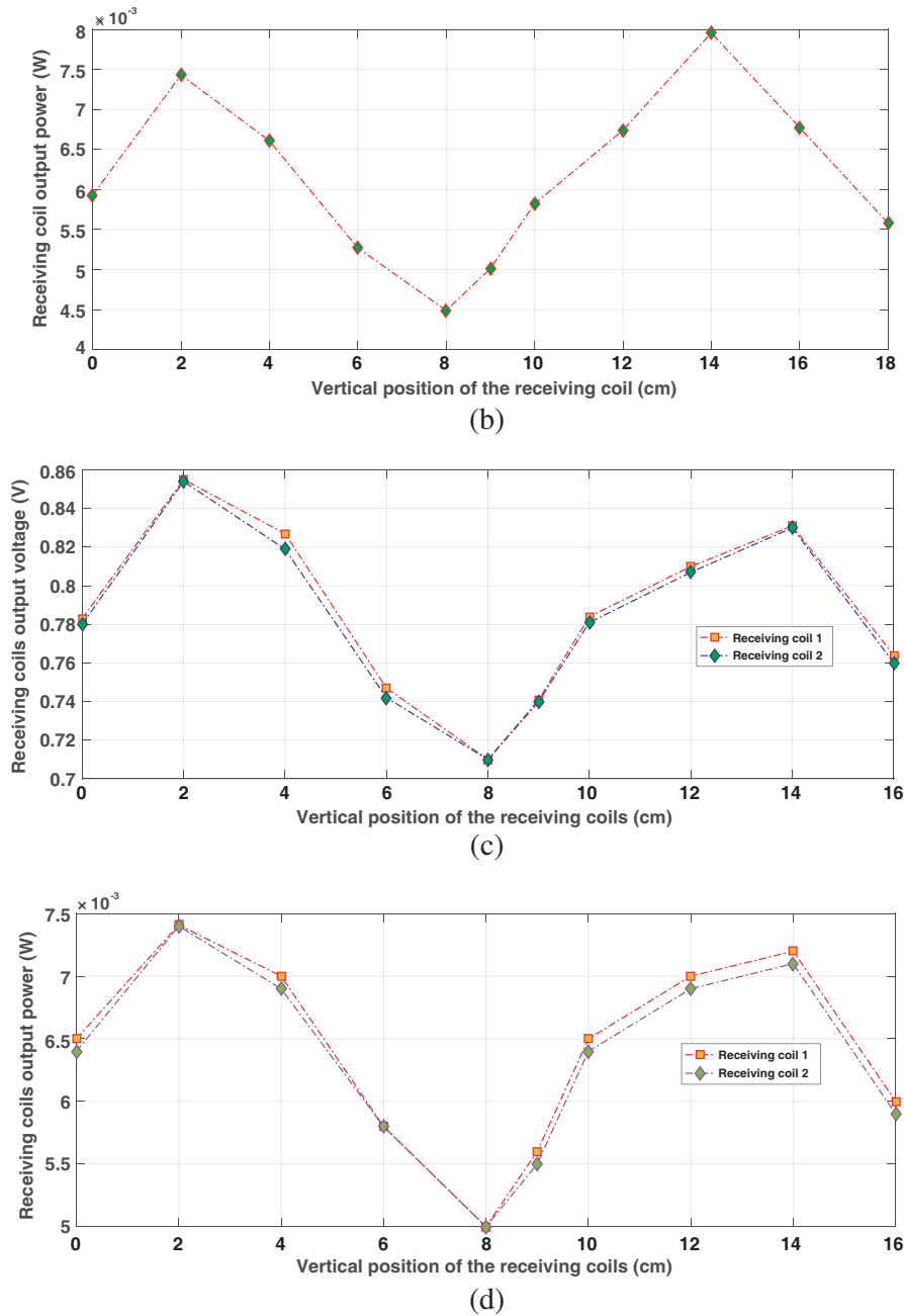
Figure 5. (a)–(d) Variation of the load voltage and the power transfer to the load in single as well as in two-loads corresponding to the position of the receiving coil.
