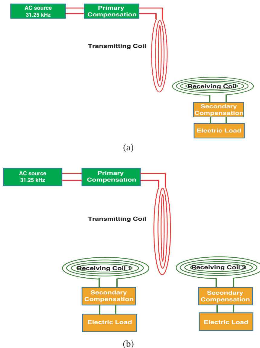
Figure 1. (a), (b) Experimental setup block diagram of RIC-WPT system for single load and multiple loads respectively.
