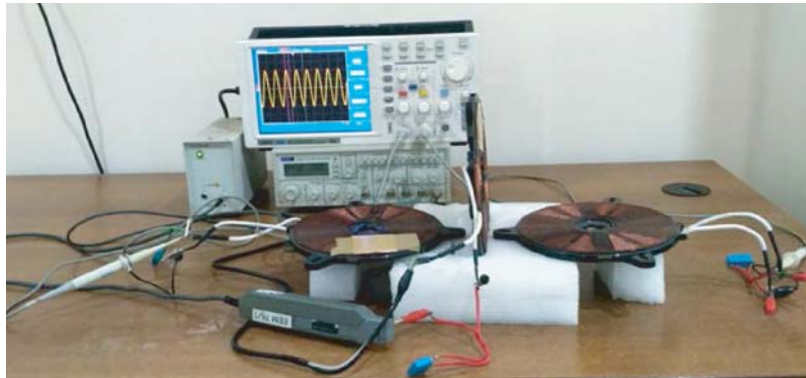
Figure 2. Experimental setup of RIC-WPT system for multiple loads.
