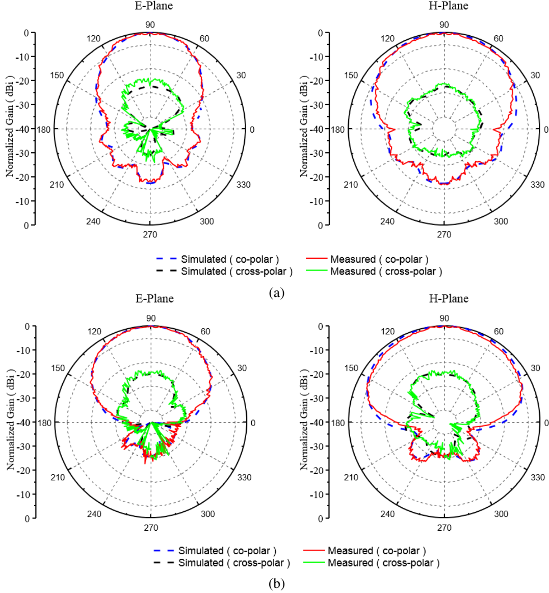
Figure 9. Simulated and measured radiation patterns of the filtering antennas. (a) Filtering antenna I. (b) Filtering antenna II.
