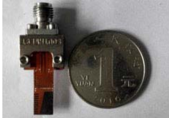
Figure 7. Photograph of the fabricated filtering antenna.
