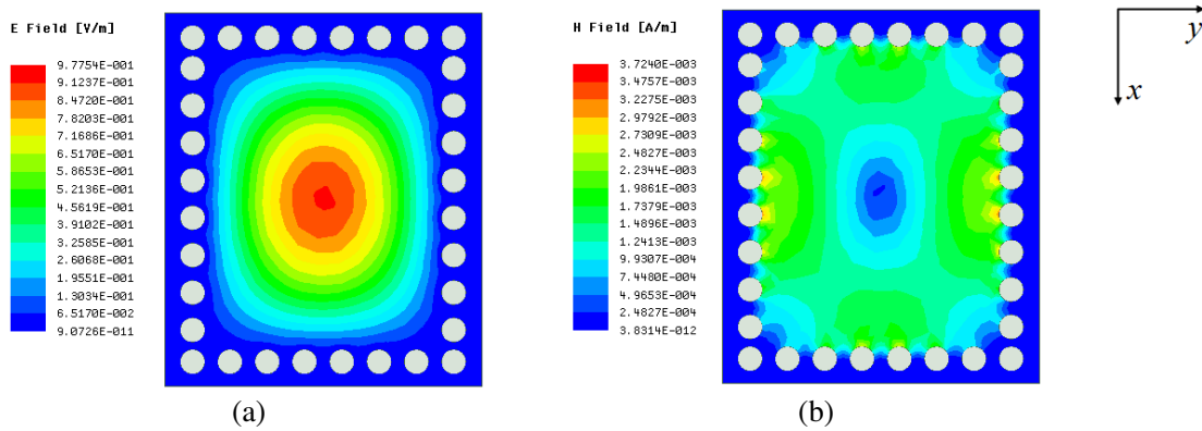
Figure 2. The field distributions of TE_{101} mode in a rectangular SIW cavity. (a) E -field. (b) H -field.
