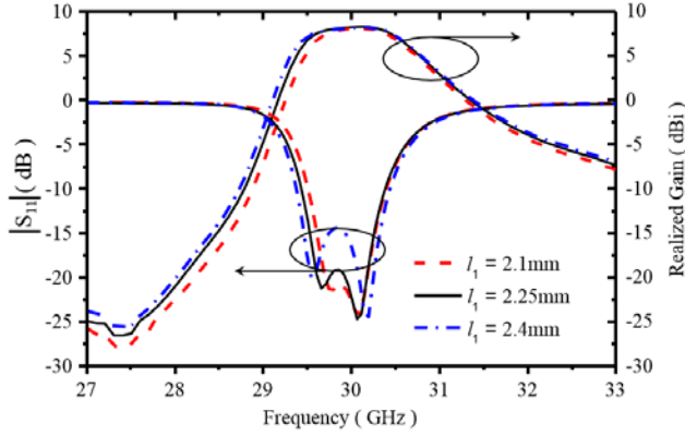
Figure 3. Simulated reflection coefficients and realized gains of the filtering antenna I with different values of l_1 .
