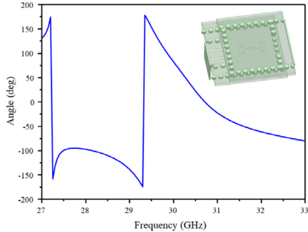
Figure 5. Simulated phase curve of S_{21} of the filtering structure in filtering antenna I.
