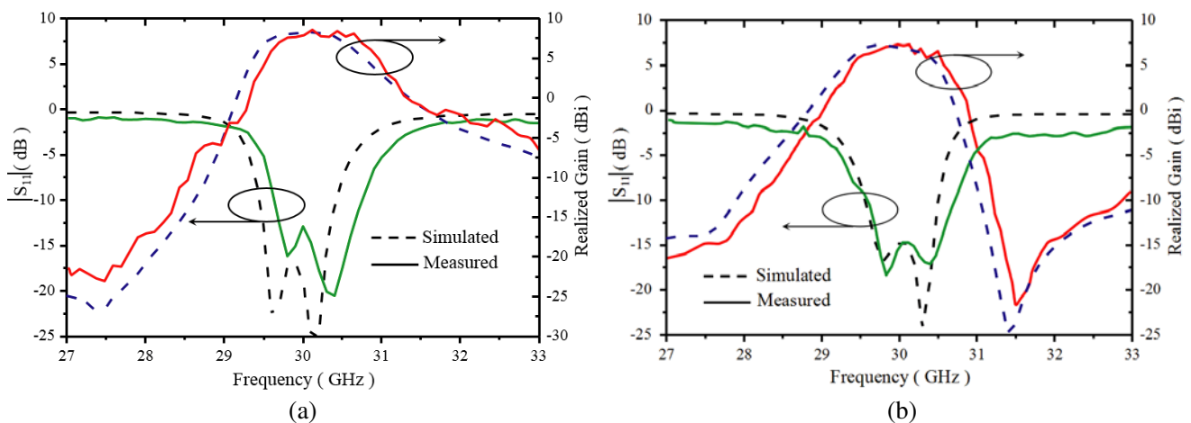
Figure 8. Simulated and measured reflection coefficients and realized gains of the filtering antennas. (a) Filtering antenna I. (b) Filtering antenna II.
