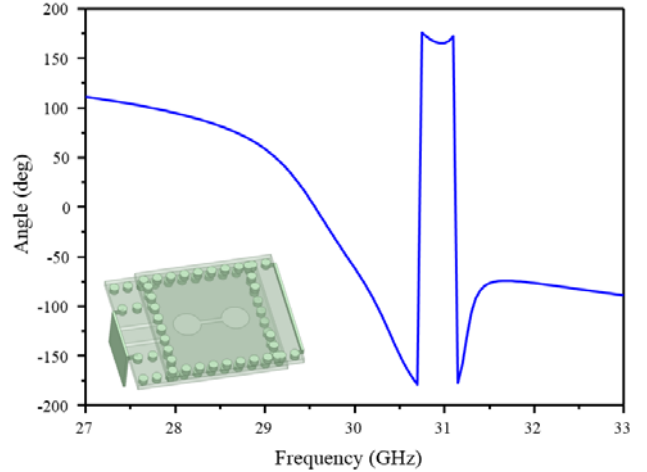
Figure 6. Simulated phase curve of S_{21} of the filtering structure in filtering antenna II.
