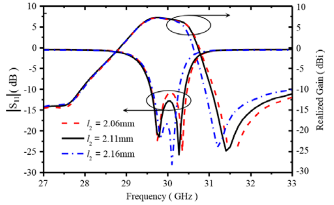
Figure 4. Simulated reflection coefficients and realized gains of the filtering antenna II with different values of l_2 .
