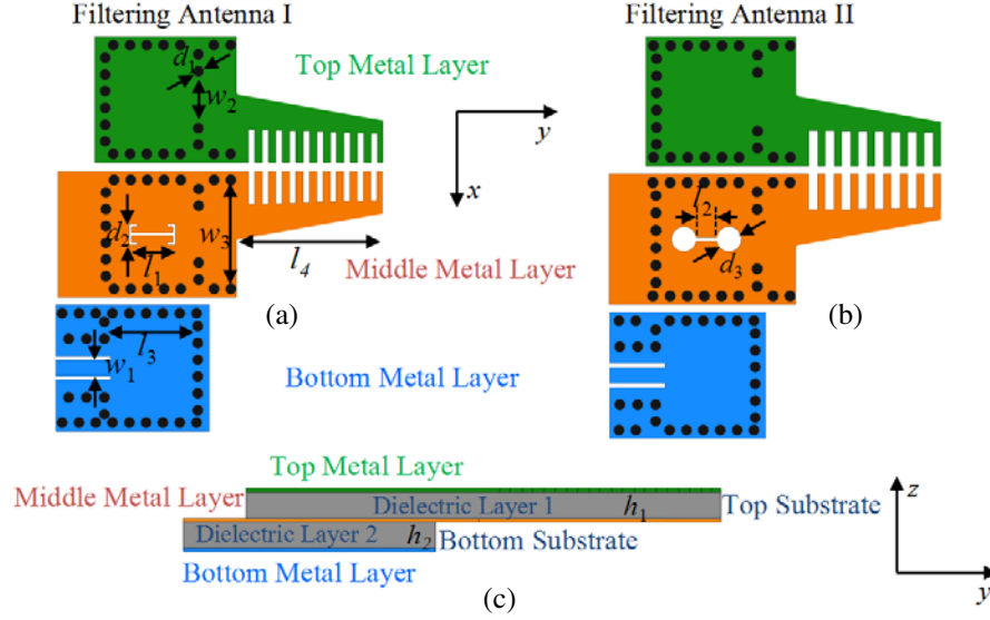
Figure 1. Geometry of the proposed type of vertically stacked SIW filtering antenna.
