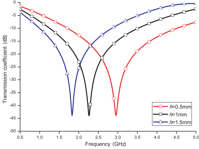
Figure 3. Simulated transmission coefficients of the proposed UMEFSS with different thicknesses of the substrate.
