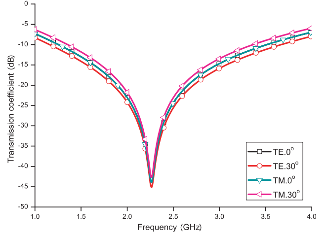
Figure 4. Simulated transmission coefficients of the proposed UMEFSS with different incident angles at different polarisations.
