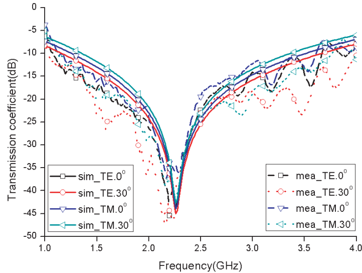
Figure 6. Simulated and measured transmission coefficients of the proposed UMEFSS with different incident angles at different polarisations.
