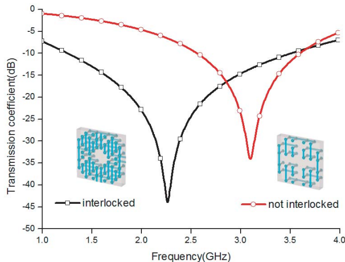
Figure 2. Simulated transmission coefficients of the FSS without interlocked structures and the proposed UMEFSS.
