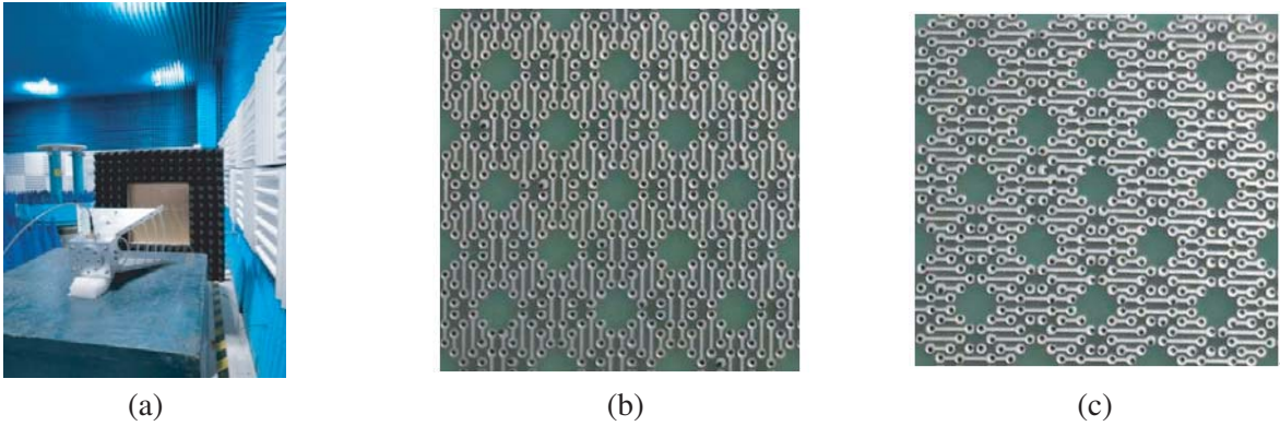
Figure 5. Photographs of measurement environment and fabricated FSS: (a) measurement environment, (b) 3 \times 3 unit cells of the fabricated FSS (top view), (c) 3 \times 3 unit cells of the fabricated FSS (bottom view).
