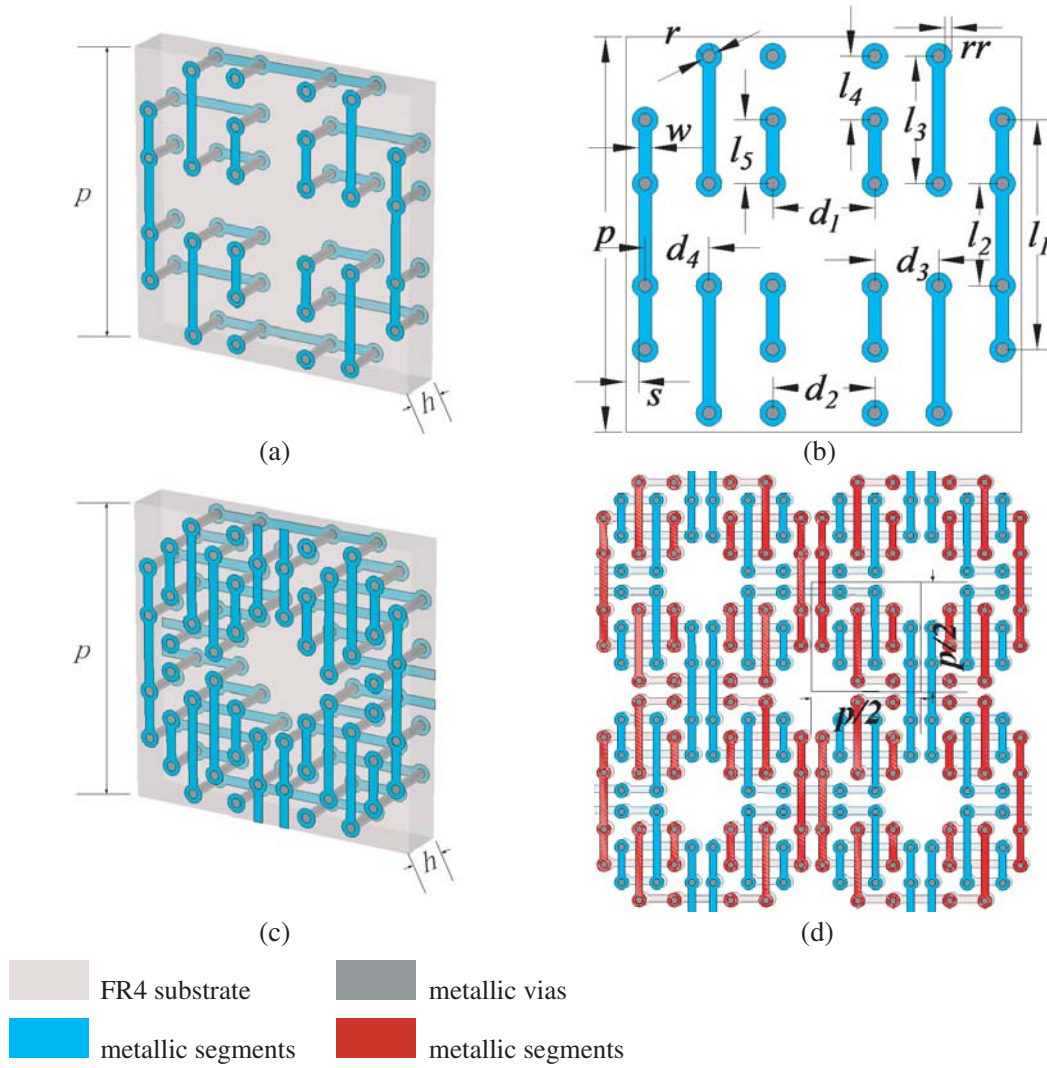
Figure 1. Geometric configuration of the proposed UMEFSS: (a) 3D view of basic element, (b) upper layer of basic element, (c) 3D view of unit cell, (d) 2 \times 2 unit cells of the proposed UMEFSS. ( p = 6.2 mm, h = 1 mm, w = r = 0.2 mm, s = 0.2 mm, rr = 0.13 mm, l_1 = 3.6 mm, l_2 = 1.6 mm, l_3 = 2 mm, l_4 = l_5 = 1 mm, d_1 = d_2 = 1.6 mm, d_3 = d_4 = 1 mm).
