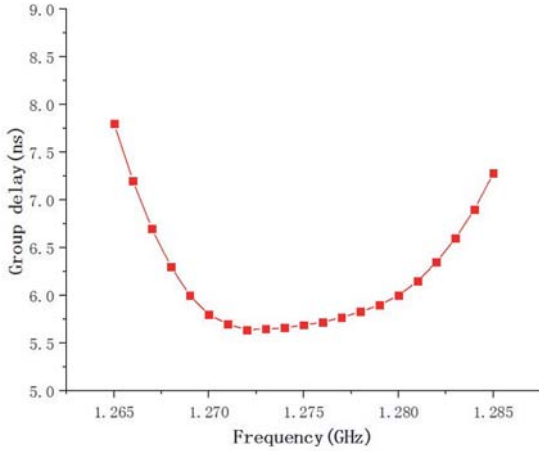
Figure 13. Passband group delay results of the filter.
