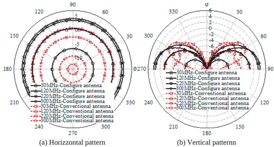
Figure 11. Radiation patterns of configure antenna.
