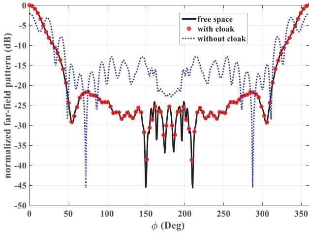
Figure 6. The far-field pattern produced by antenna 1 at 10.5 GHz for three cases: 1) Antenna 1 radiating in free space. 2) Antenna 1 radiating in the presence of the loop-type antenna (antenna 2). 3) Antenna 2 is covered by the proposed cloak.
