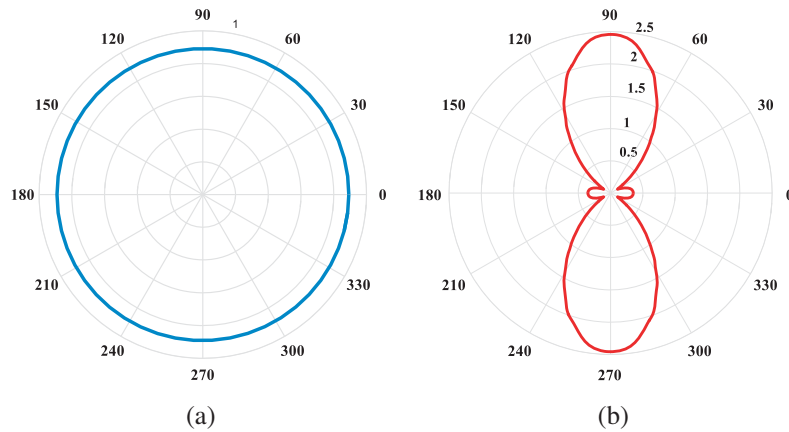
Figure 4. Far-field pattern at 3.5 GHz of (a) loop antenna in free space and (b) loop antenna covered with the proposed material.
