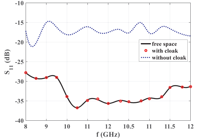
Figure 7. The S -parameter of the horn antenna for three cases illustrated in Fig. 6.
