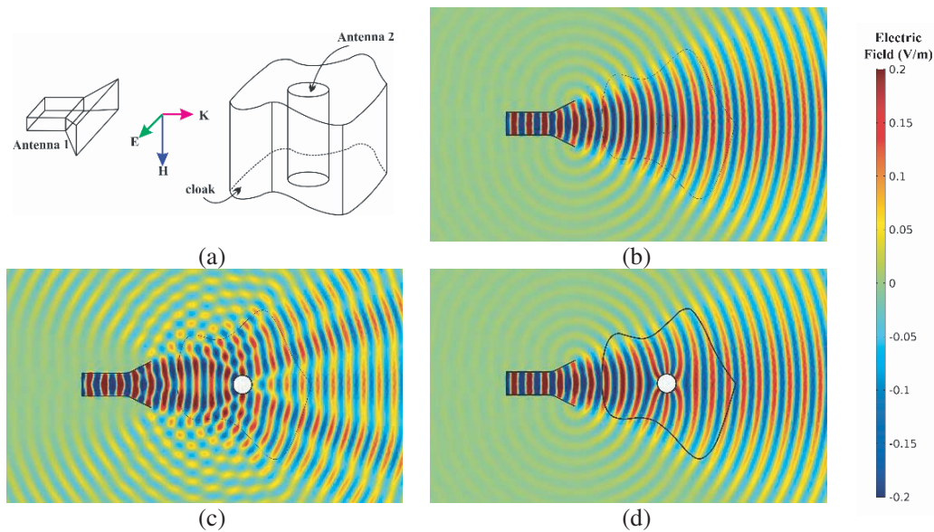
Figure 5. The electric field distribution radiated by the horn antenna at 10.5 GHz (antenna 1): (a) the schematic of multiple antenna environment and the proposed method for coupling reduction. (b) Radiating fields from antenna 1 in free space. (c) Radiating fields from antenna 1 in the presence of loop-type antenna (antenna 2). (d) Antenna 2 is covered by the proposed layer.
