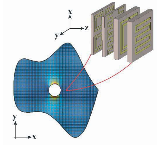
Figure 8. Discretization of the desired permeability to achieve locally homogeneous materials with the proposed meta-atom consists of SRR-meander line array.
