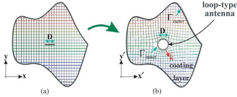
Figure 1. Schematic diagram of coordinate transformation using quasi-conformal mapping. (a) Virtual space; (b) Physical space.
