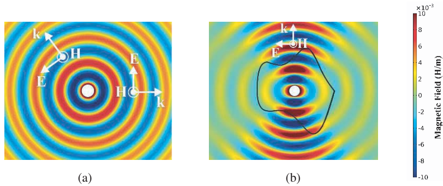
Figure 3. The magnetic field distribution at 3.5\text{ GHz} for (a) loop antenna in free space and (b) loop antenna covered with the proposed material.
