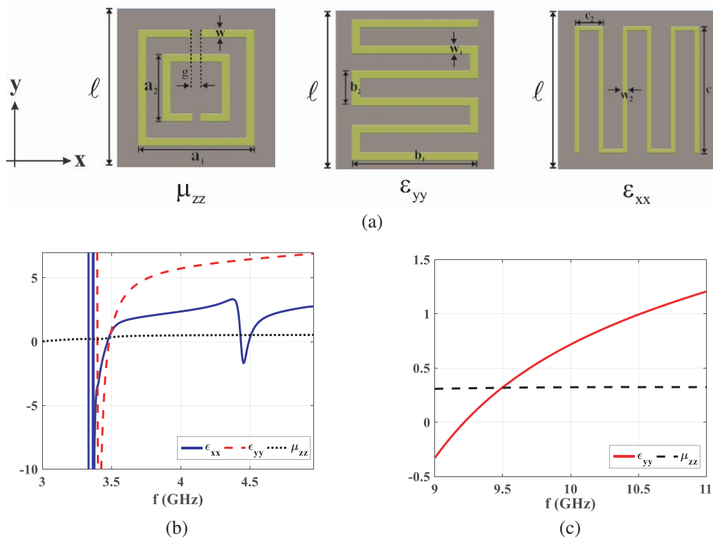
Figure 9. (a) The metamaterial unit-cell geometry with parameters of \ell = 8.2 mm, a_1 = 6.6 mm, a_2 = 5 mm, w = 0.4 mm, g = 0.4 mm, b_1 = 5.9 mm, b_2 = 1.5 mm, w_1 = 0.4 mm, c_1 = 5.6 , c_2 = 1.6 mm, w_2 = 0.35 mm for f = 3.5 GHz and \ell = 4.1 mm, a_1 = 3.3 mm, a_2 = 2.3 mm, w = 0.2 mm, g = 0.2 mm, b_1 = 1.94 mm, b_2 = 0.95 mm, w_1 = 0.2 mm for f = 10.5 GHz. (b), (c) The retrieved material parameters.
