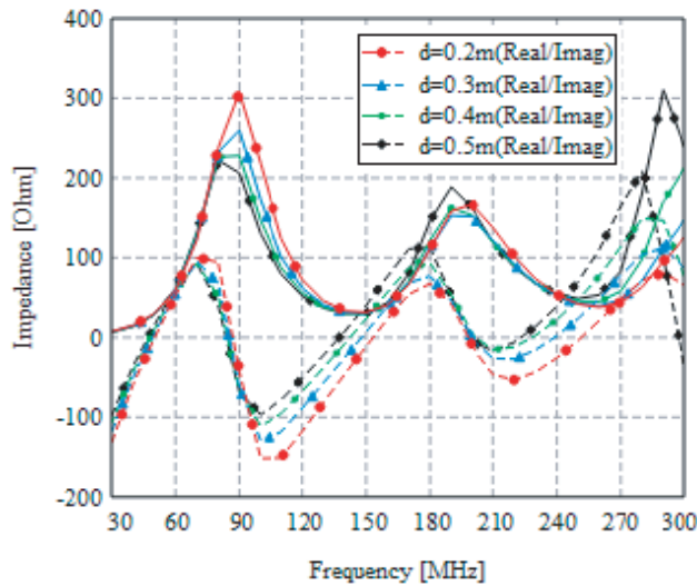
Figure 3. Input impedance of double-whip antenna with different d .
