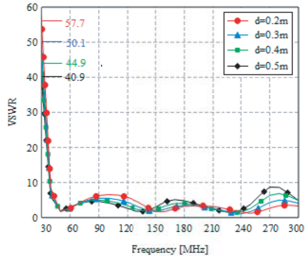
Figure 4. The VSWR of double-whip antenna with different d .
