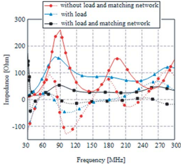
Figure 7. Comparison of input impedance before and after optimization.
