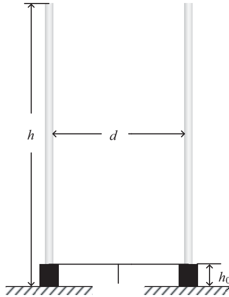
Figure 1. Diagram of a double-whip antenna.
