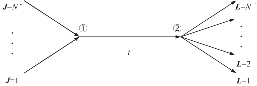
Figure 2. The wiring segment contained in the i -th basis function.
