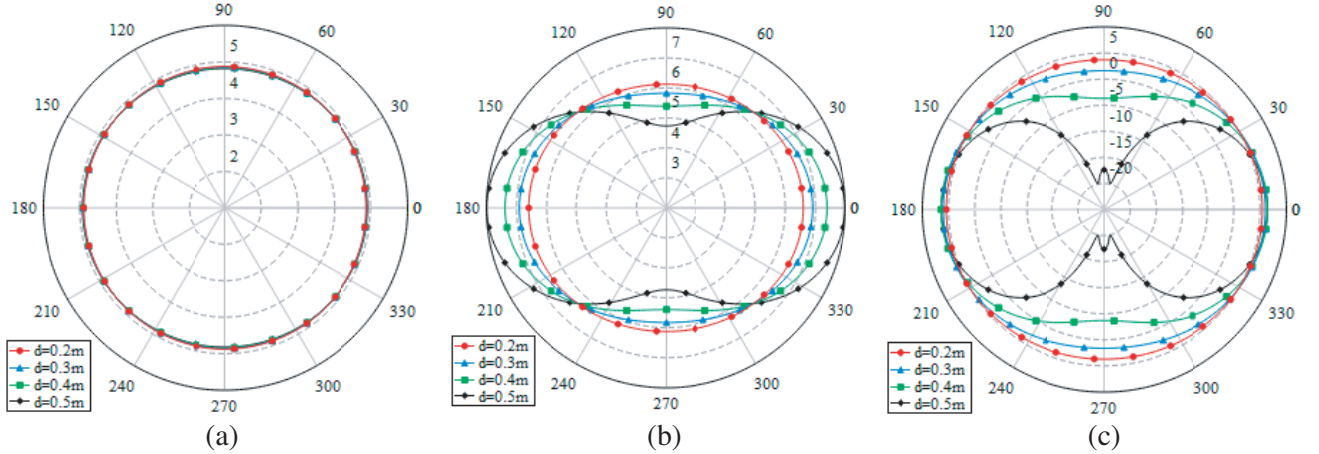
Figure 5. Horizontal pattern of double-whip antenna at different spacing, (a) 3 MHz, (b) 15 MHz, (c) 300 MHz.
