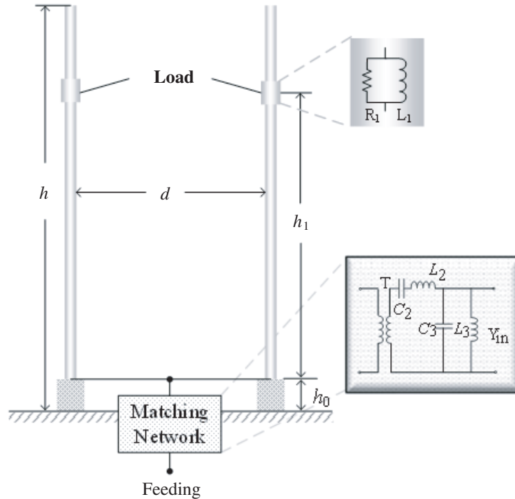
Figure 6. The proposed double-whip antenna structure.
