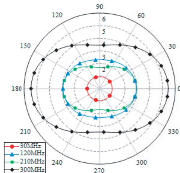
Figure 11. The pattern of the proposed double-whip antenna.
