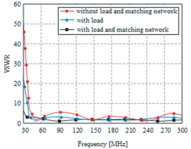
Figure 8. Comparison of VSWR before and after optimization.
