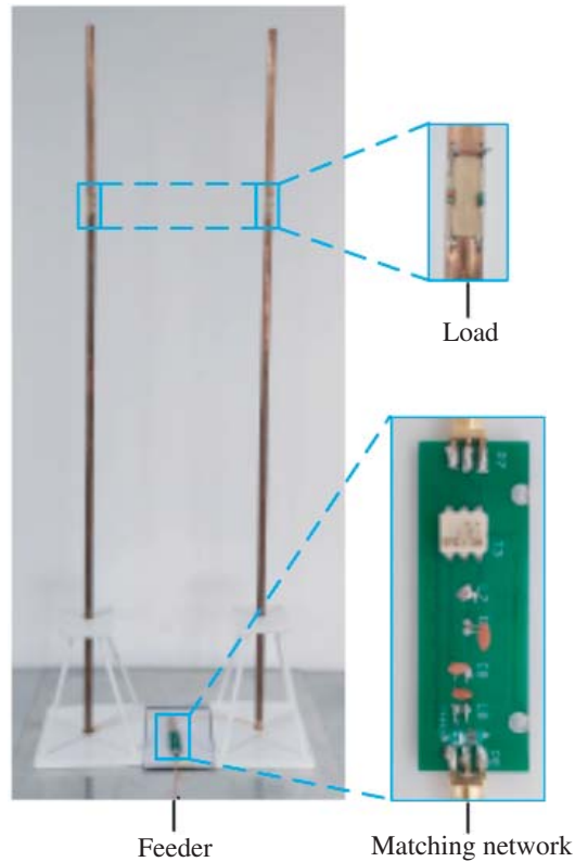
Figure 9. The fabricated prototype of the proposed antenna.
