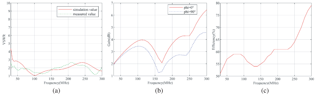
Figure 10. Performance curves of the proposed double-whip antenna. (a) VSWR. (b) Gain. (c) Efficiency.
