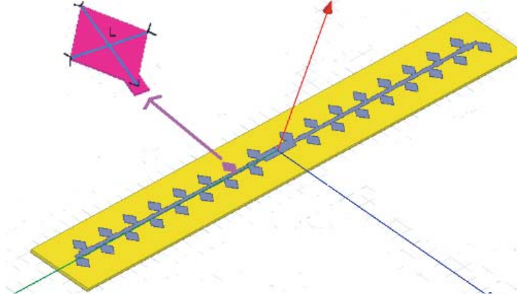
Figure 1. Single in line antenna array with 32 elements.
