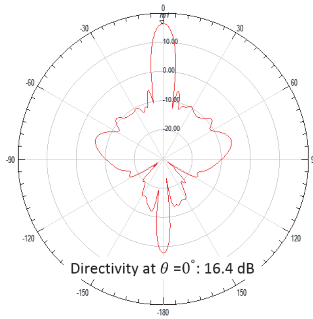
Figure 2. The single-line antenna directivity in plane of \varphi = 0^\circ .
