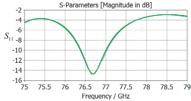
Figure 7. The simulated S_{11} for the final antenna array.
