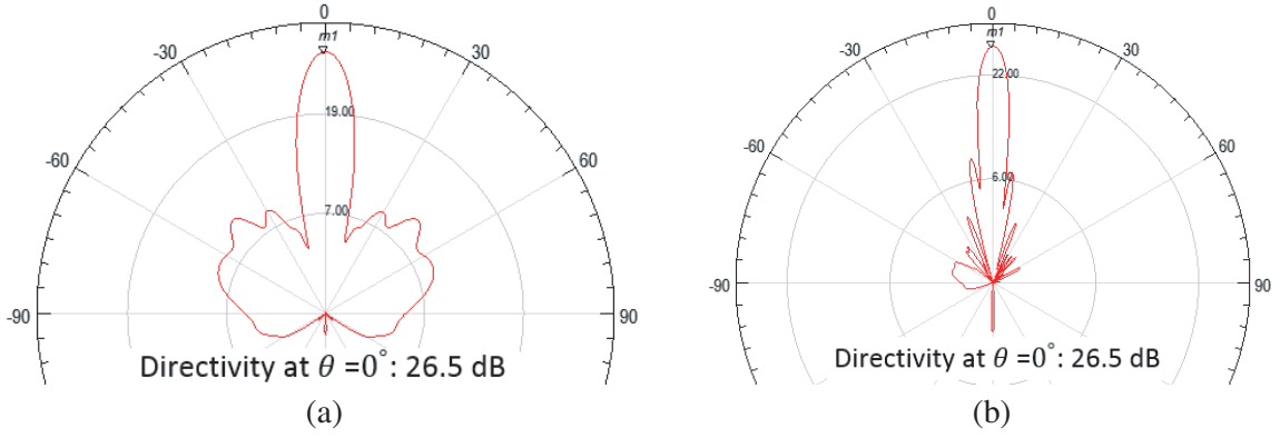
Figure 3. Two-dimensional antenna radiation pattern. (a) H -plane. (b) E -plane.
