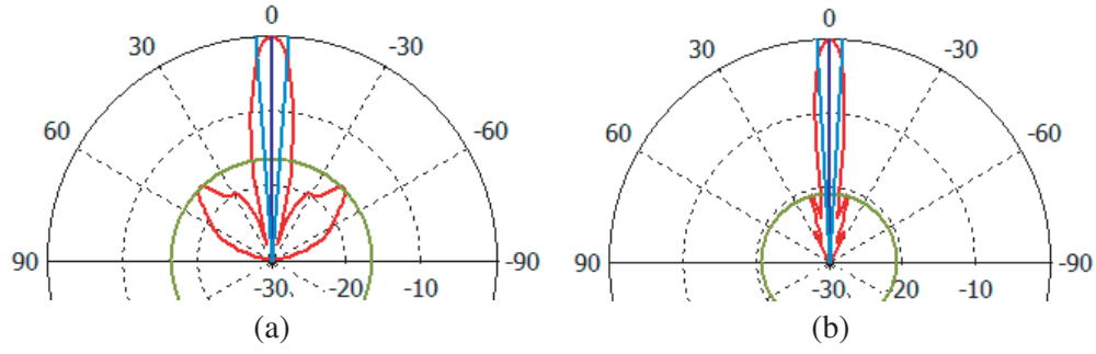
Figure 6. The directivity radiation pattern of the final antenna at 76.8 GHz. (a) H -plane. (b) E -plane.
