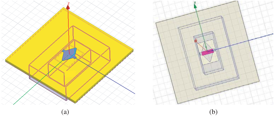
Figure 4. The antenna waveguide feed and its matching element. (a) Antenna waveguide feed structure. (b) Matching element of the waveguide feed.
