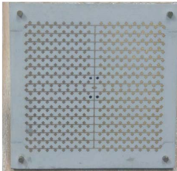
Figure 8. The photograph of the fabricated antenna.
