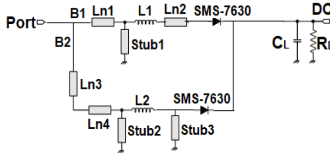
Figure 7. Schematic of the dual band rectifier. ( Ln1 = 6.2 mm, Ln2 = 2 mm, Ln3 = 3.5 mm, Ln4 = 3.5 mm, Stub 1 = 2.9 mm, Stub 2 = 8.1 mm, Stub 3 = 6.1, L1 = 5.6 , L2 = 1.6 nH, W_{\text{Stub}} = 2,38 mm, R_L = 0.5 k \Omega ).
