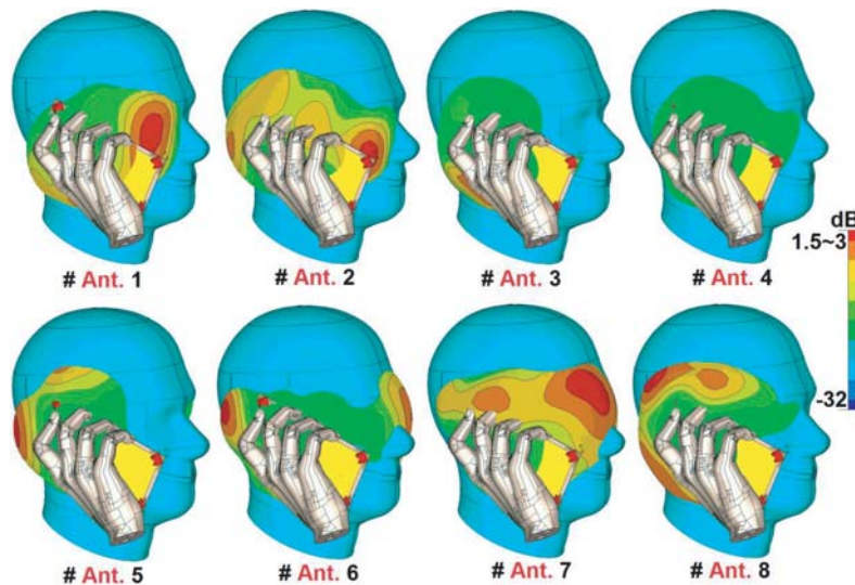
Figure 14. Radiation patterns at 3.5 GHz in Talk-Mode.
