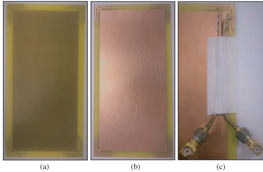
Figure 8. (a) Front (b) back views of the prototype sample, and (c) the feeding mechanism for two PIFAs.
