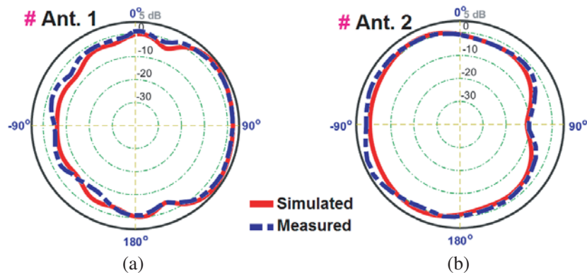
Figure 10. 2D polar radiation patterns at 3.5 GHz for Ports (a) 1 and (b) 2.
