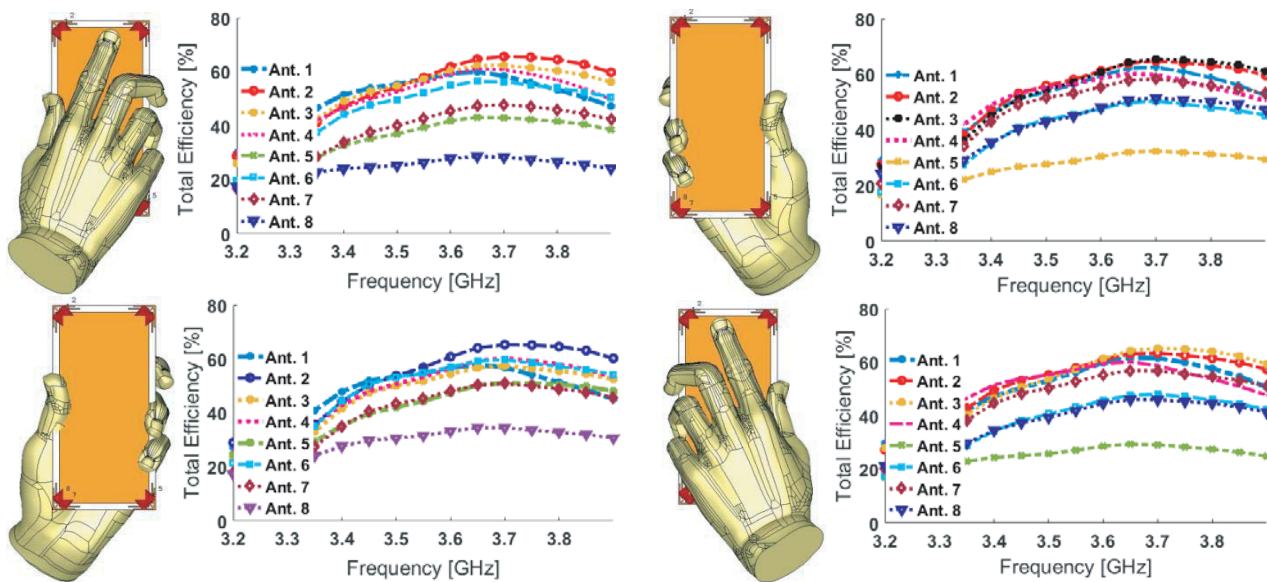
Figure 12. Placement and efficiencies of the PIFA array at different user-hand scenarios.
