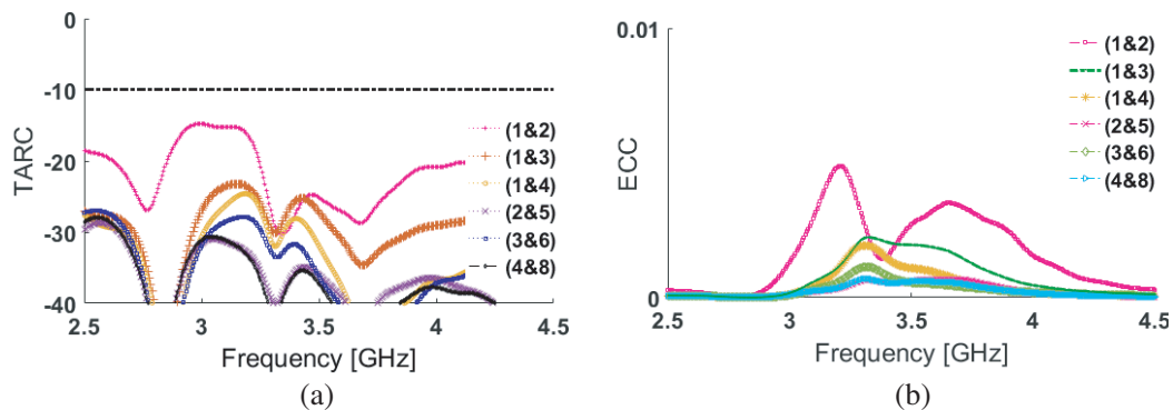
Figure 7. Calculated (a) TARC, (b) ECC results.
