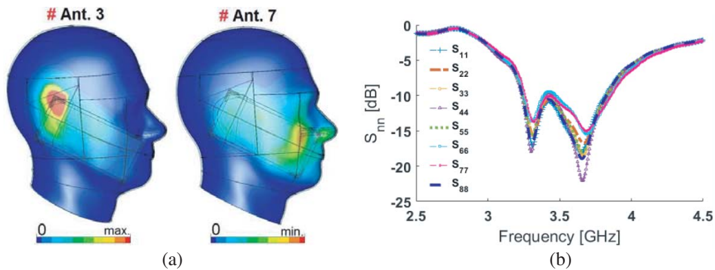
Figure 13. (a) SAR and (b) reflection coefficients in Talk-Mode.
