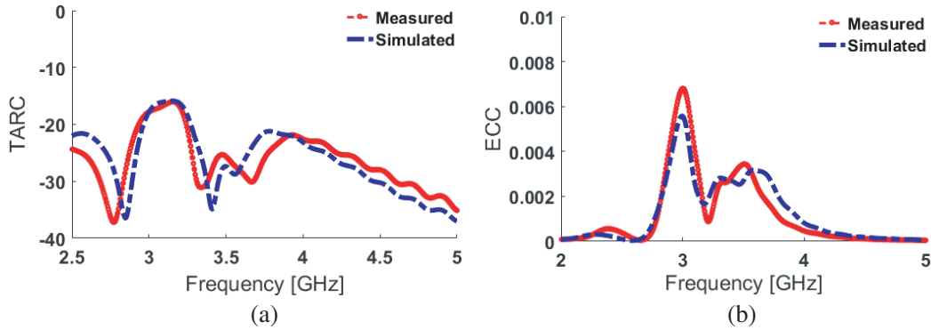
Figure 11. Calculated (a) TARC, (b) ECC results of the adjacent elements.
