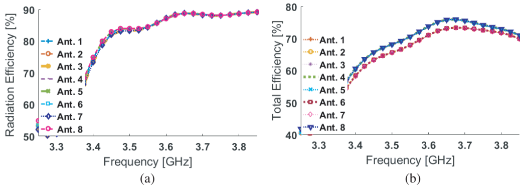
Figure 6. (a) Radiation and (b) total efficiencies of the MIMO design.
