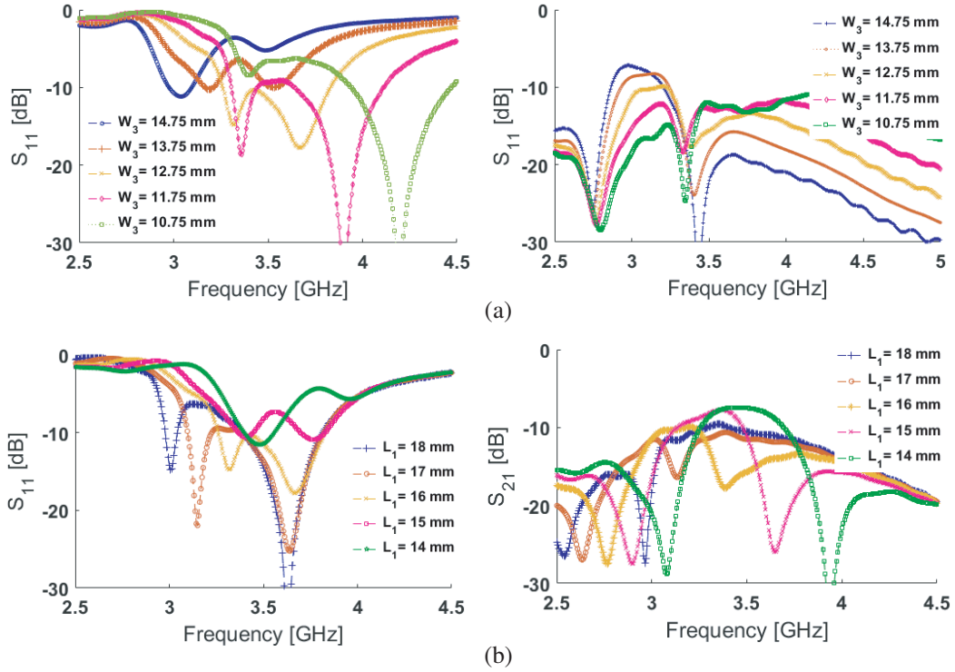
Figure 3. S_{11}/S_{21} results for different values of (a) W_2 and (b) L_2 .
