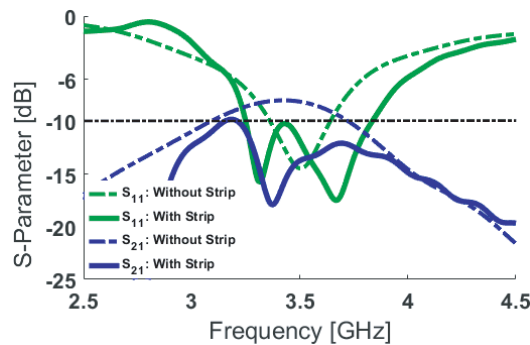
Figure 2. S_{11}/S_{21} of adjacent elements with/without the arrow-strip.
