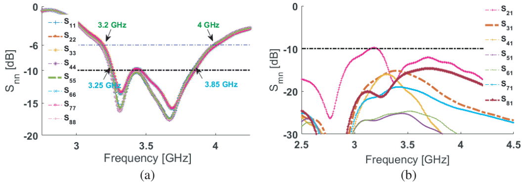
Figure 4. Simulated (a) S_{nn} and (b) S_{mn} of the array S -parameters.
