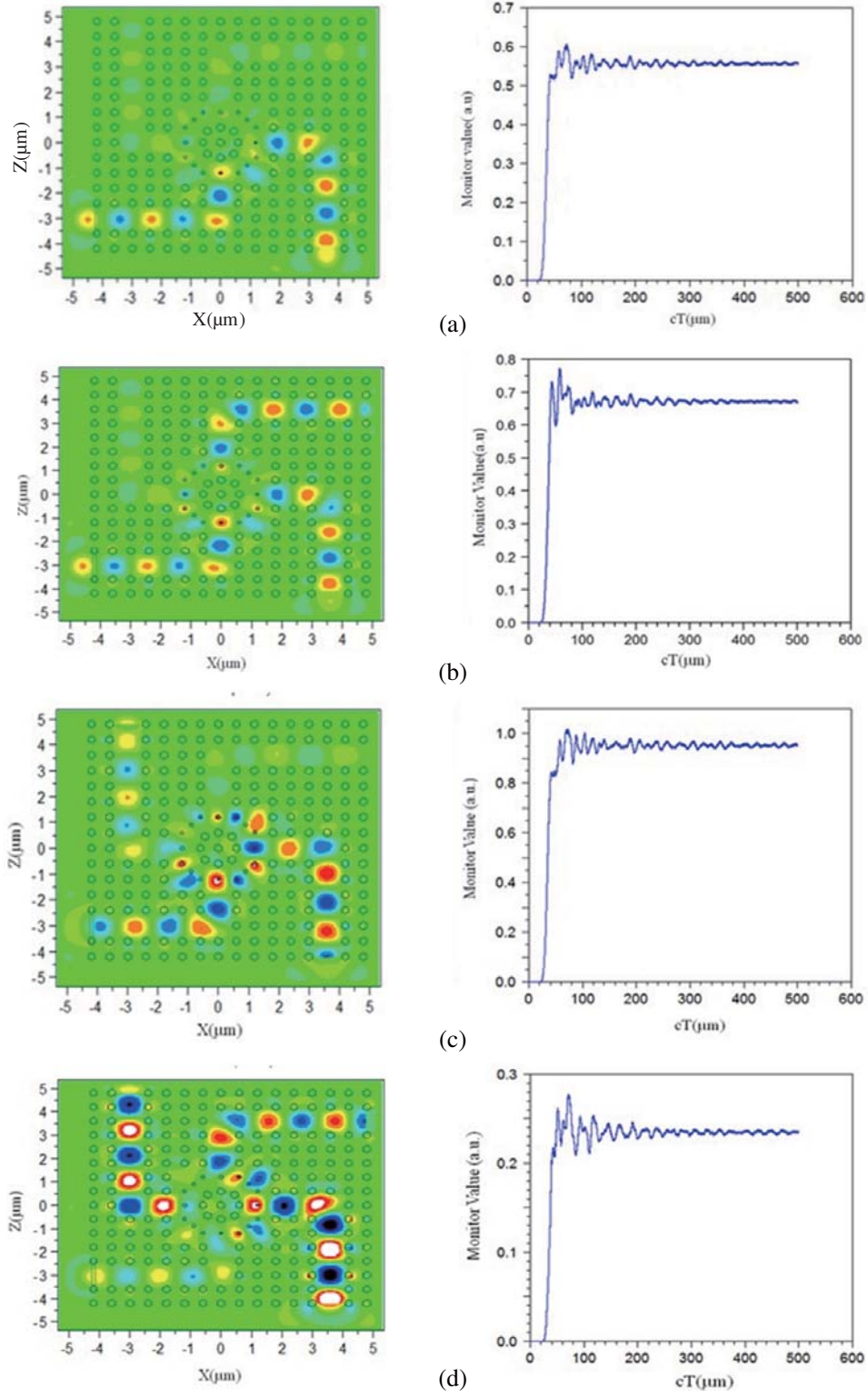
Figure 3. Transmission diagram and output power for the optical NAND gate. (a) A = 0, B = 0, CI = 1 , (b) A = 0, B = 1, CI = 1 , (c) A = 1, B = 0, CI = 1 , (d) A = 1, B = 1, CI = 1 .
