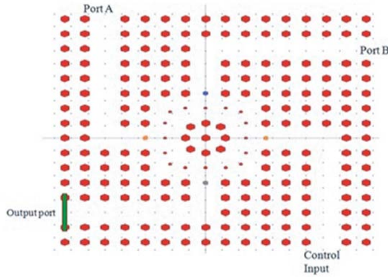
Figure 4. Proposed structure for optical NOR gate.
