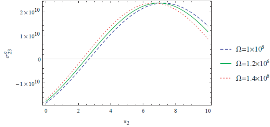
Figure 7. Variation of the shear stress \sigma_{23}^c in the core layer given in Eq. (21) with variation of rotation.
