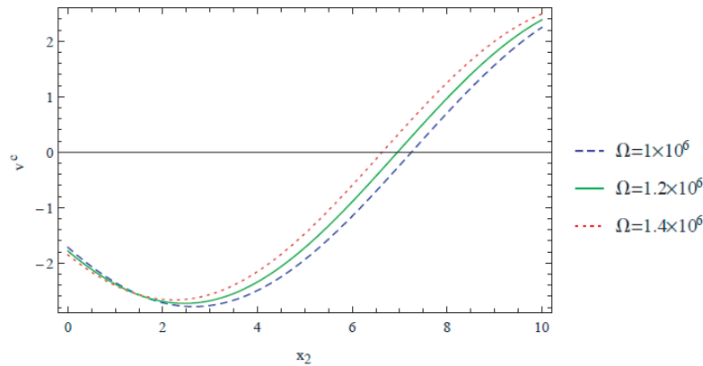
Figure 6. Variation of the displacement v^c in core layer given in Eq. (21) with variation of rotation.
