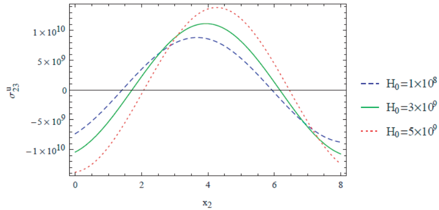
Figure 5. Variation of the shear stress \sigma_{23}^u in the upper skin layer given in Eq. (20) with variation of magnetic field.
