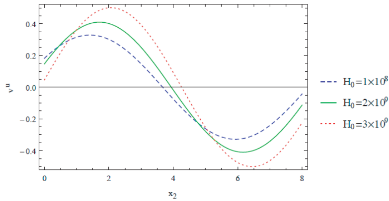
Figure 4. Variation of the displacement v^u in the upper skin layer given in Eq. (20) with variation of magnetic field.
