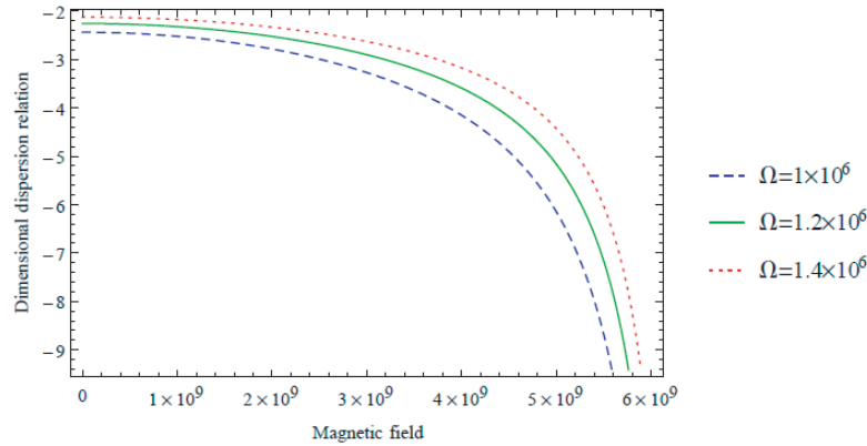
Figure 9. Variation of the general dispersion relation given in Eq. (27) with respect to the magnetic field with variation in rotation.
