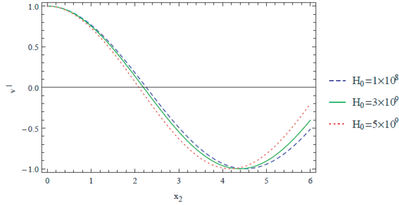
Figure 2. Variation of the displacement v^l in the lower skin layer given in Eq. (19) with variation of magnetic field.
