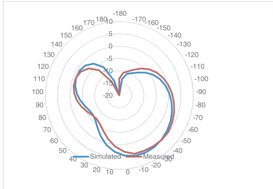
Figure 11. Measured radiation pattern of antenna 3.
