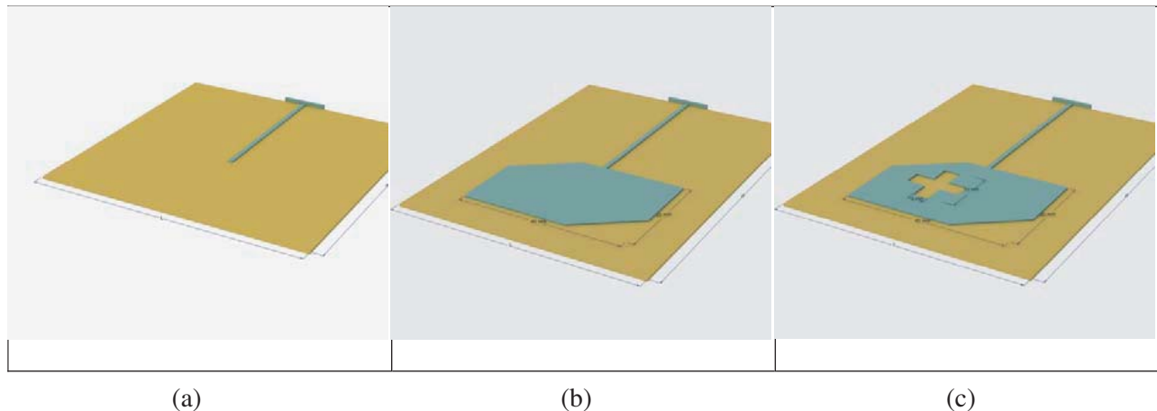
Figure 4. Development phases of the antenna structure. (a) Antenna 1. (b) Antenna 2. (c) Antenna 3.
