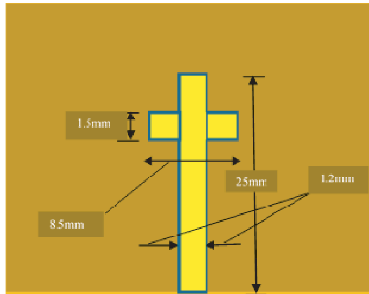
Figure 2. Aperture coupled feed (top view).
