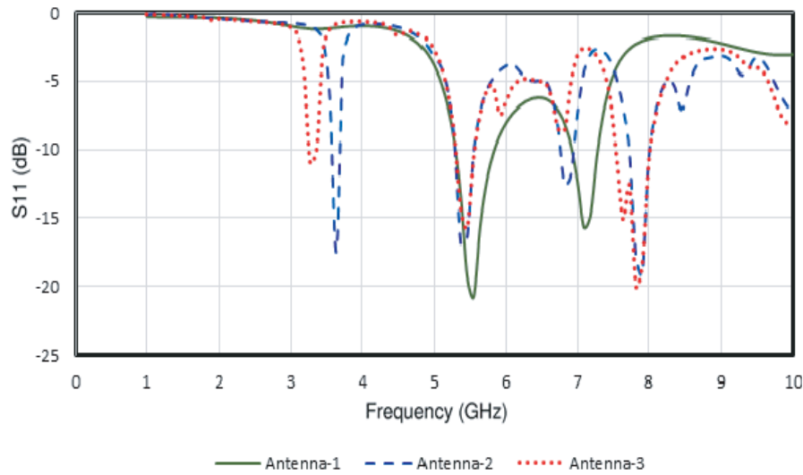
Figure 5. Reflection coefficient of antenna 1, antenna 2, antenna 3.
