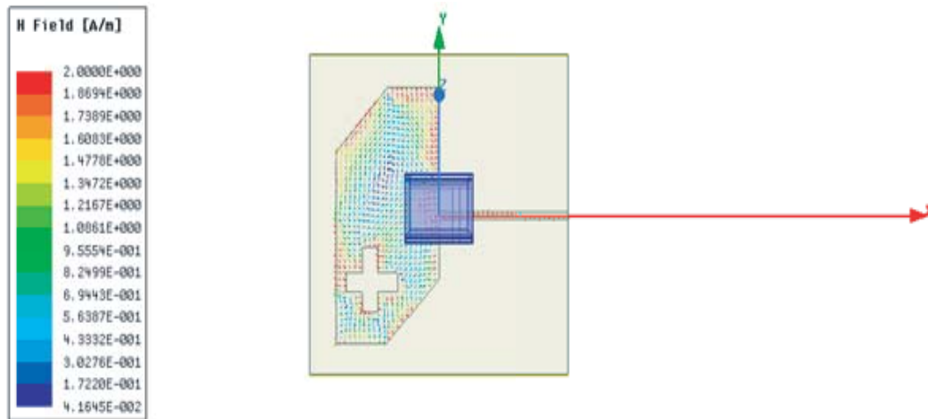
Figure 8. Circular polarization in antenna 3.
