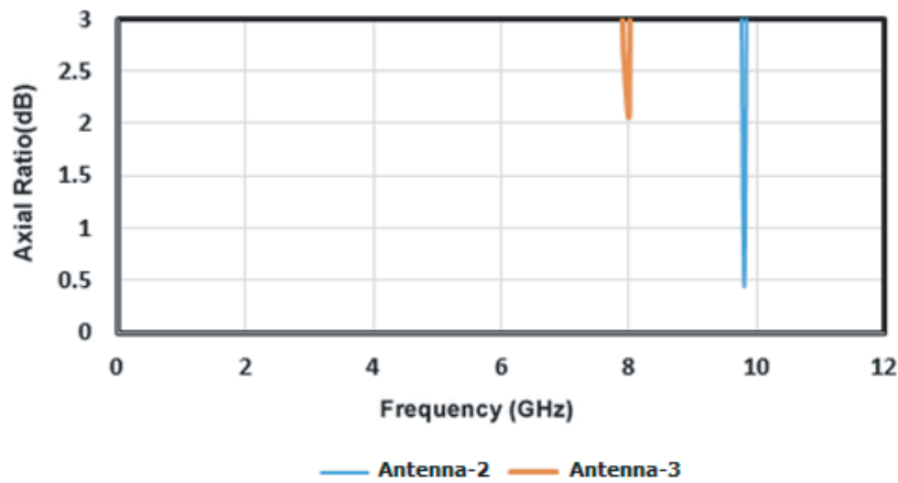
Figure 6. Axial ratio of antenna 2 and antenna 3.
