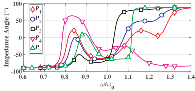
Figure 3. Impedance angle versus \omega/\omega_0 with different positions.
