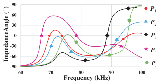
Figure 8. Measured impedance angle versus frequency with different positions.
