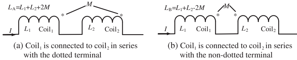
Figure 7. Measured mutual inductance model.
