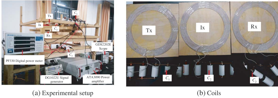
Figure 6. Experimental setup of the three-coil WPT system.
