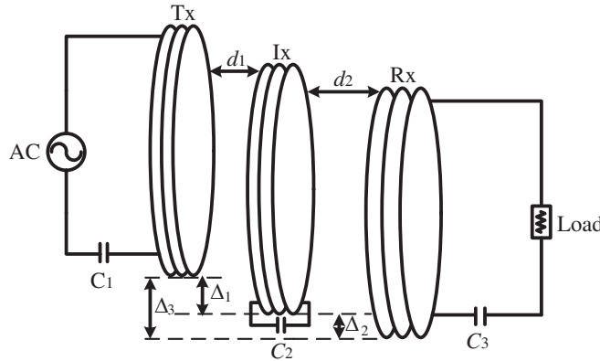
Figure 1. Diagram of three-coil WPT system.
