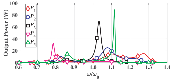
Figure 5. Output power versus \omega/\omega_0 with different positions.
