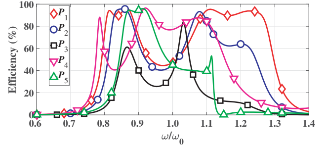
Figure 4. Efficiency versus \omega/\omega_0 with different positions.
