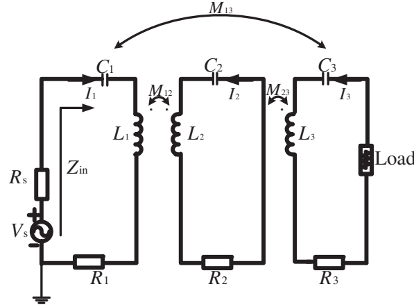
Figure 2. Equivalent circuit diagram of three-coil WPT system.
