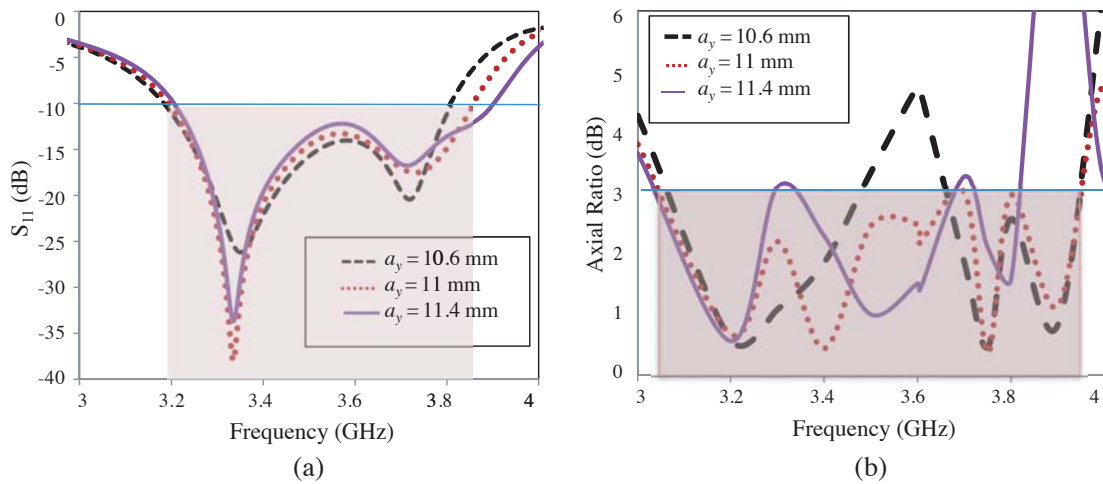
Figure 4. Parametric analysis by varying the DRA offset along y -direction. (a) S_{11} . (b) Axial Ratio.
