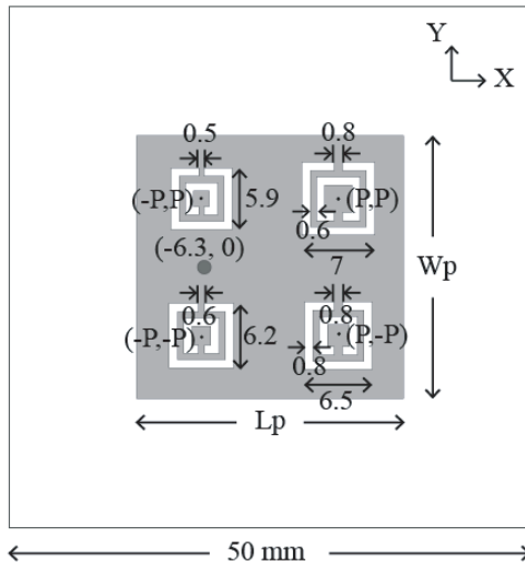
Figure 1. Geometry of the asymmetric CSRRs loaded CP antenna: L_p = 25.6 \text{ mm} , W_p = 25.2 \text{ mm} and P = 6.56 \text{ mm} .
