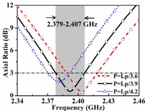
Figure 3. Axial ratio plot of the antenna for different positions of CSRRs.
