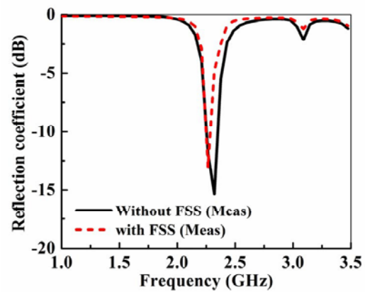
Figure 19. Measured reflection coefficient of the antenna with and without FSS.
